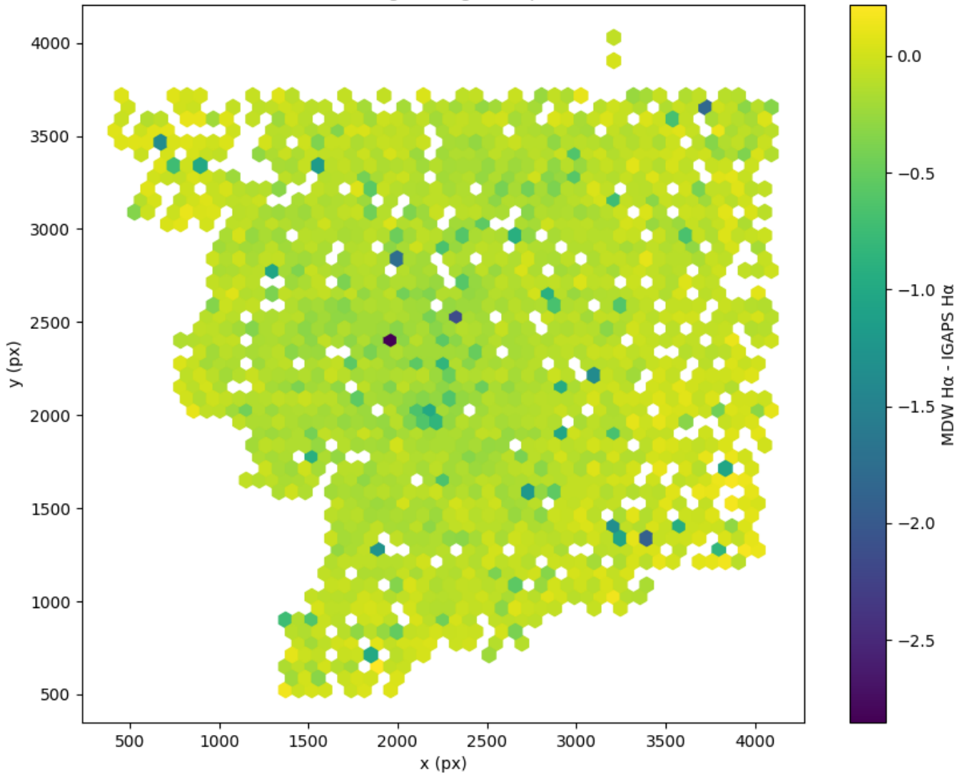
Field 2146 2D field distribution of MDW H \alpha - IGAPS H \alpha Hexagon length: 73px
