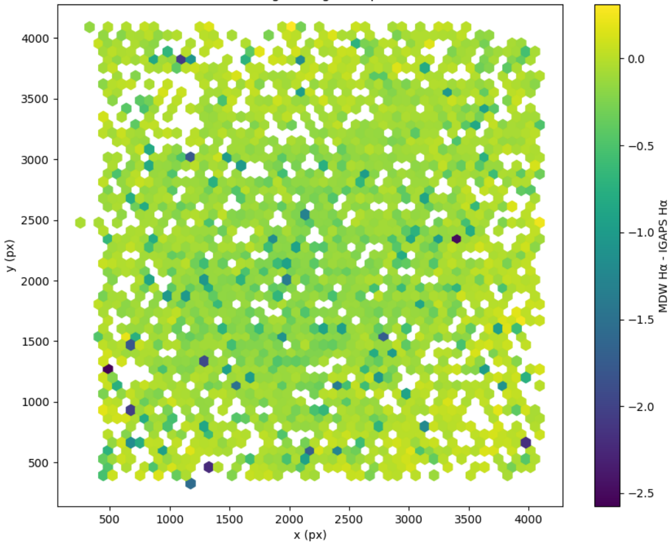
Field 0256 2D field distribution of MDW H \alpha - IGAPS H \alpha Hexagon length: 77px
