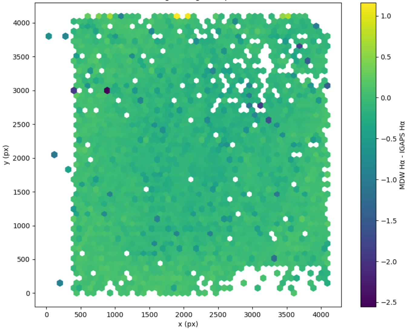
Field 0367 2D field distribution of MDW H \alpha - IGAPS H \alpha Hexagon length: 81px
