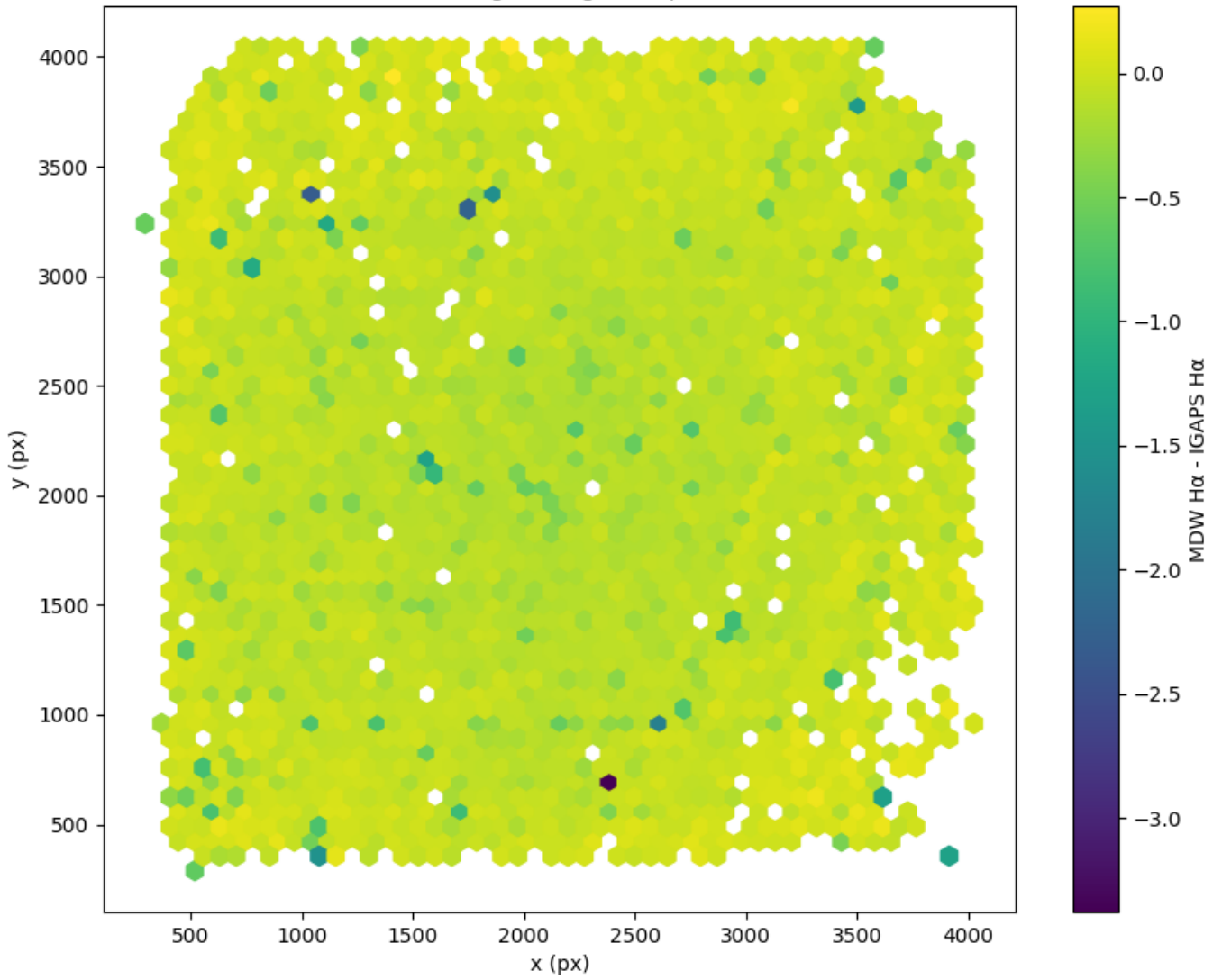
Field 0477 2D field distribution of MDW H \alpha - IGAPS H \alpha Hexagon length: 75px
