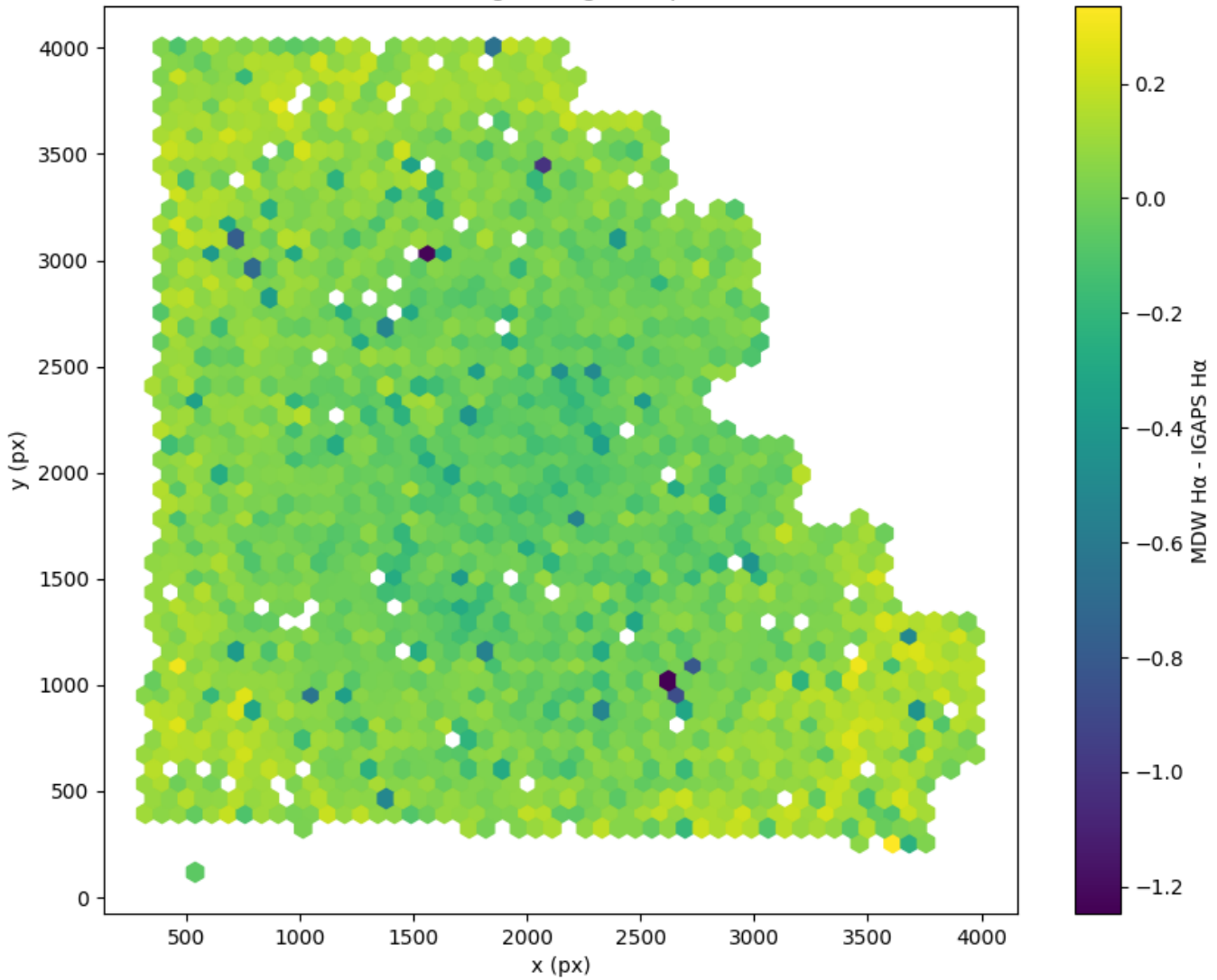
Field 0588 2D field distribution of MDW H \alpha - IGAPS H \alpha Hexagon length: 74px
