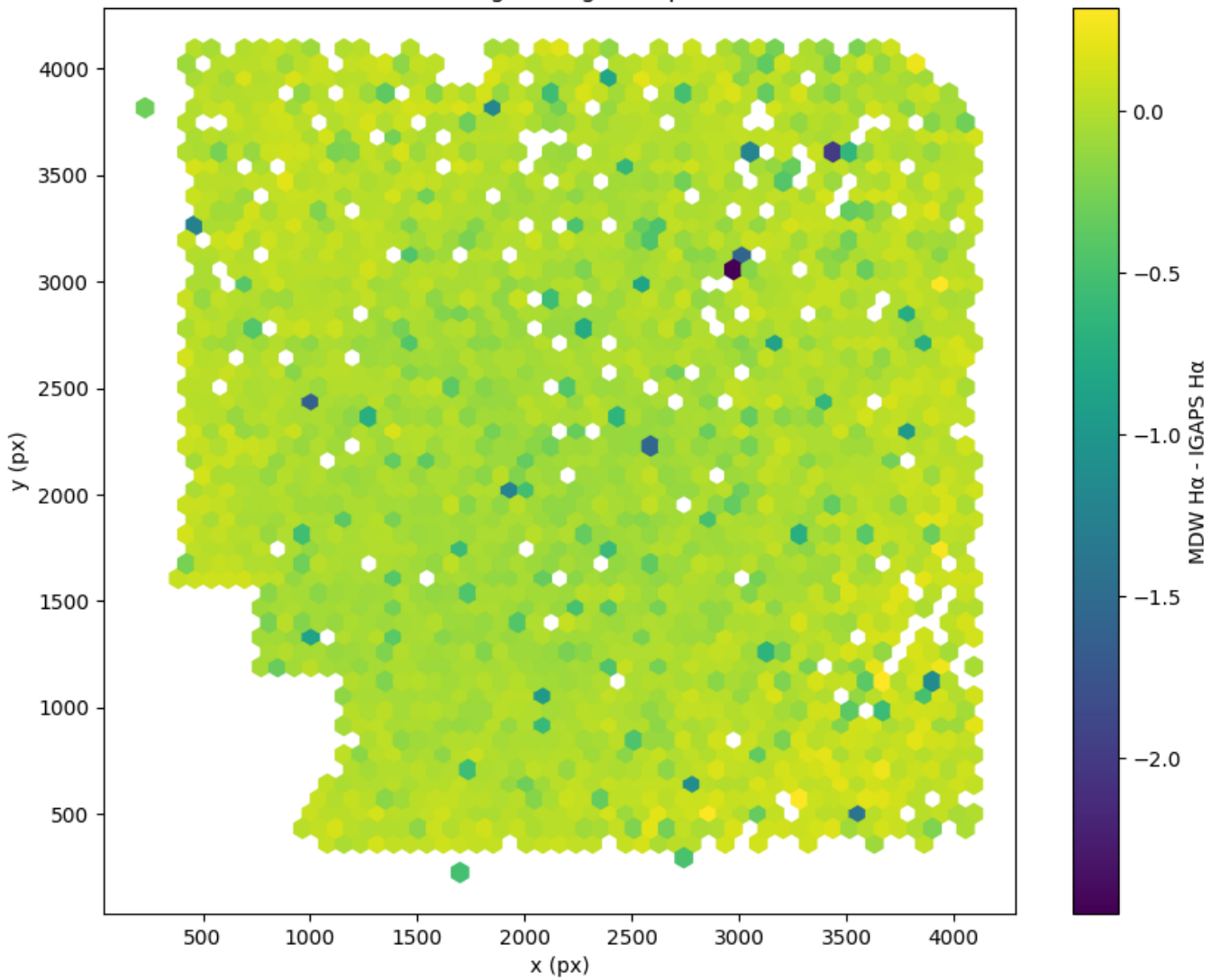
Field 0476 2D field distribution of MDW H \alpha - IGAPS H \alpha Hexagon length: 77px
