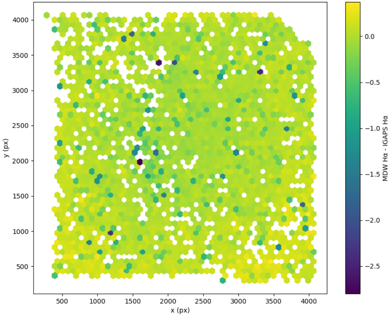
Field 0368 2D field distribution of MDW H \alpha - IGAPS H \alpha Hexagon length: 76px
