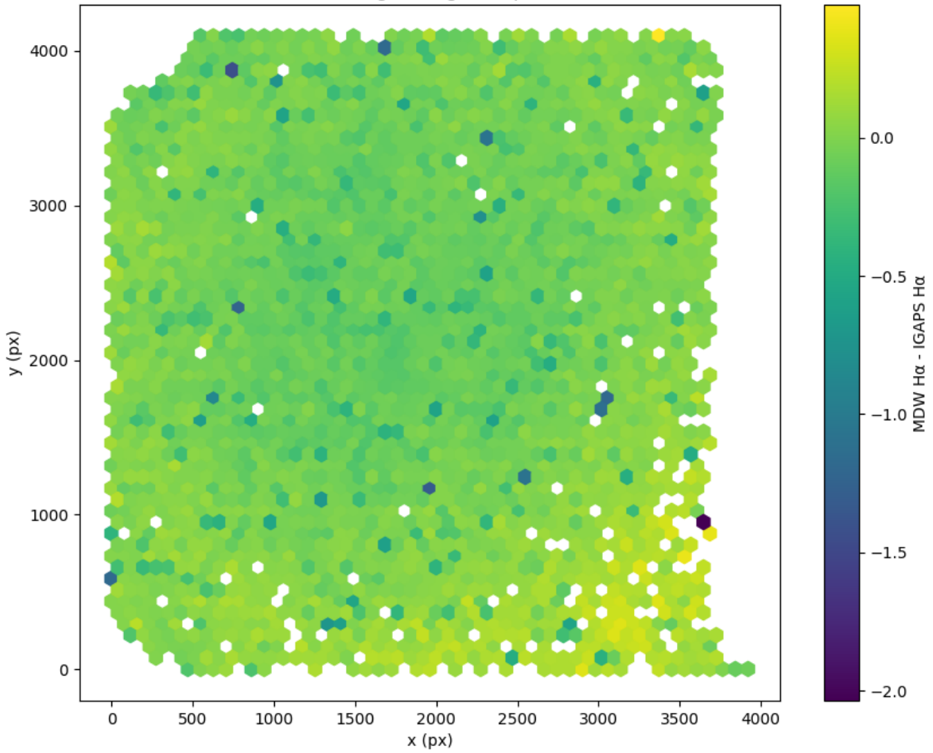
Field 0033 2D field distribution of MDW H \alpha - IGAPS H \alpha Hexagon length: 78px
