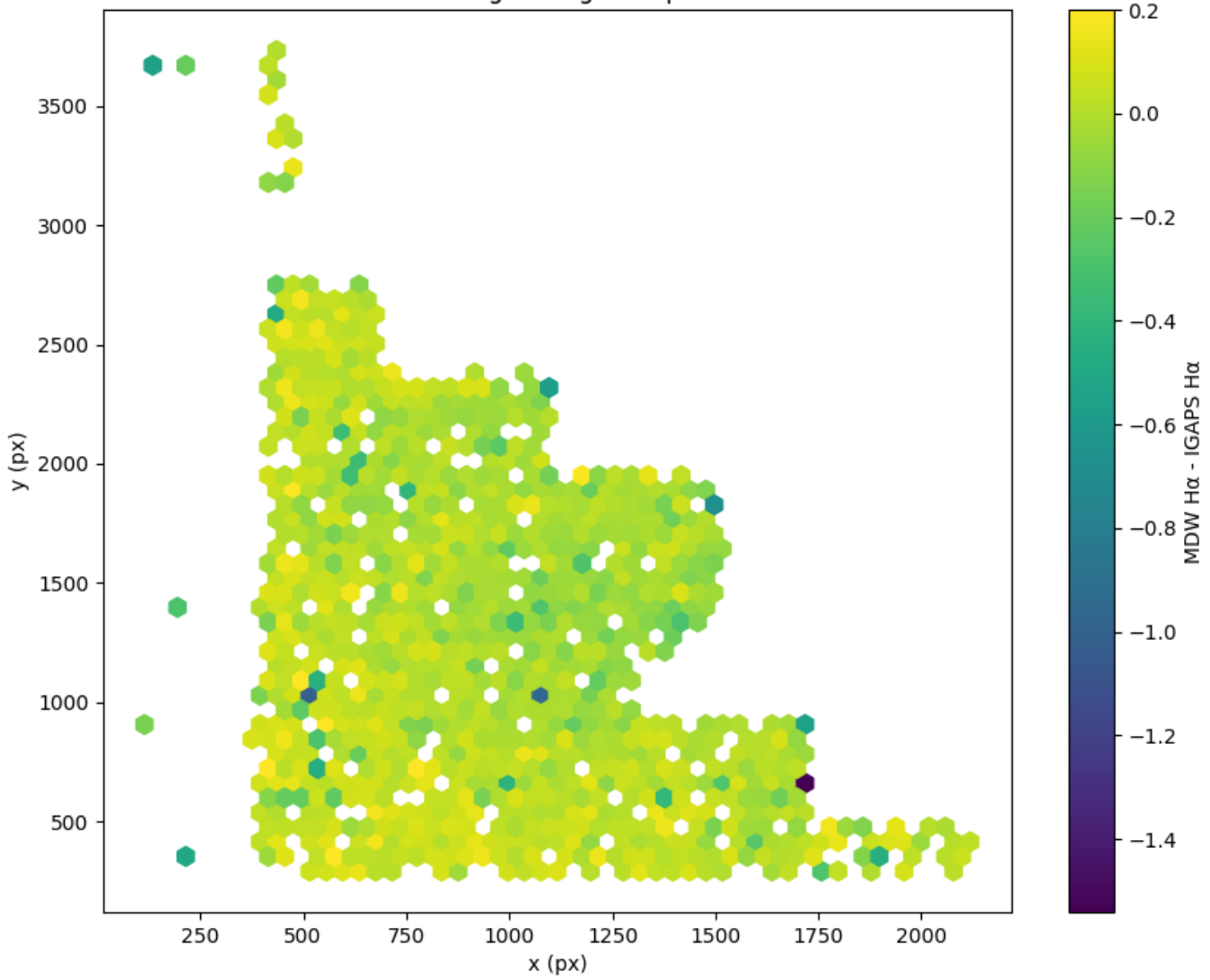
Field 0258 2D field distribution of MDW H \alpha - IGAPS H \alpha Hexagon length: 40px
