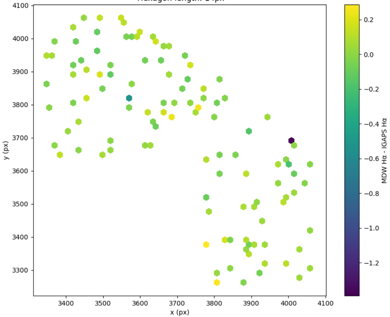
Field 0142 2D field distribution of MDW H \alpha - IGAPS H \alpha Hexagon length: 14px
