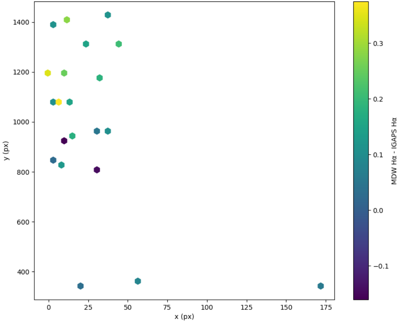
Field 0697 2D field distribution of MDW H \alpha - IGAPS H \alpha Hexagon length: 3px
