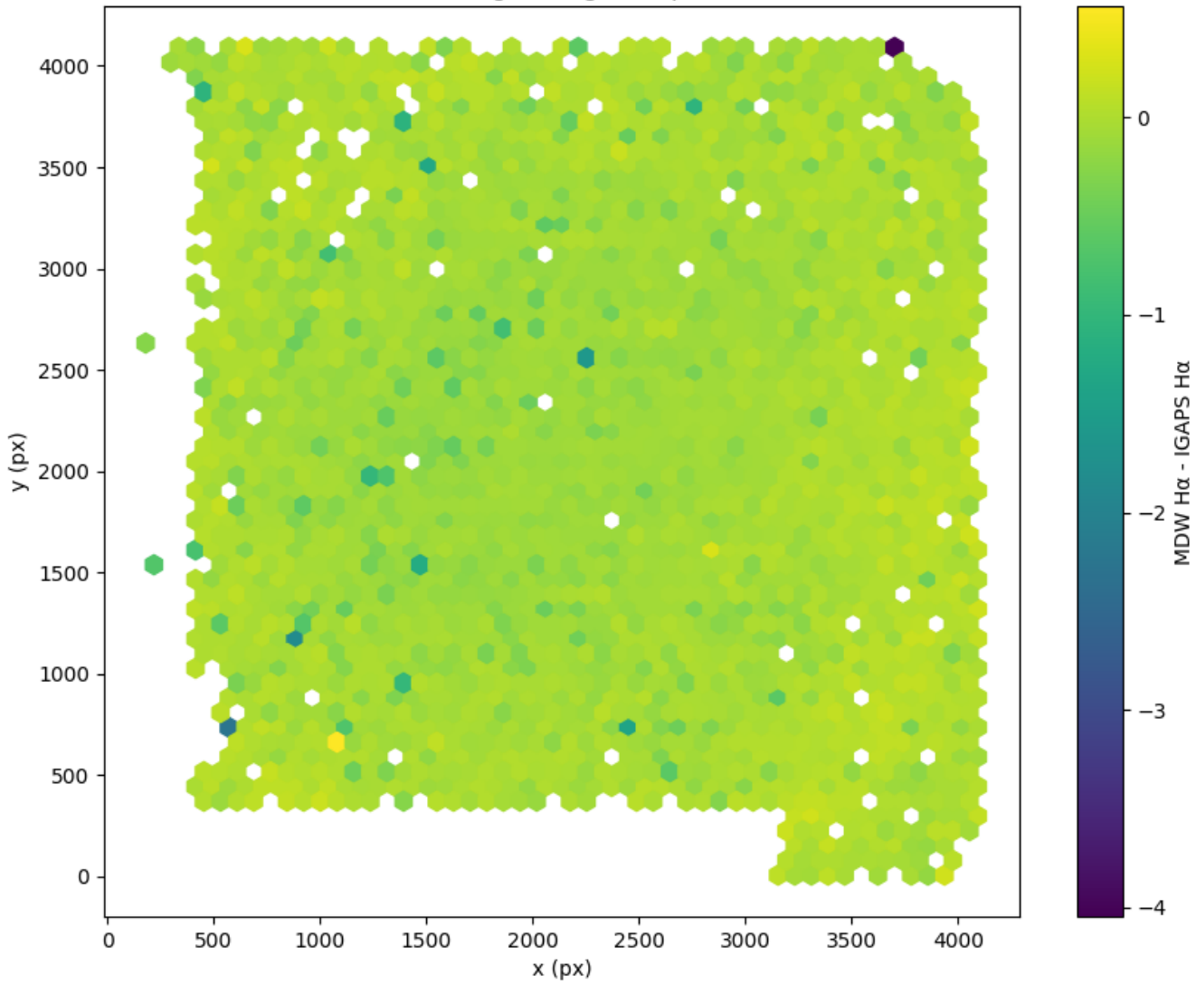
Field 0366 2D field distribution of MDW H \alpha - IGAPS H \alpha Hexagon length: 78px
