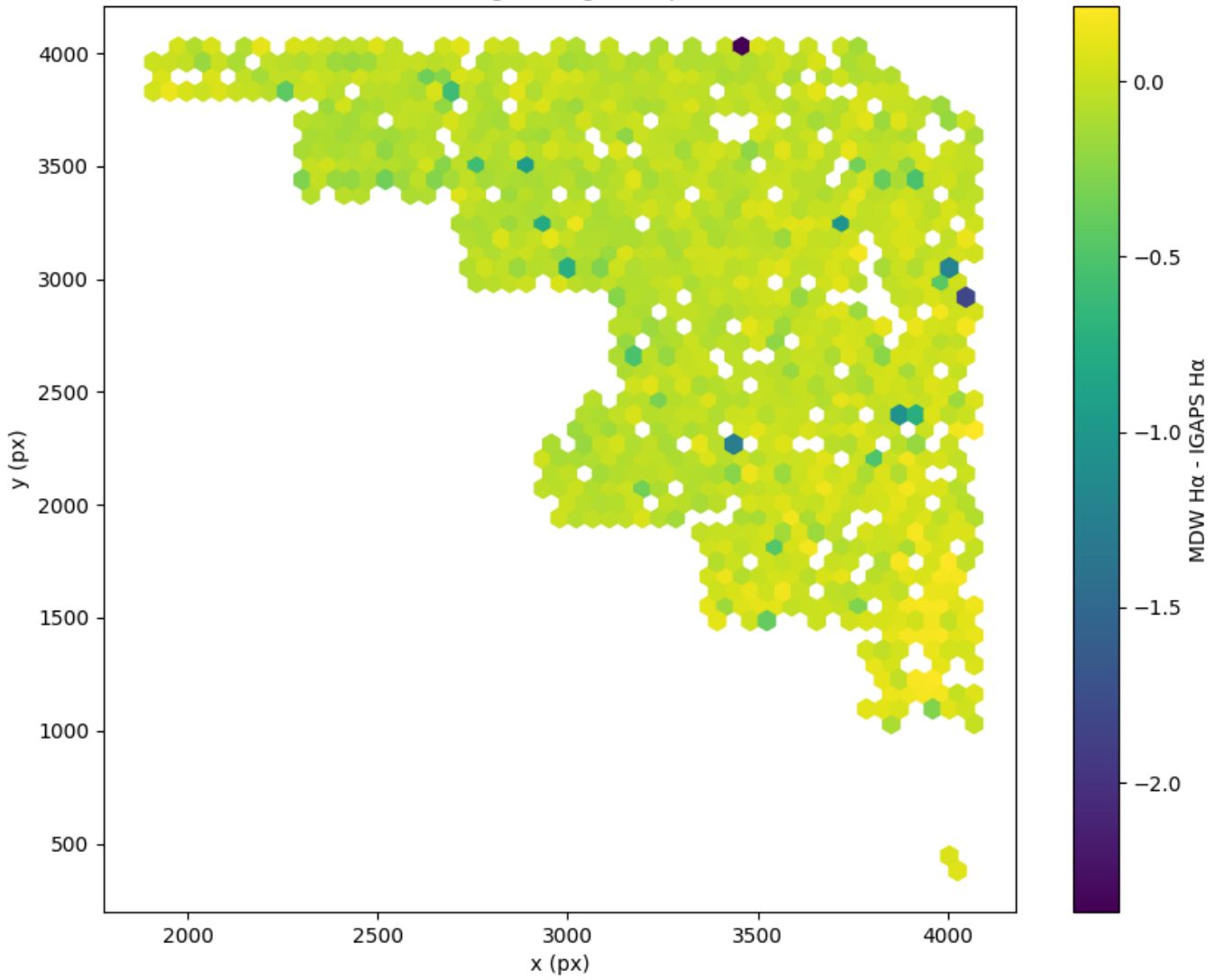
Field 0365 2D field distribution of MDW H \alpha - IGAPS H \alpha Hexagon length: 44px
