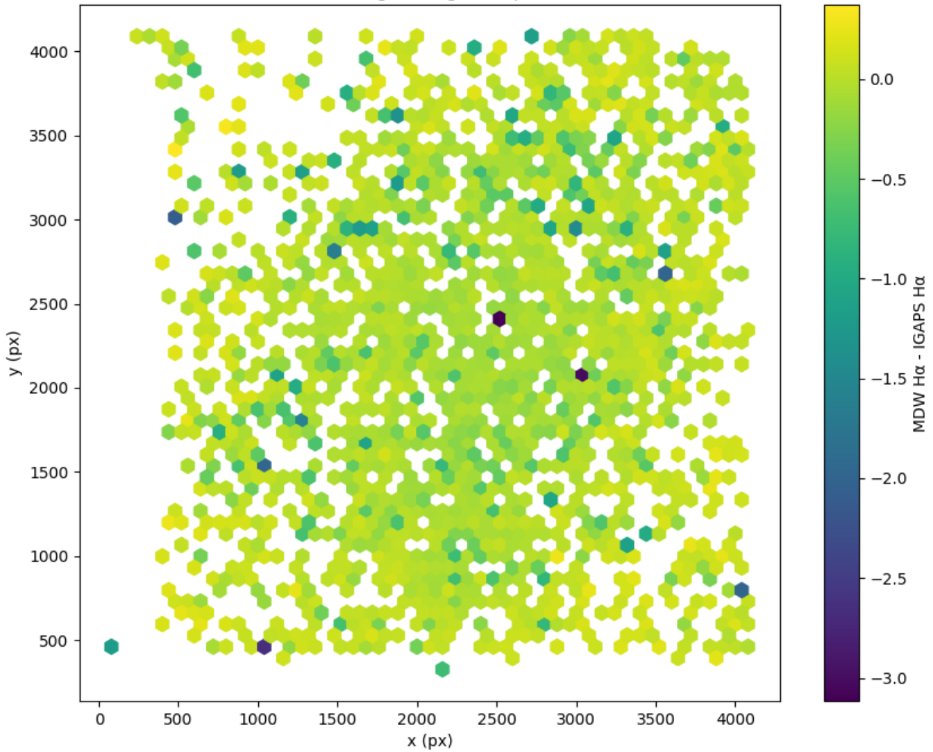
Field 0144 2D field distribution of MDW H \alpha - IGAPS H \alpha Hexagon length: 80px
