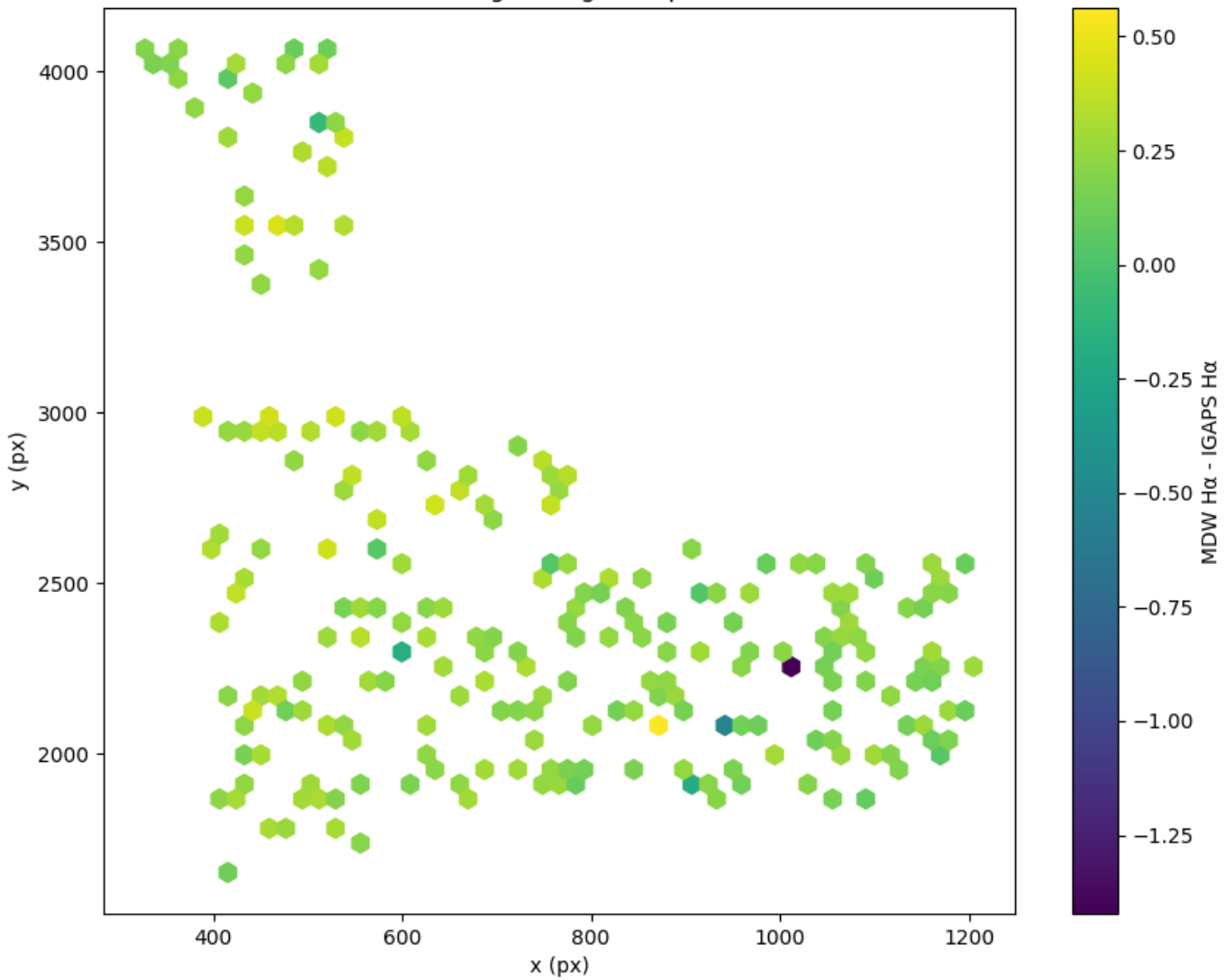
Field 0035 2D field distribution of MDW H \alpha - IGAPS H \alpha Hexagon length: 18px
