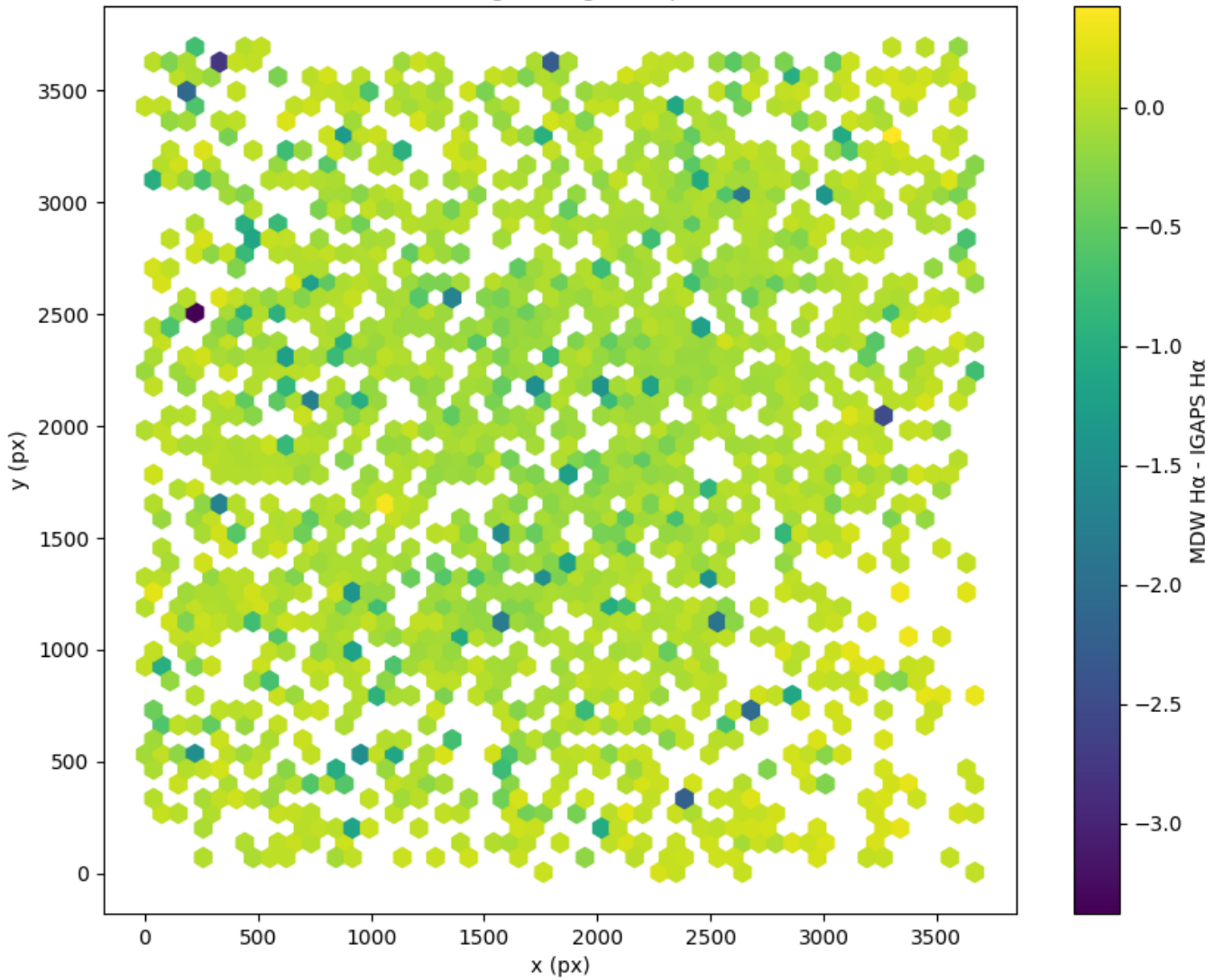
Field 0255 2D field distribution of MDW H \alpha - IGAPS H \alpha Hexagon length: 73px
