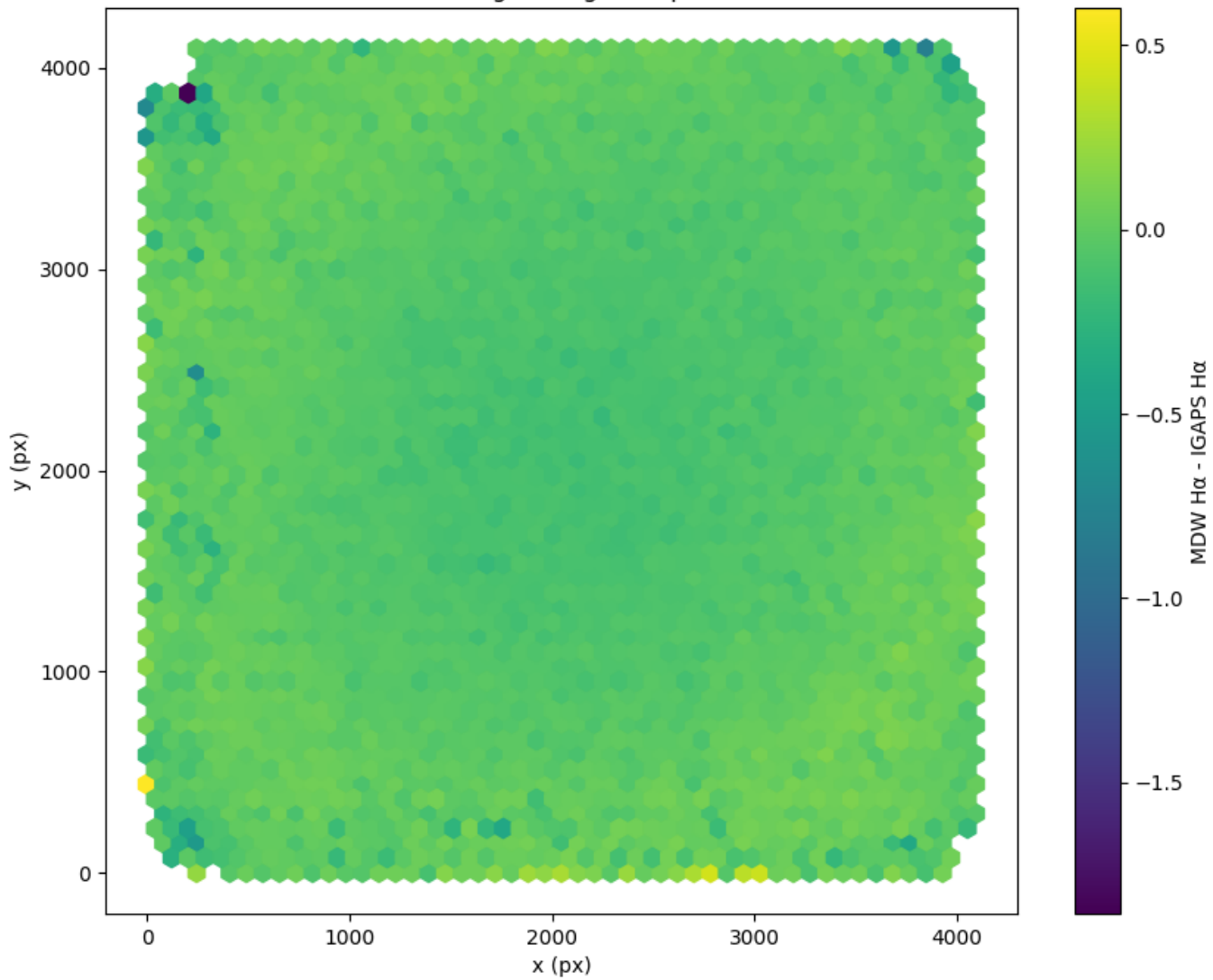
Across all fields 2D field distribution of MDW H \alpha - IGAPS H \alpha Hexagon length: 82px
