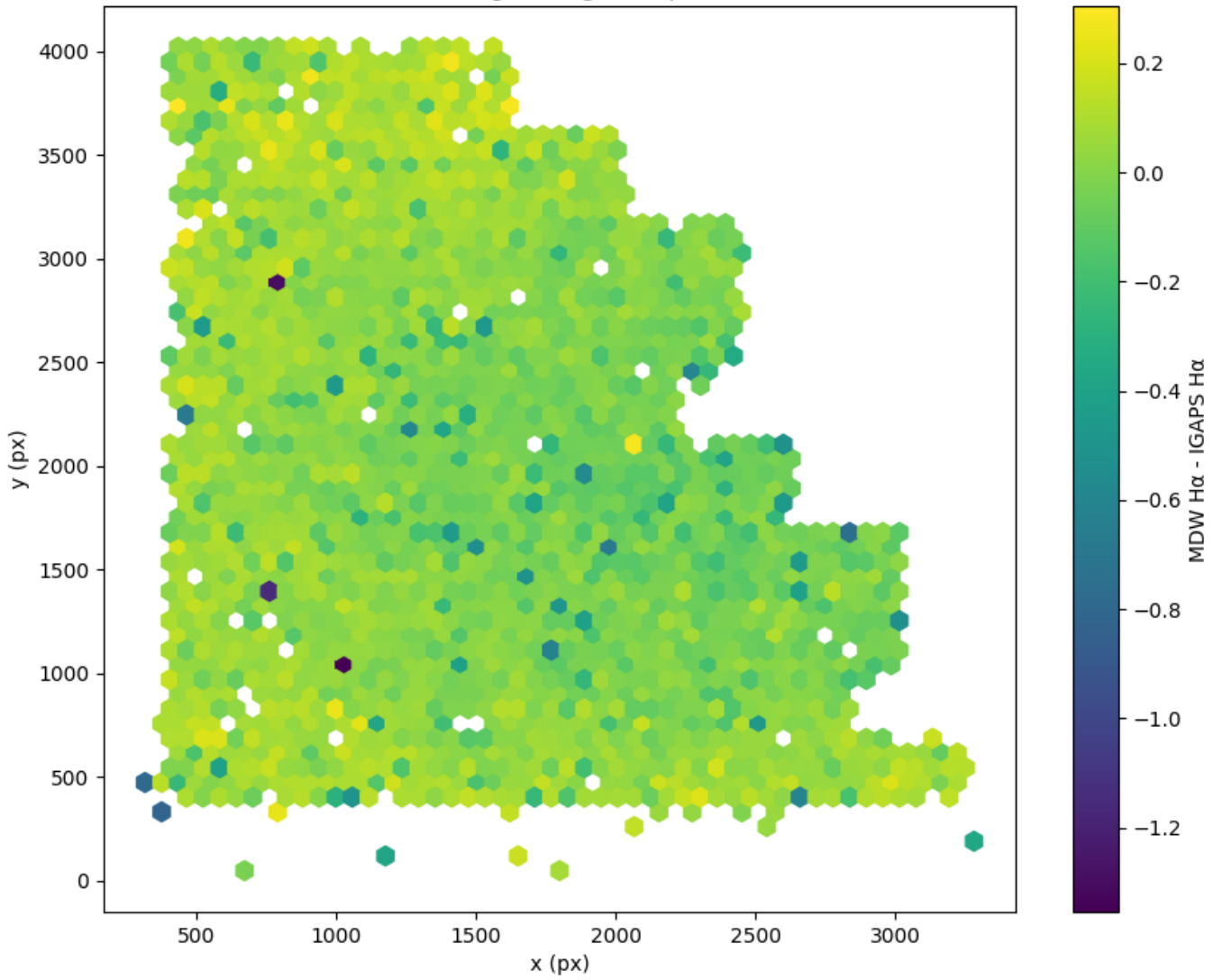
Field 0479 2D field distribution of MDW H \alpha - IGAPS H \alpha Hexagon length: 59px
