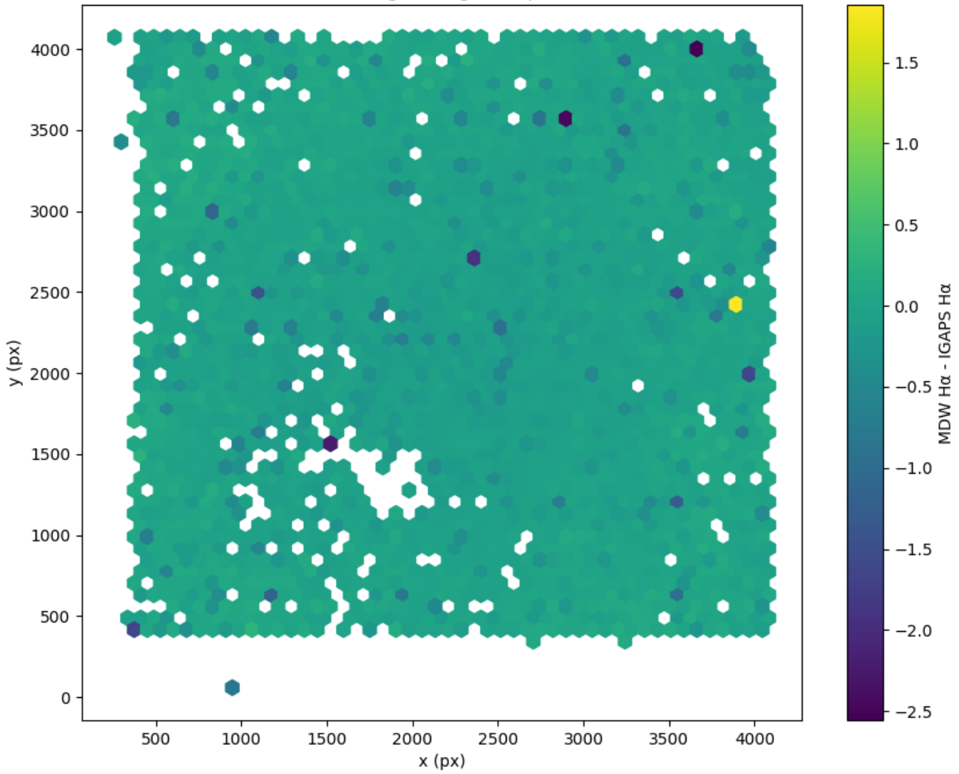
Field 0478 2D field distribution of MDW H \alpha - IGAPS H \alpha Hexagon length: 76px
