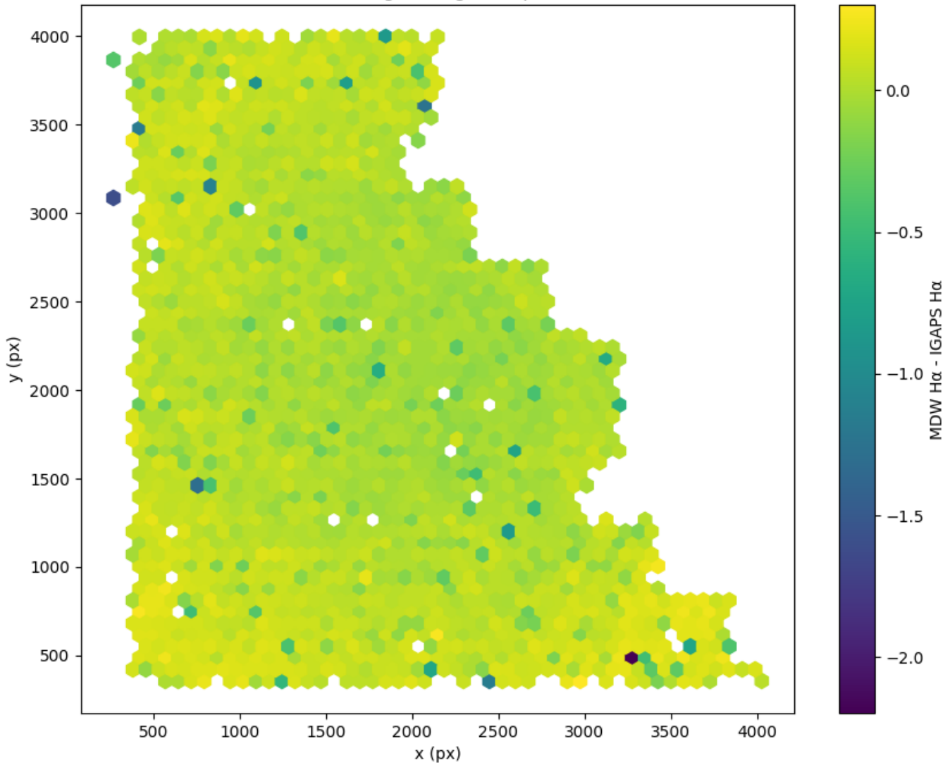
Field 0146 2D field distribution of MDW H \alpha - IGAPS H \alpha Hexagon length: 80px
