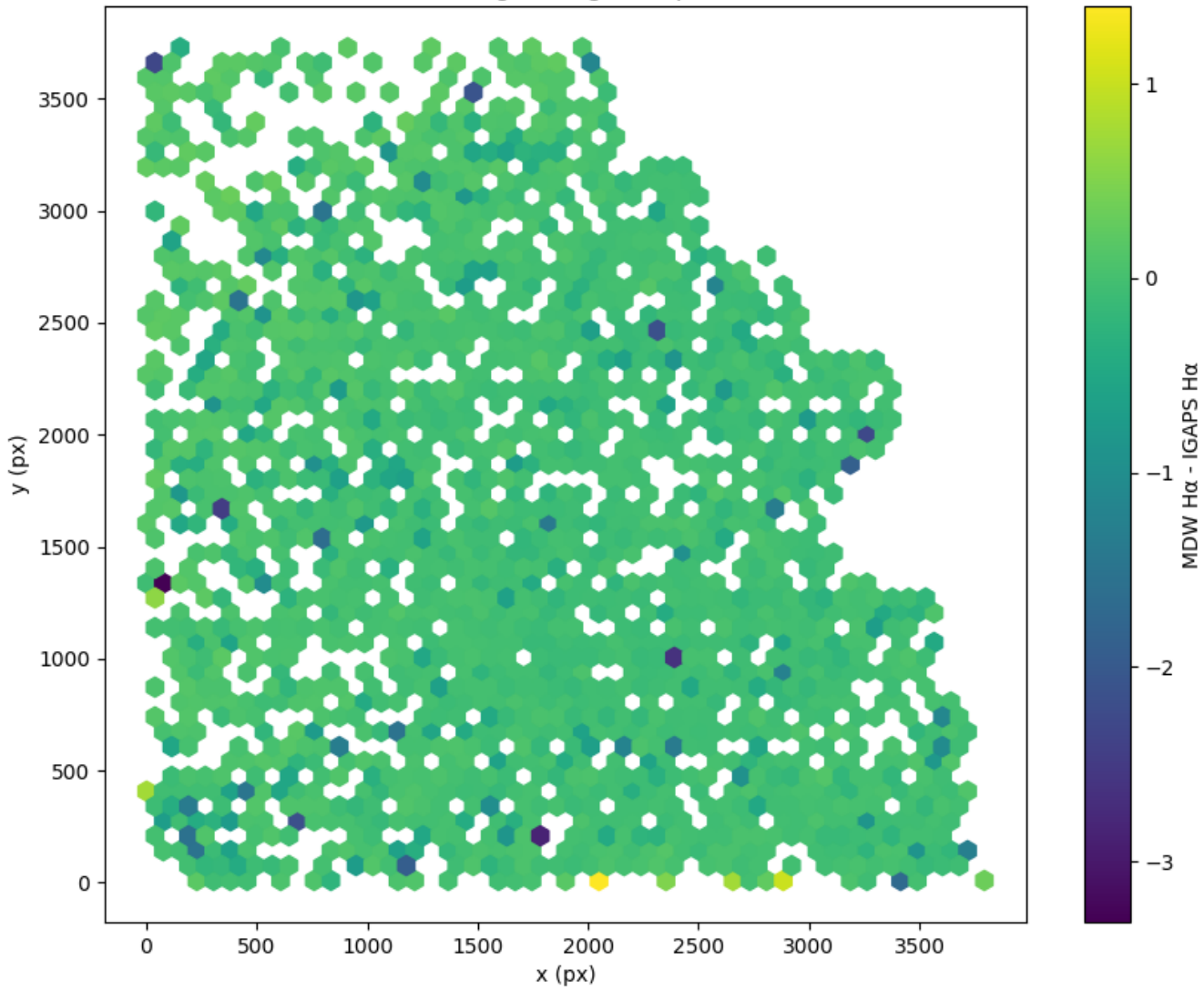
Field 0143 2D field distribution of MDW H \alpha - IGAPS H \alpha Hexagon length: 76px
