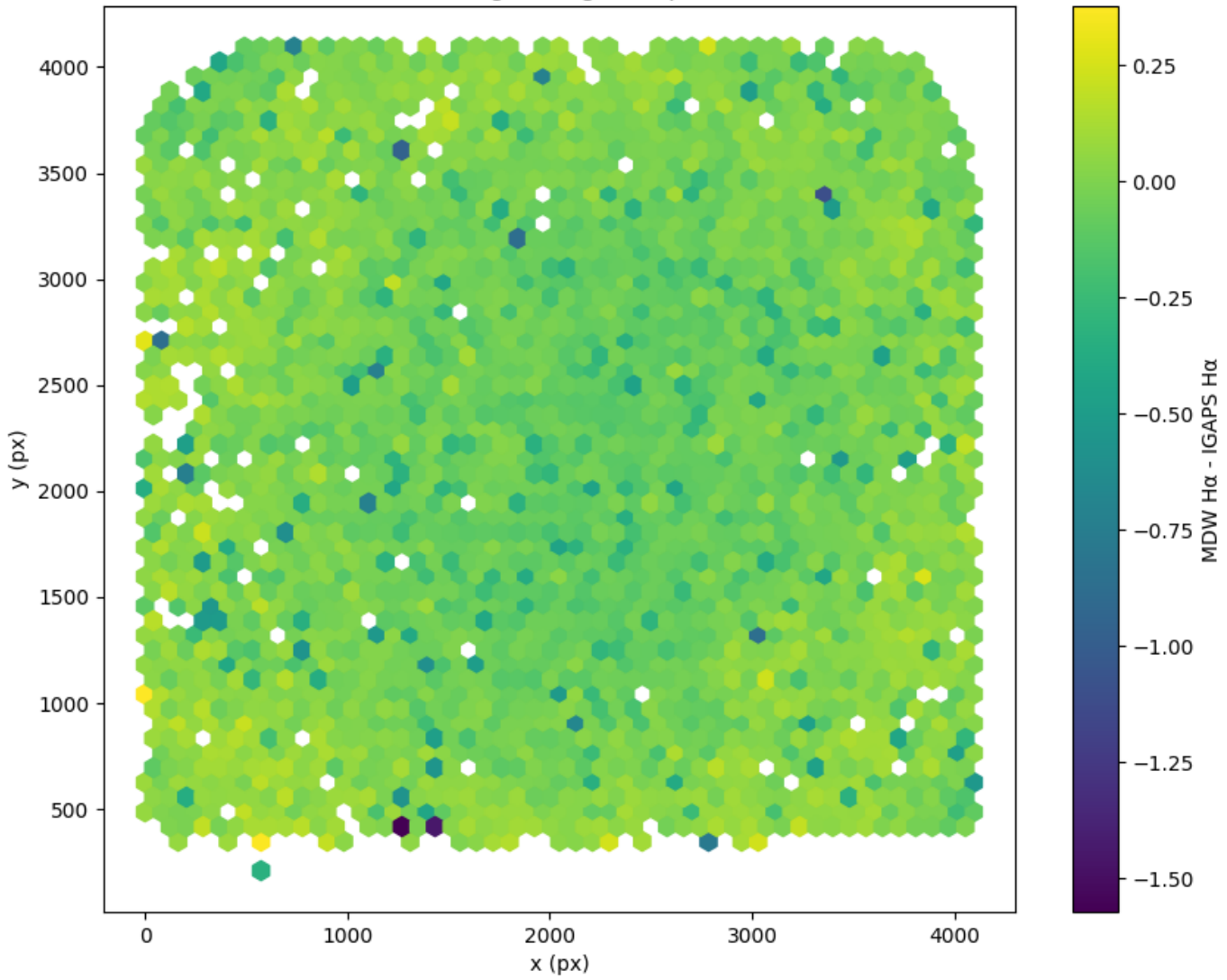
Field 0587 2D field distribution of MDW H \alpha - IGAPS H \alpha Hexagon length: 82px
