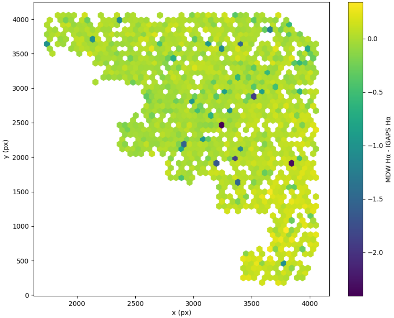
Field 0031 2D field distribution of MDW H \alpha - IGAPS H \alpha Hexagon length: 46px
