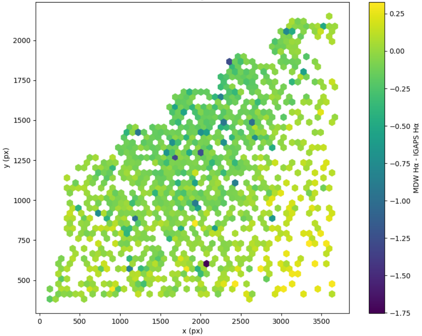
Field 2147 2D field distribution of MDW H \alpha - IGAPS H \alpha Hexagon length: 71px
