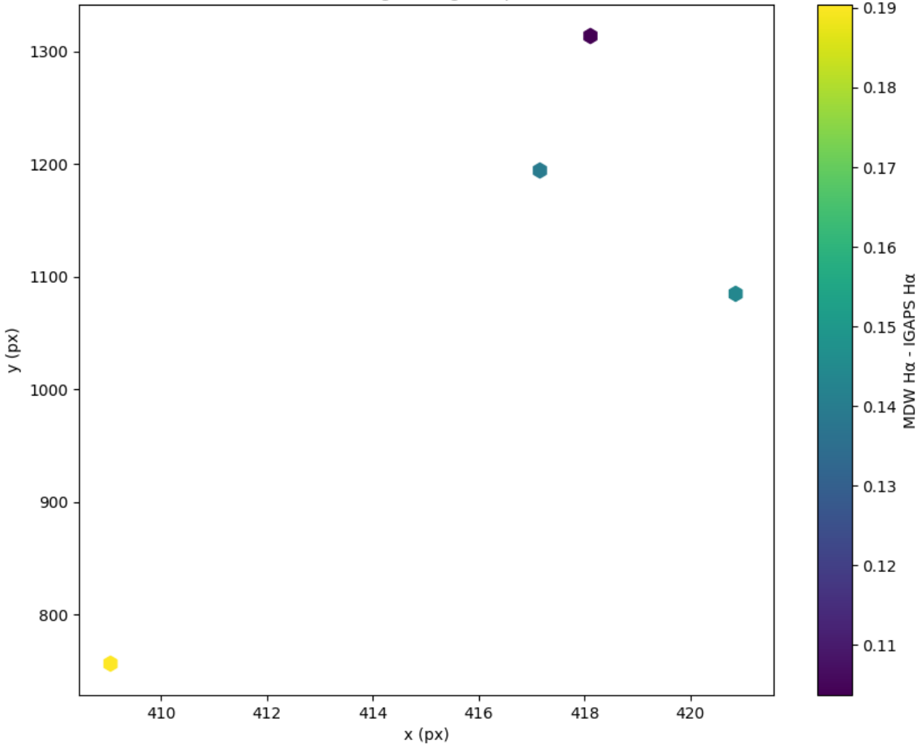
Field 0589 2D field distribution of MDW H \alpha - IGAPS H \alpha Hexagon length: 0px
