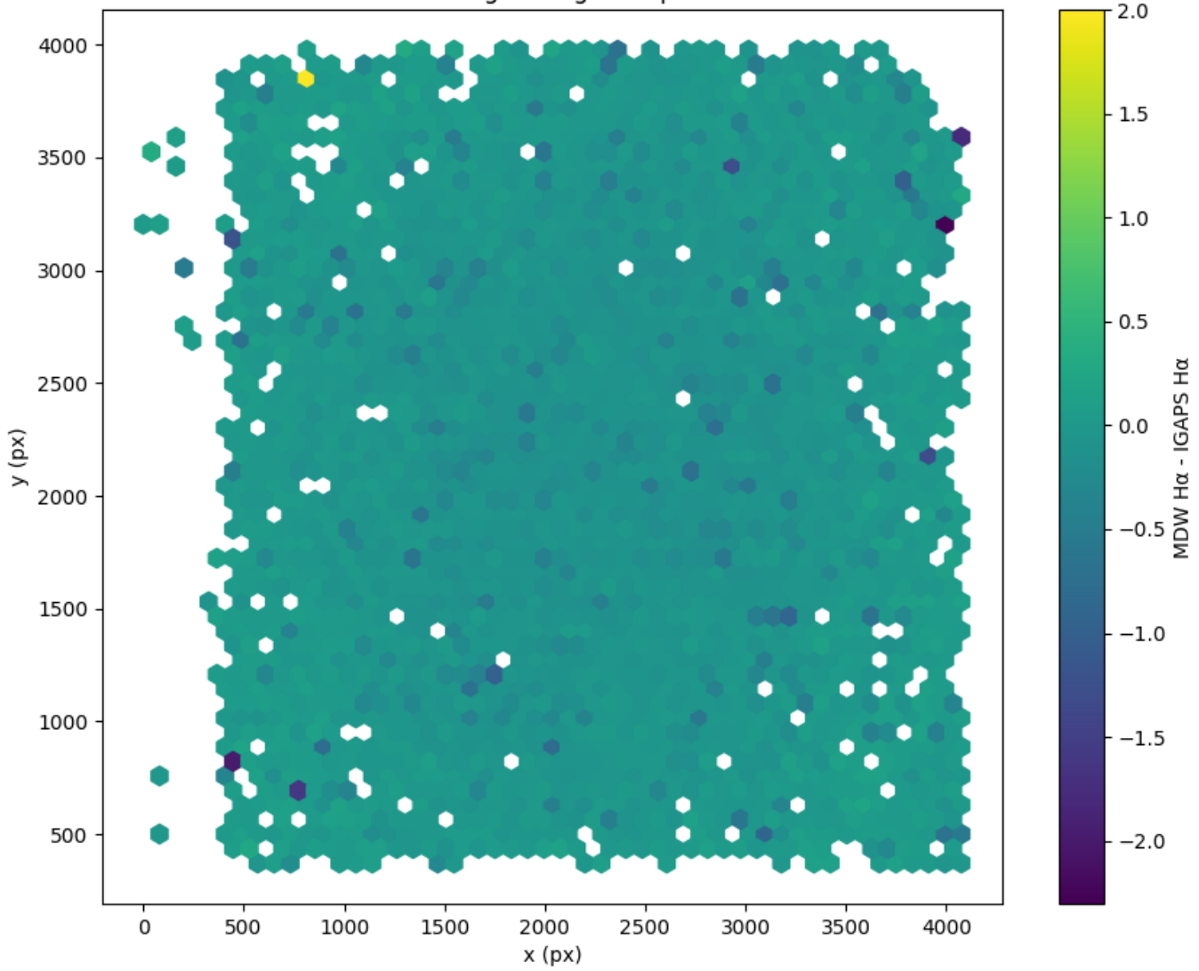
Field 0257 2D field distribution of MDW H \alpha - IGAPS H \alpha Hexagon length: 82px
