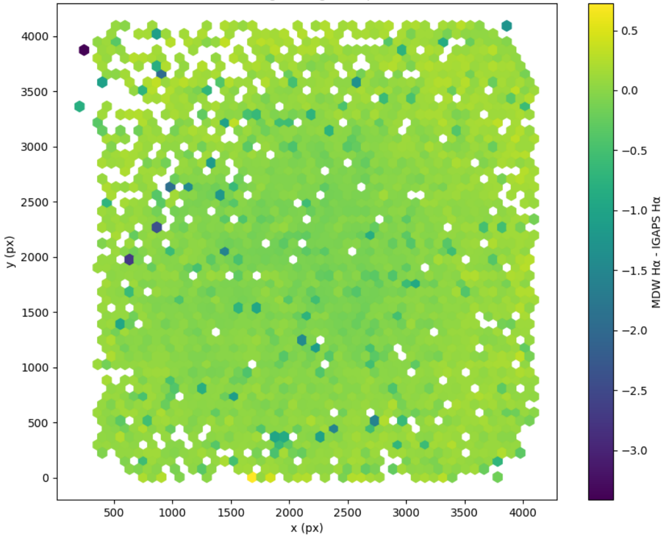
Field 0032 2D field distribution of MDW H \alpha - IGAPS H \alpha Hexagon length: 78px
