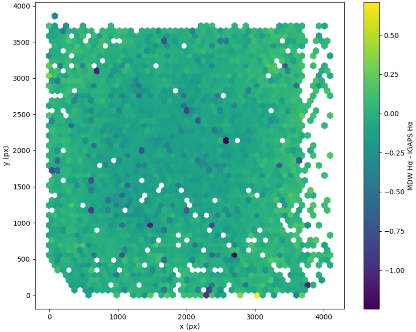
Field 0145 2D field distribution of MDW H \alpha - IGAPS H \alpha Hexagon length: 82px
