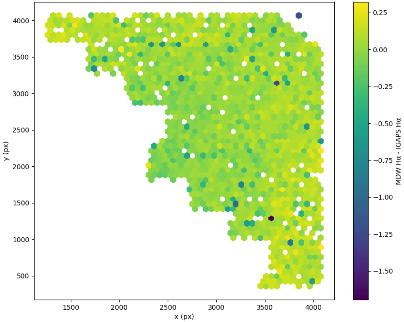
Field 0254 2D field distribution of MDW H \alpha - IGAPS H \alpha Hexagon length: 56px
