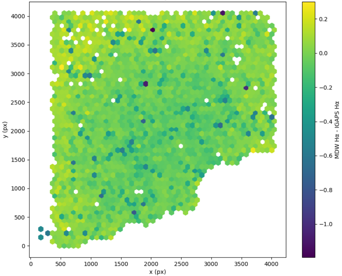
Field 0034 2D field distribution of MDW H \alpha - IGAPS H \alpha Hexagon length: 77px
