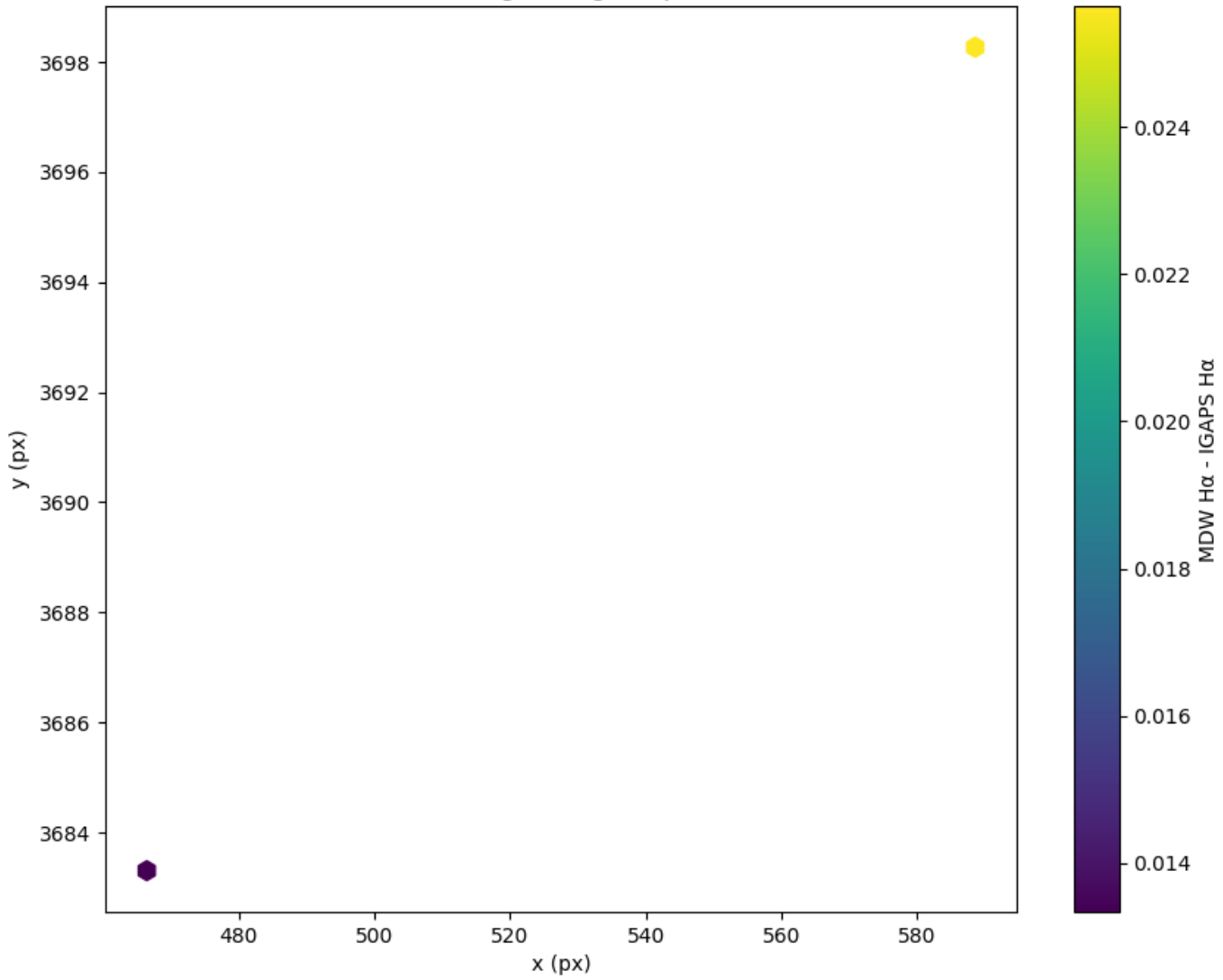
Field 2148 2D field distribution of MDW H \alpha - IGAPS H \alpha Hexagon length: 2px
