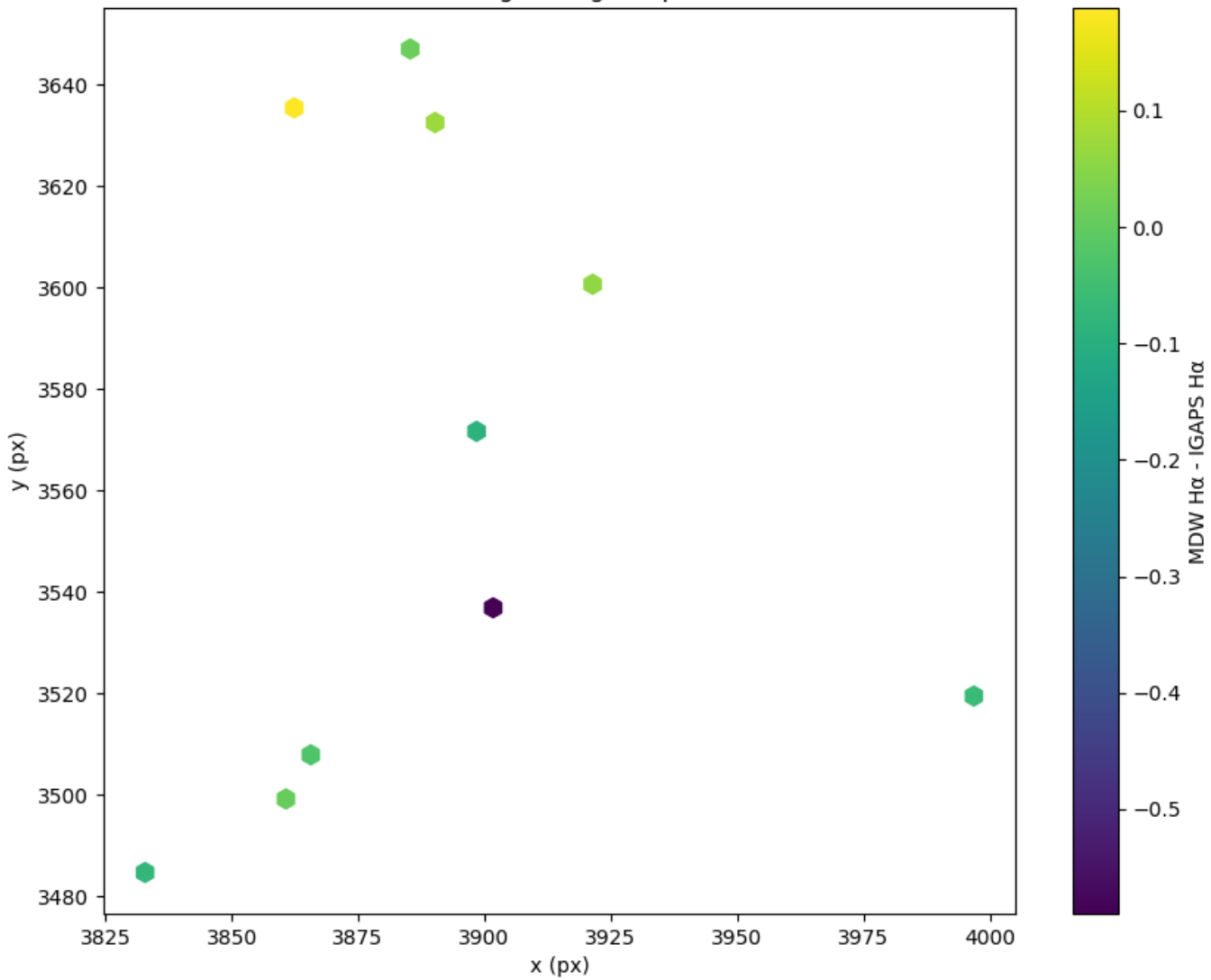
Field 2145 2D field distribution of MDW H \alpha - IGAPS H \alpha Hexagon length: 3px
