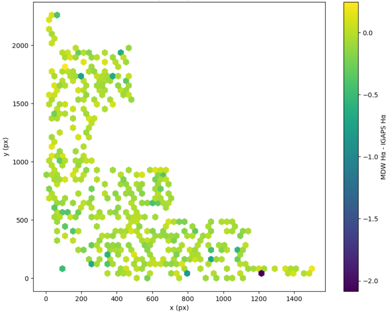
Field 0475 2D field distribution of MDW H \alpha - IGAPS H \alpha Hexagon length: 30px
