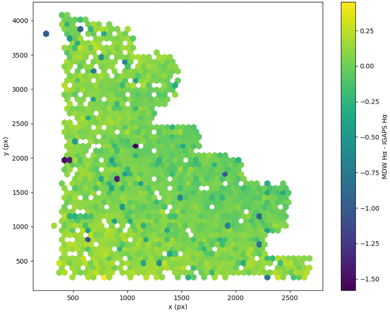
Field 0369 2D field distribution of MDW H \alpha - IGAPS H \alpha Hexagon length: 49px
