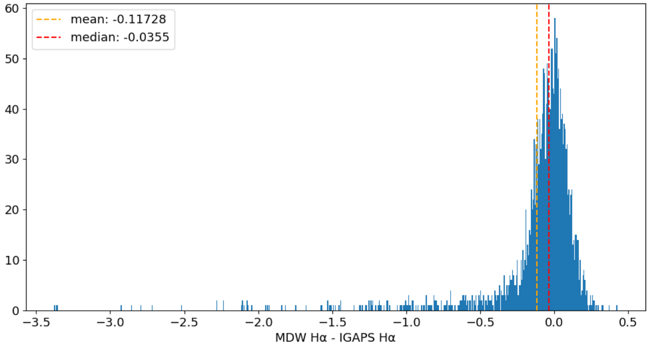
Field 0255 MDW H \alpha - IGAPS H \alpha 600 bins
