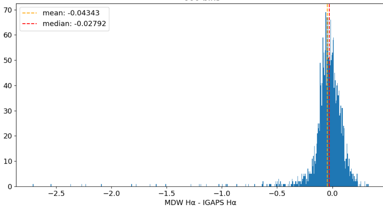
Field 0365 MDW H \alpha - IGAPS H \alpha 600 bins
