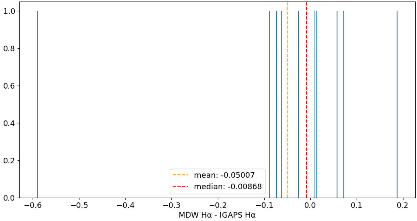
Field 2145 MDW H \alpha - IGAPS H \alpha 600 bins
