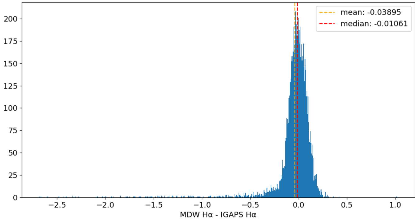
Field 0476 MDW H \alpha - IGAPS H \alpha 600 bins
