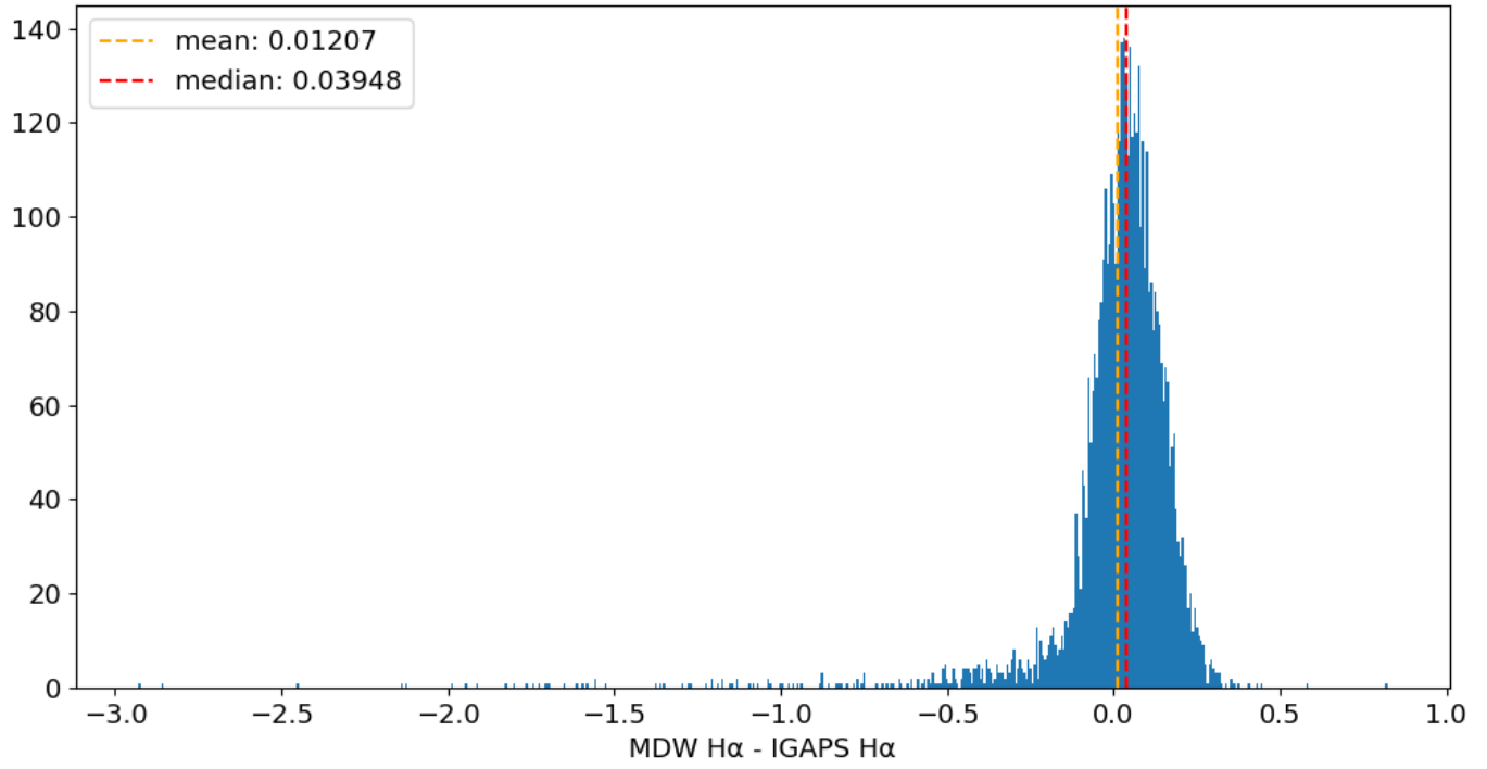
Field 0254 MDW H \alpha - IGAPS H \alpha 600 bins
