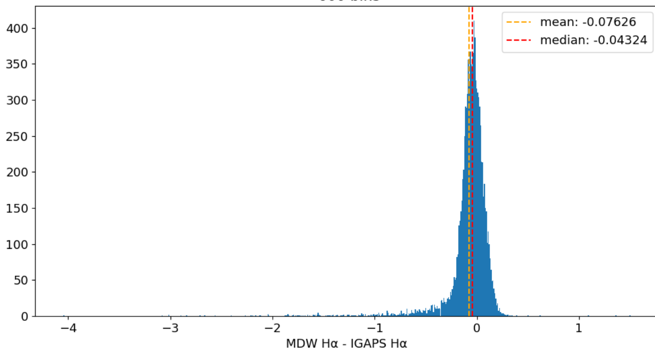
Field 0366 MDW H \alpha - IGAPS H \alpha 600 bins
