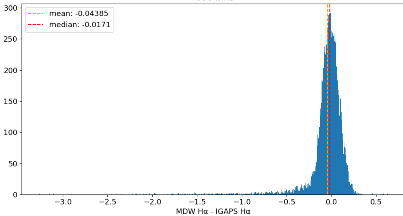
Field 0587 MDW H \alpha - IGAPS H \alpha 600 bins
