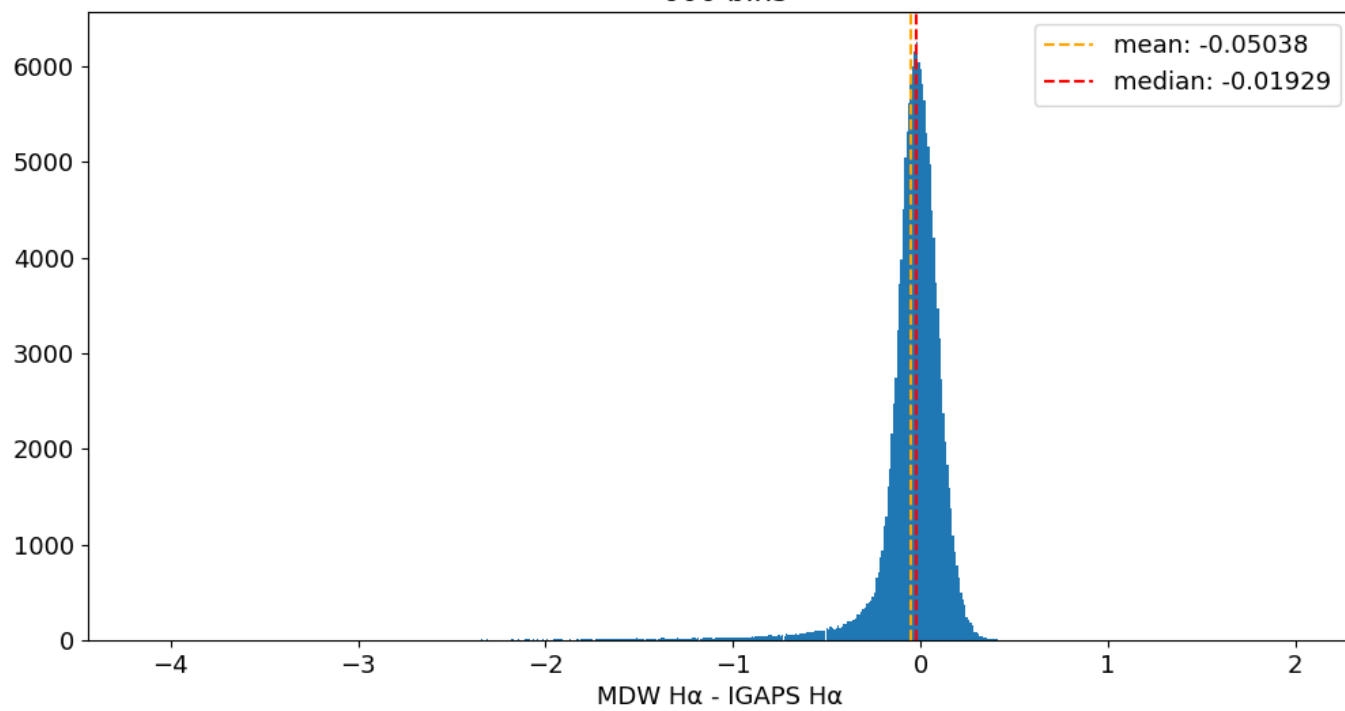
All fields (overlapping with IGAPS) MDW H \alpha - IGAPS H \alpha 600 bins
