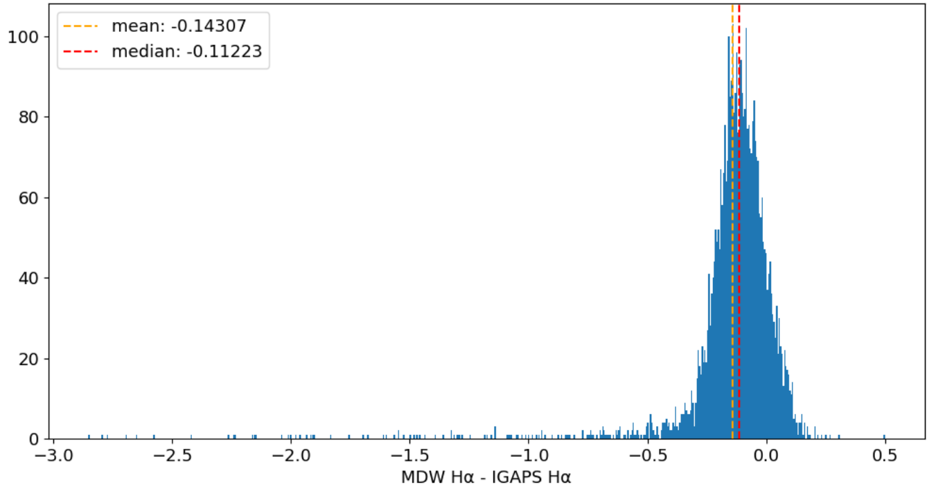
Field 2146 MDW H \alpha - IGAPS H \alpha 600 bins
