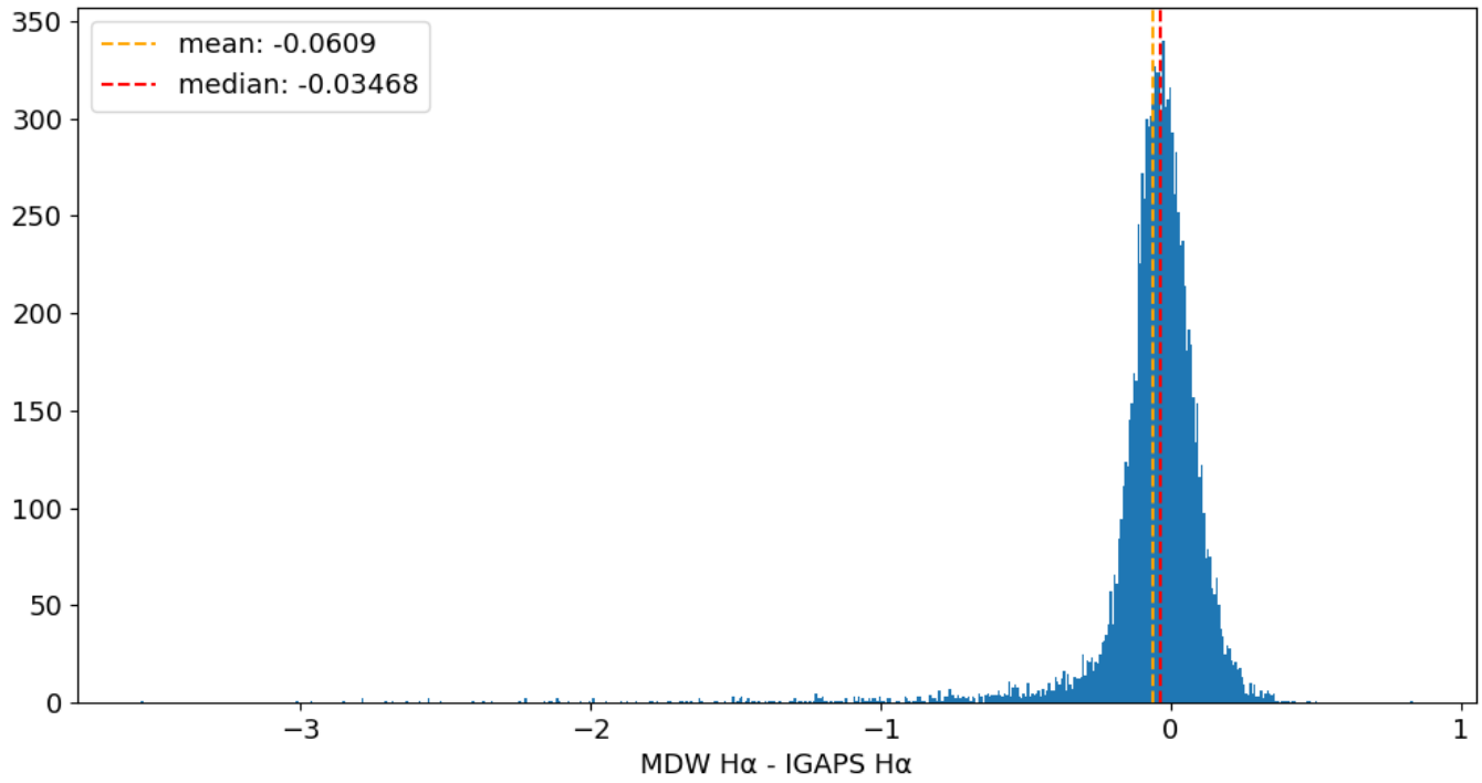
Field 0033 MDW H \alpha - IGAPS H \alpha 600 bins
