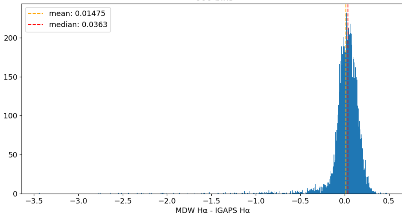
Field 0146 MDW H \alpha - IGAPS H \alpha 600 bins
