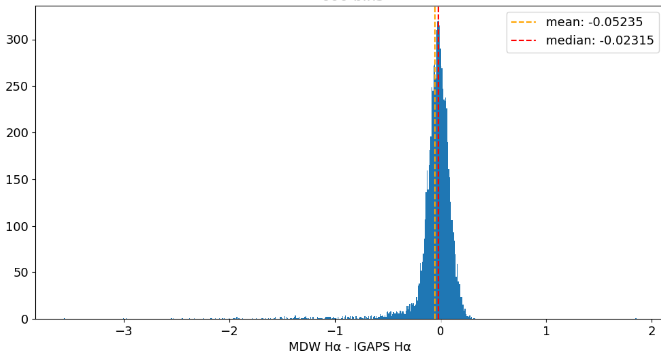
Field 0478 MDW H \alpha - IGAPS H \alpha 600 bins
