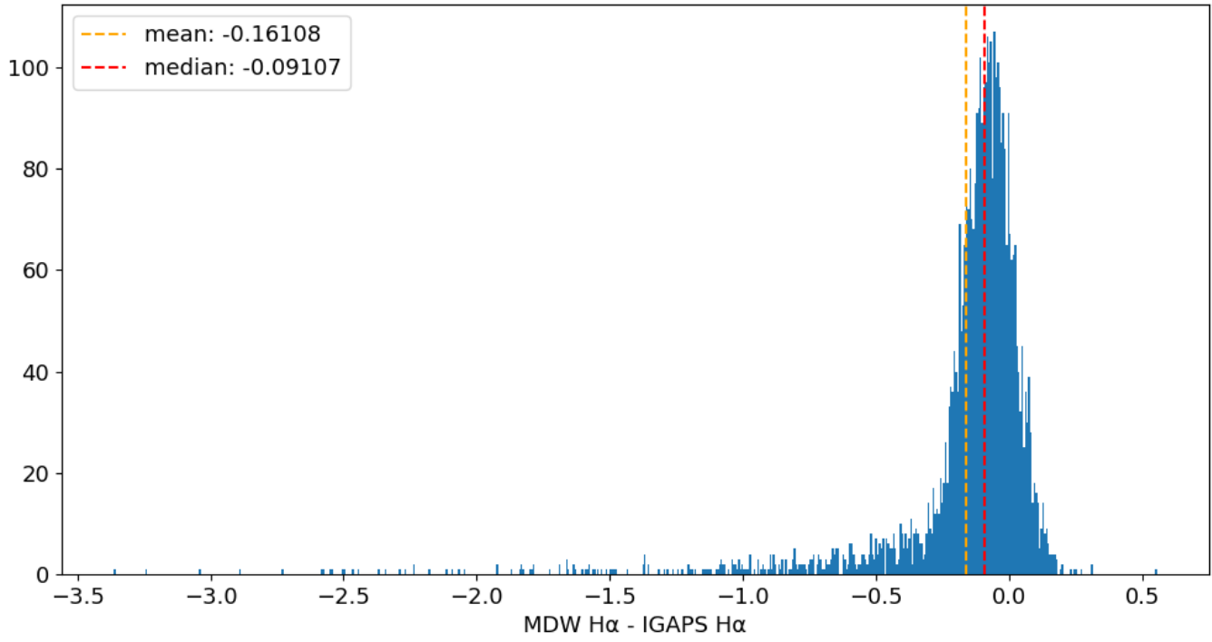
Field 0256 MDW H \alpha - IGAPS H \alpha 600 bins
