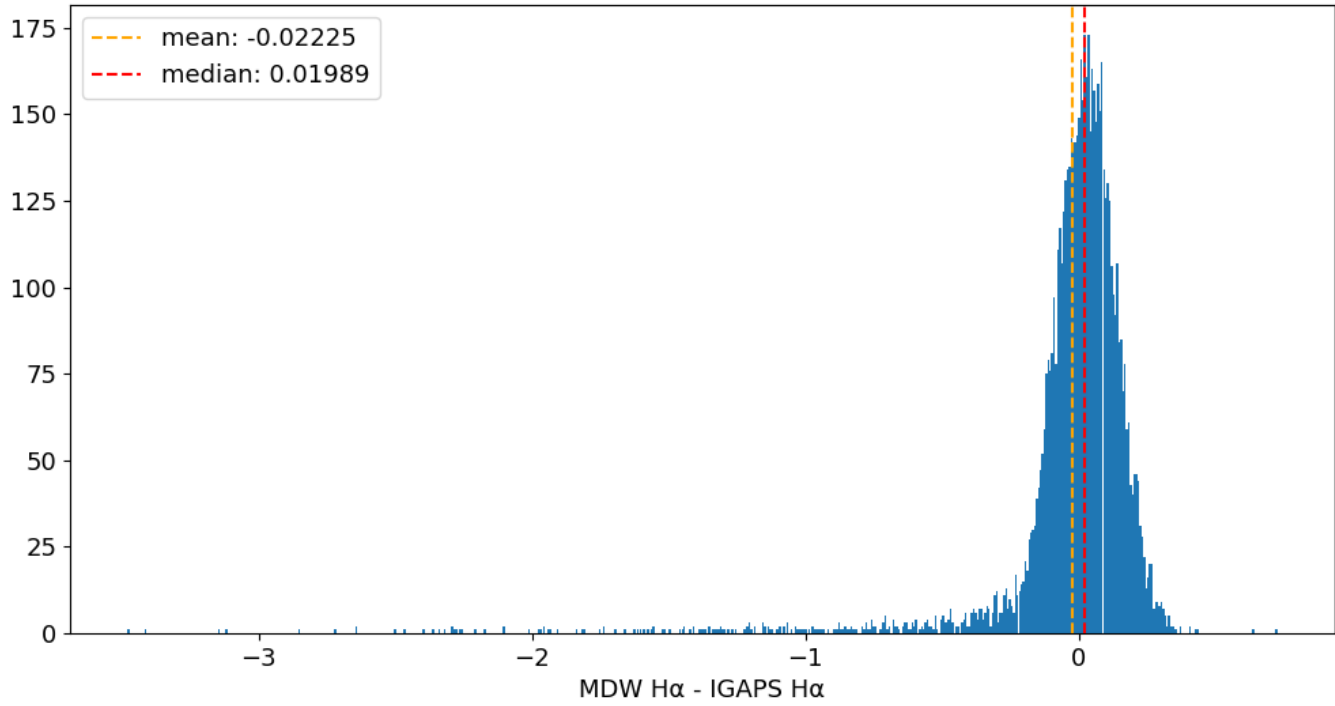
Field 0032 MDW H \alpha - IGAPS H \alpha 600 bins
