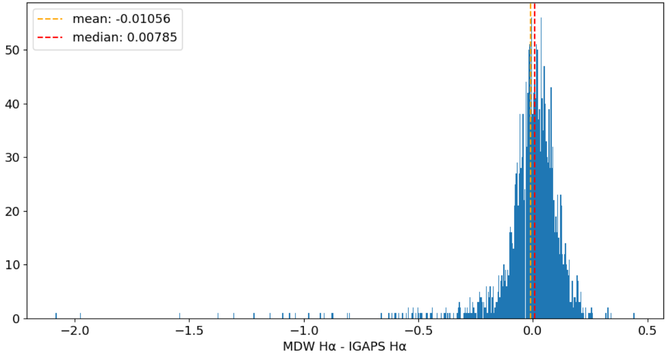
Field 0258 MDW H \alpha - IGAPS H \alpha 600 bins
