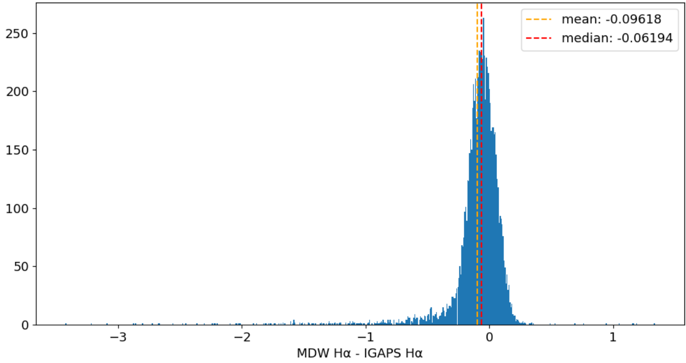
Field 0367 MDW H \alpha - IGAPS H \alpha 600 bins
