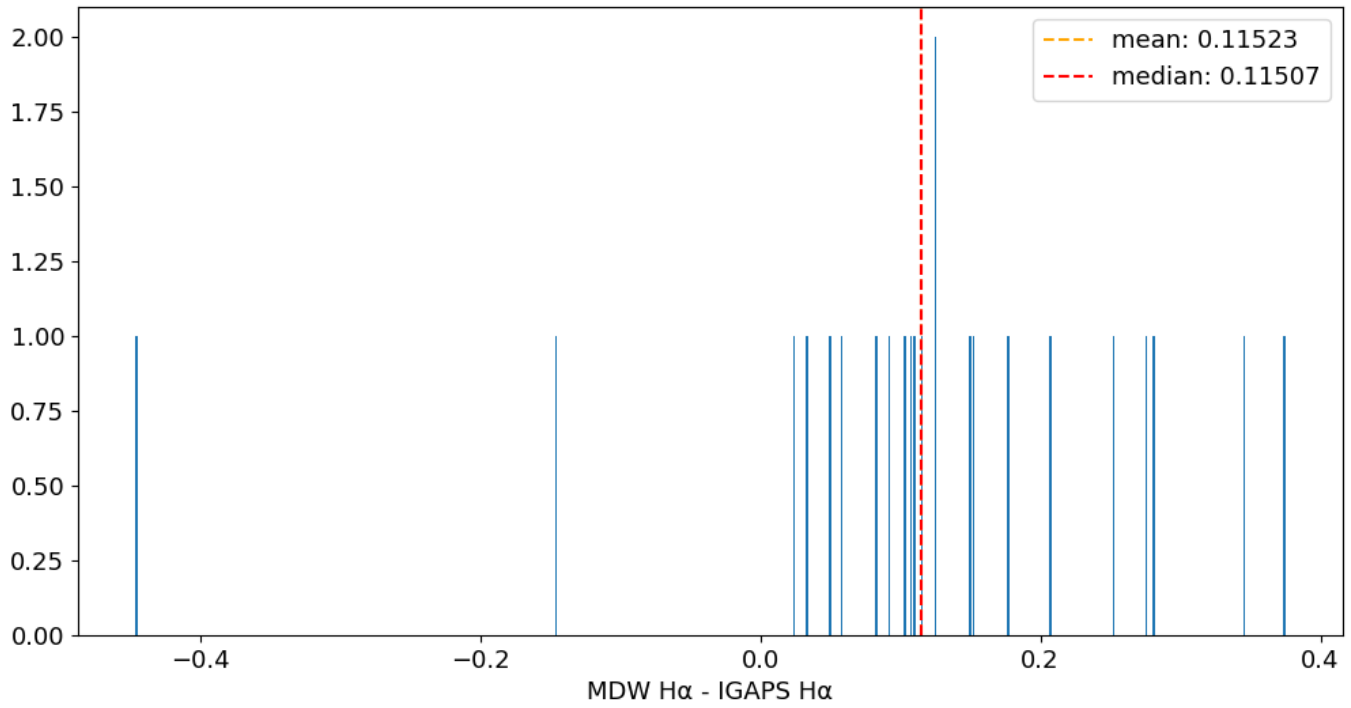
Field 0697 MDW H \alpha - IGAPS H \alpha 600 bins
