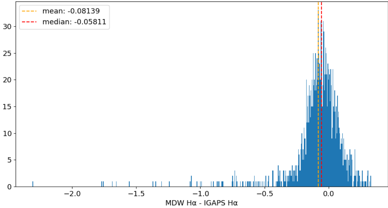
Field 2147 MDW H \alpha - IGAPS H \alpha 600 bins
