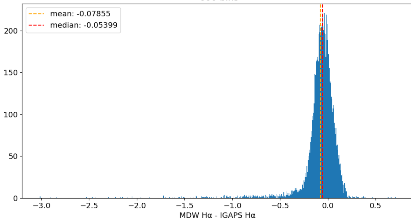
Field 0145 MDW H \alpha - IGAPS H \alpha 600 bins
