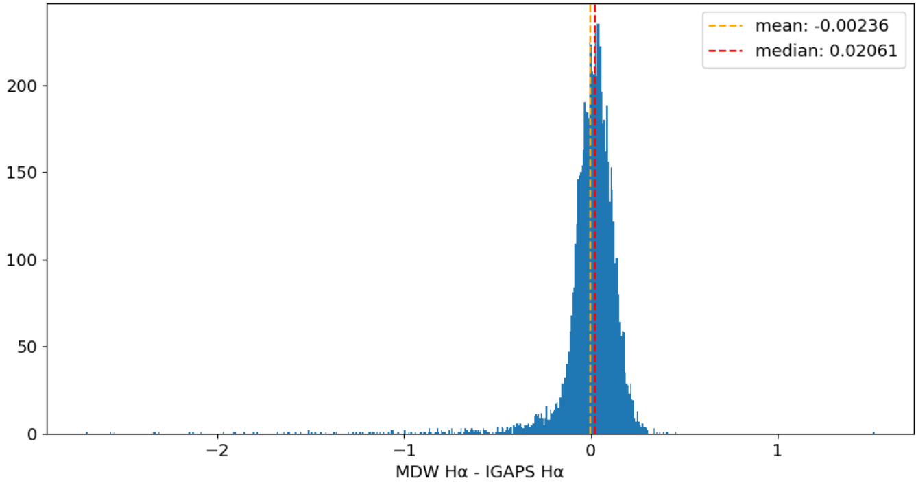
Field 0479 MDW H \alpha - IGAPS H \alpha 600 bins
