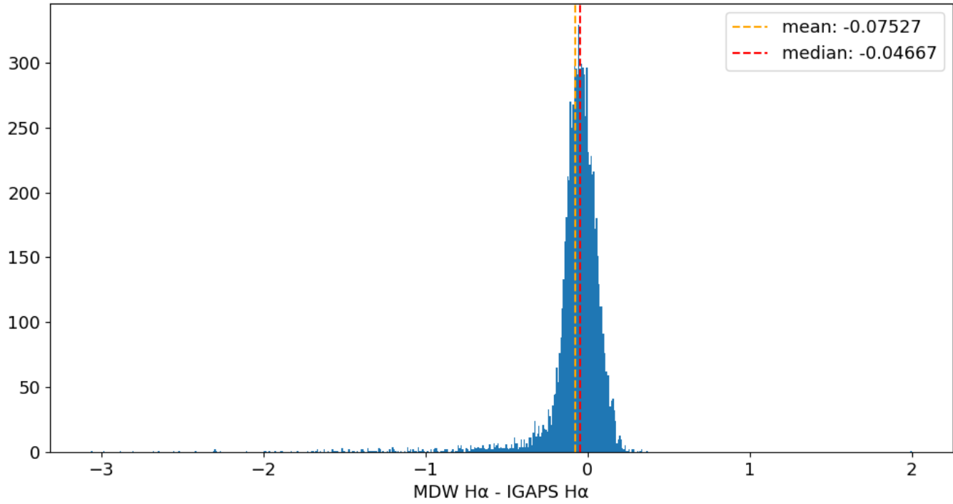
Field 0257 MDW H \alpha - IGAPS H \alpha 600 bins
