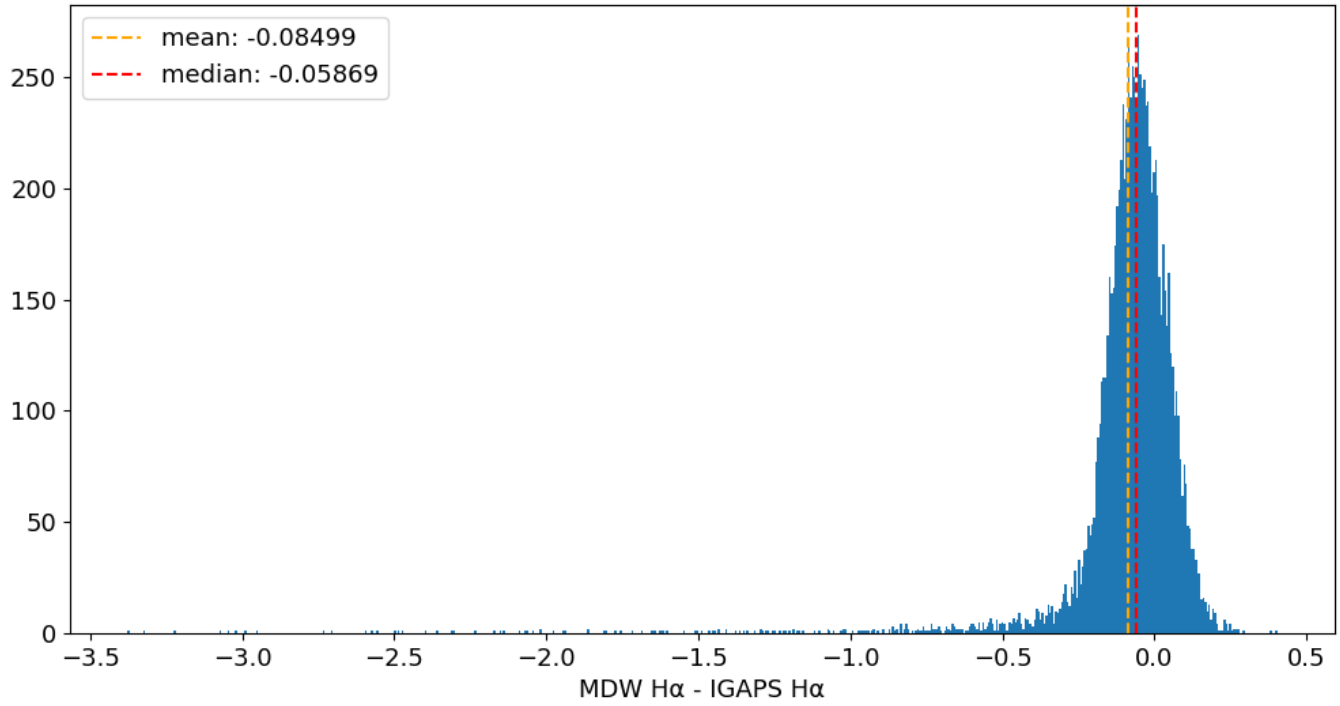
Field 0477 MDW H \alpha - IGAPS H \alpha 600 bins
