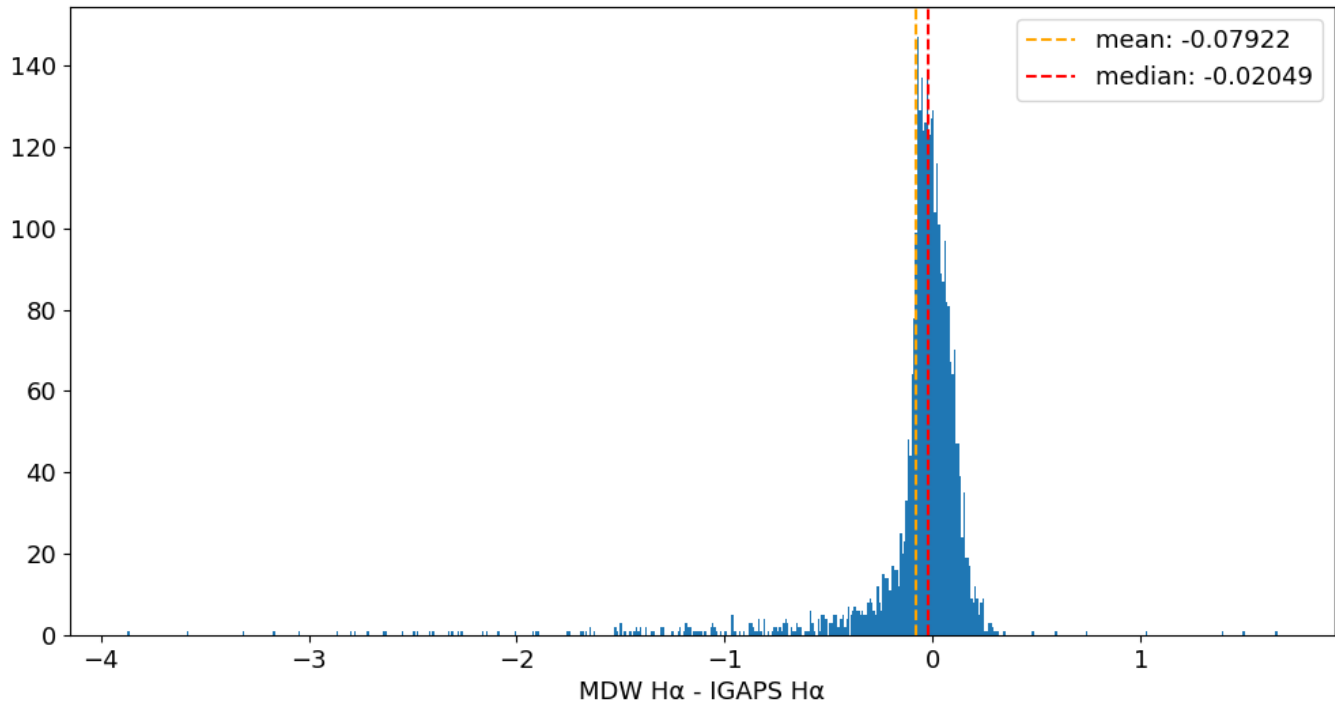
Field 0143 MDW H \alpha - IGAPS H \alpha 600 bins
