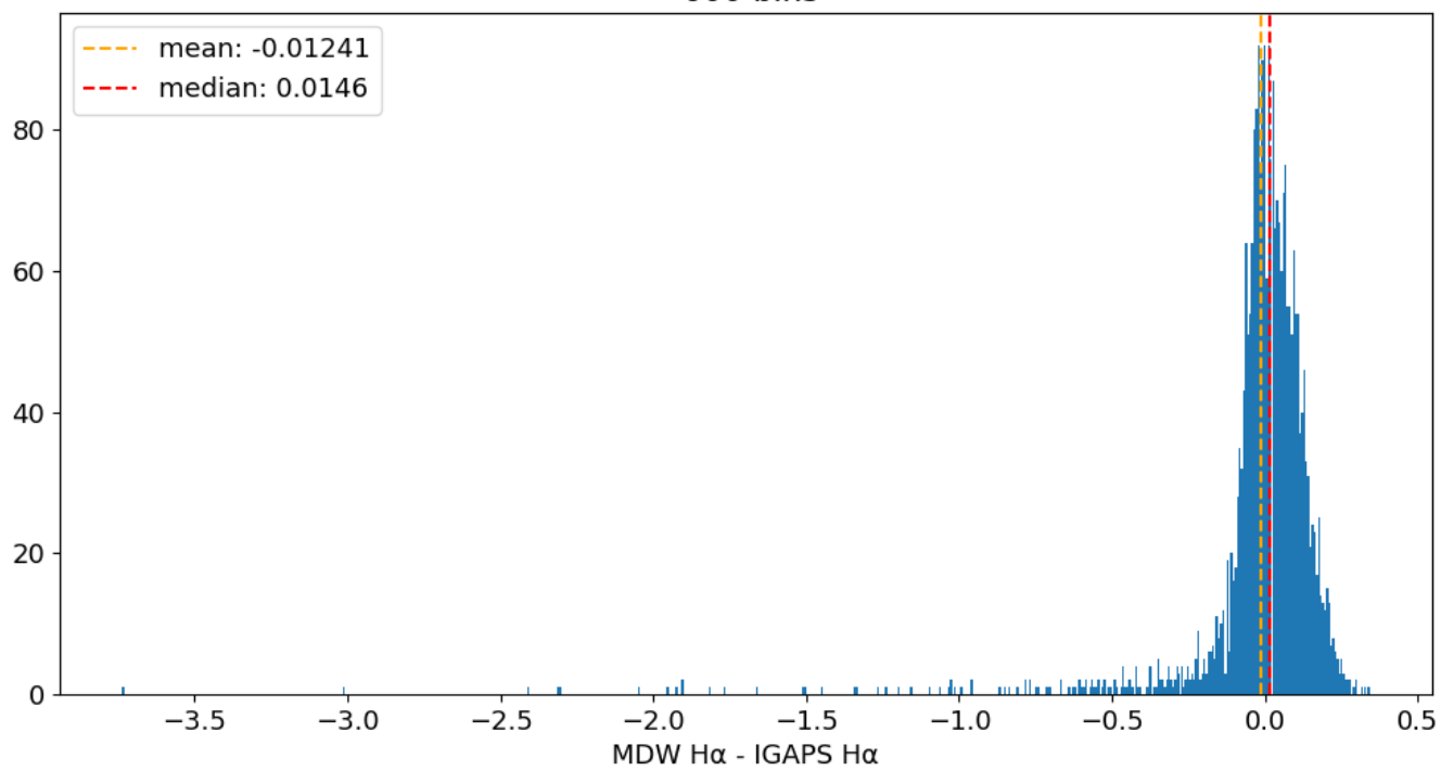
Field 0031 MDW H \alpha - IGAPS H \alpha 600 bins
