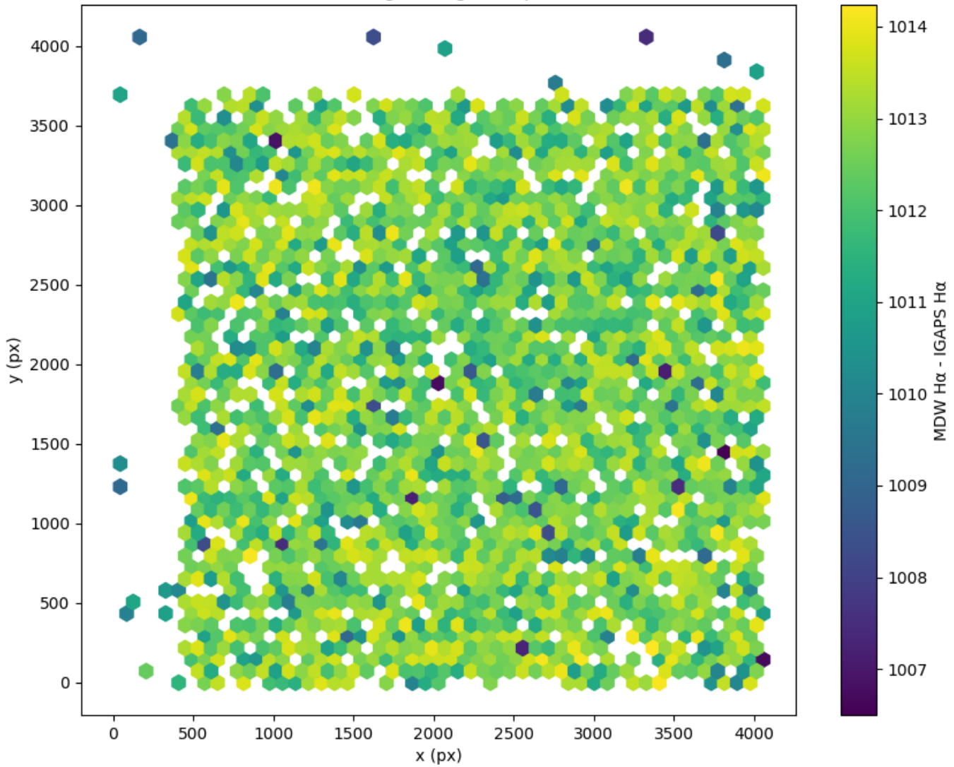
Field 2474 2D field distribution of (MDW H \alpha - Pan-STARRS r) Hexagon length: 81px
