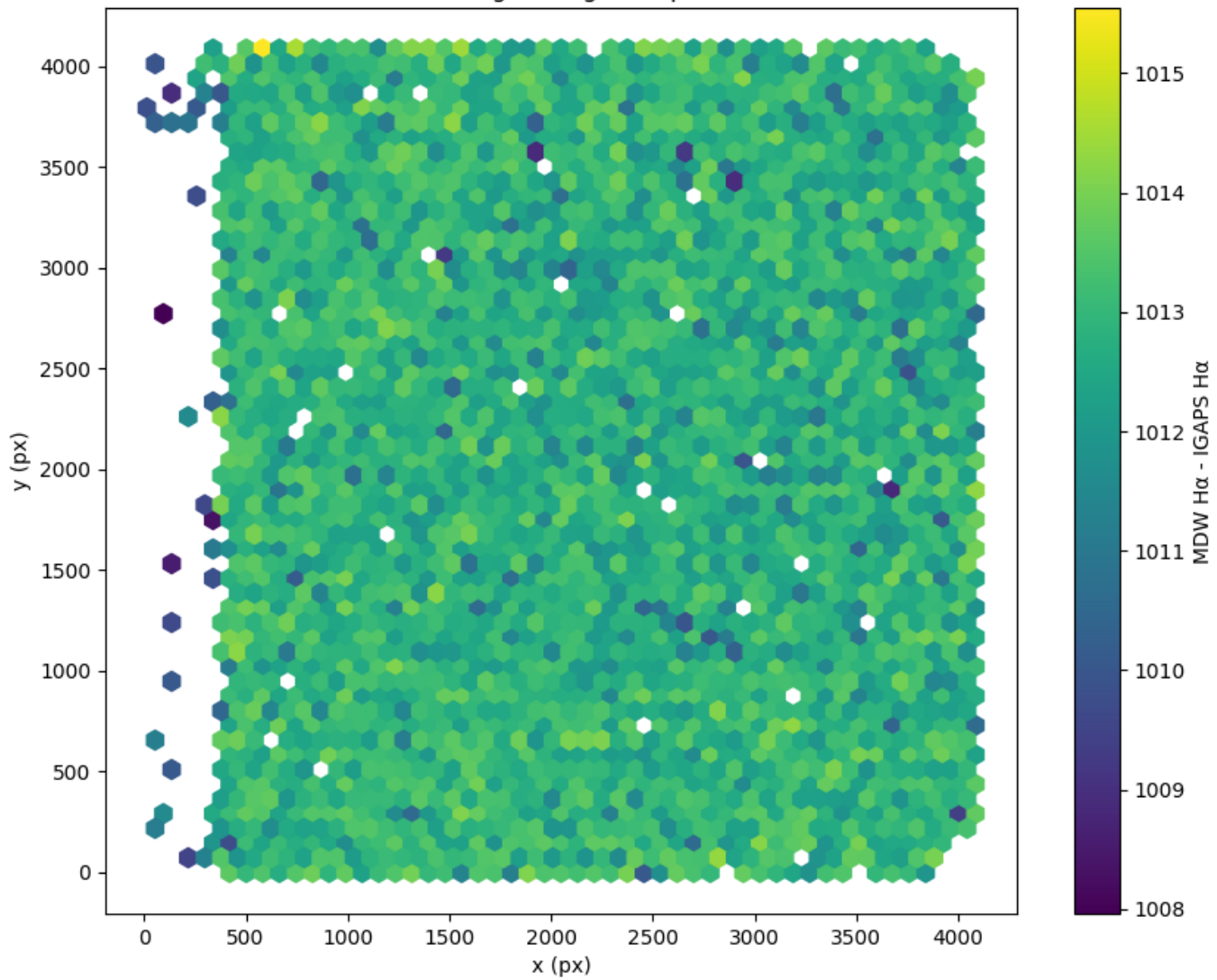
Field 0038 2D field distribution of (MDW H \alpha - Pan-STARRS r) Hexagon length: 81px
