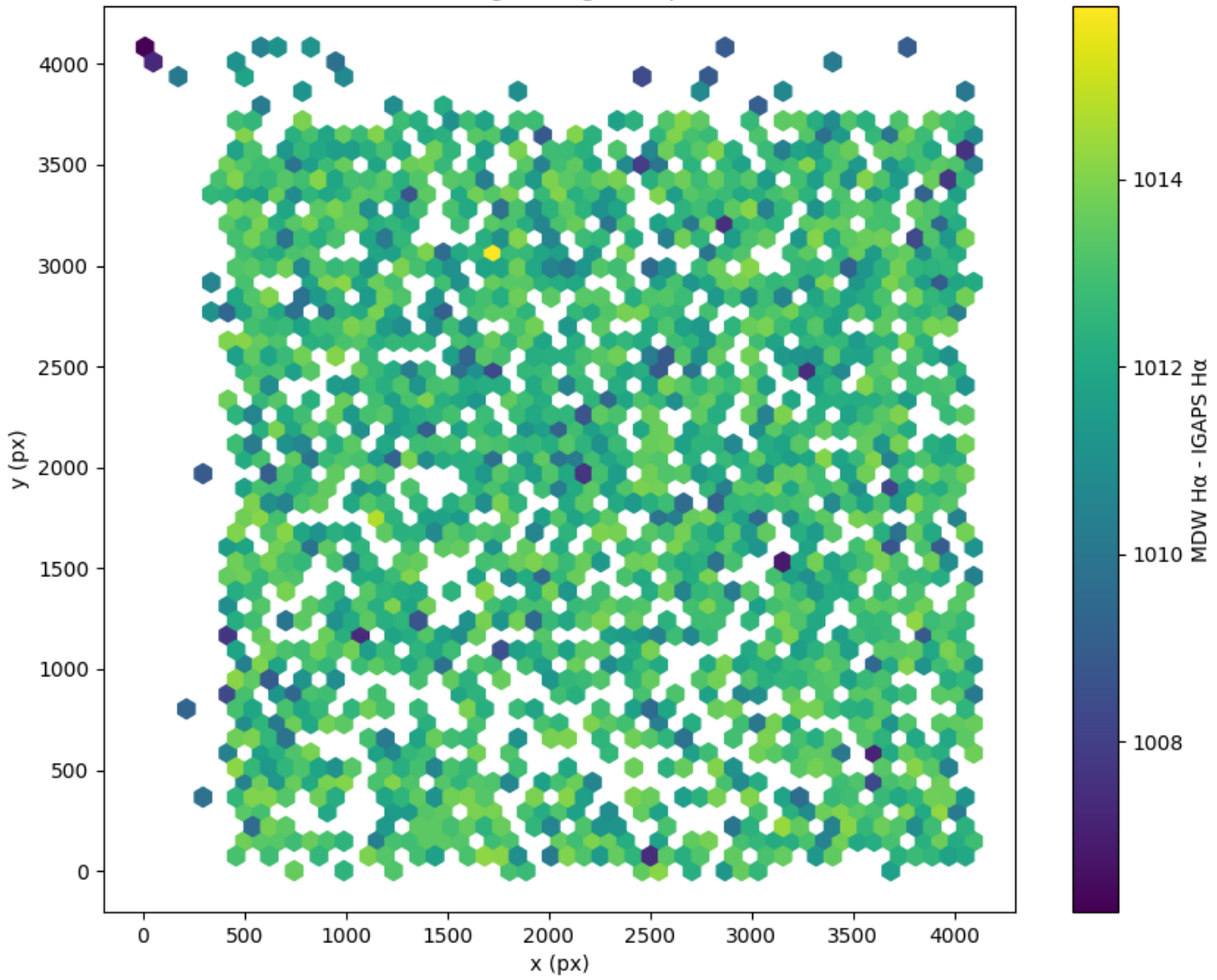
Field 2471 2D field distribution of (MDW H \alpha - Pan-STARRS r) Hexagon length: 82px
