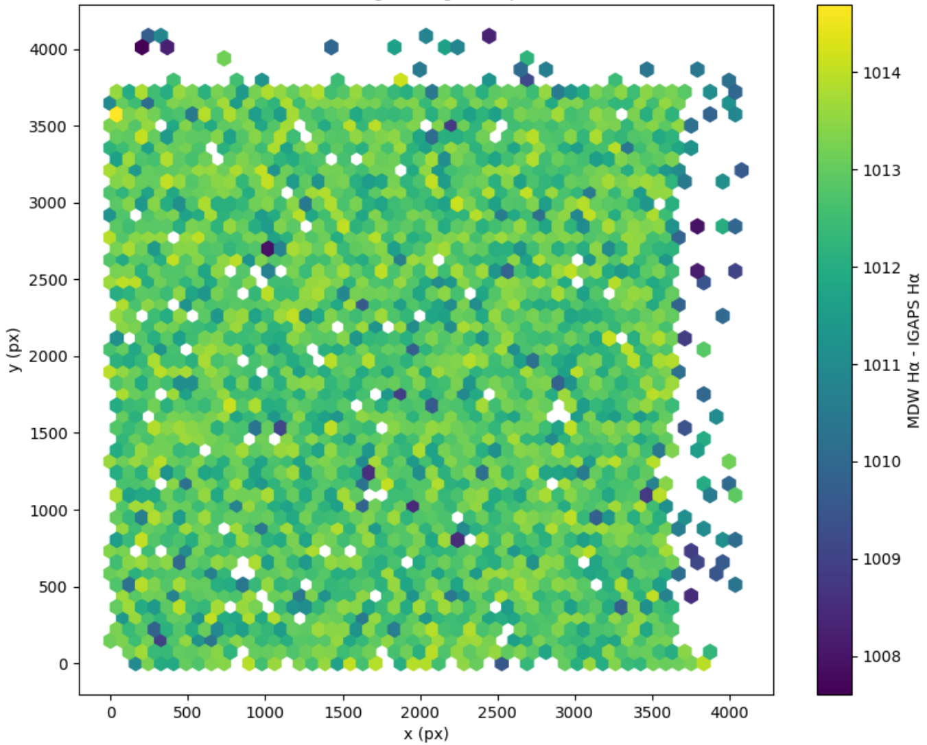
Field 0807 2D field distribution of (MDW H \alpha - Pan-STARRS r) Hexagon length: 82px
