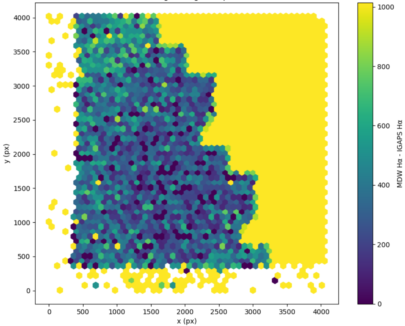
Field 0479 2D field distribution of (MDW H \alpha - Pan-STARRS r) Hexagon length: 81px
