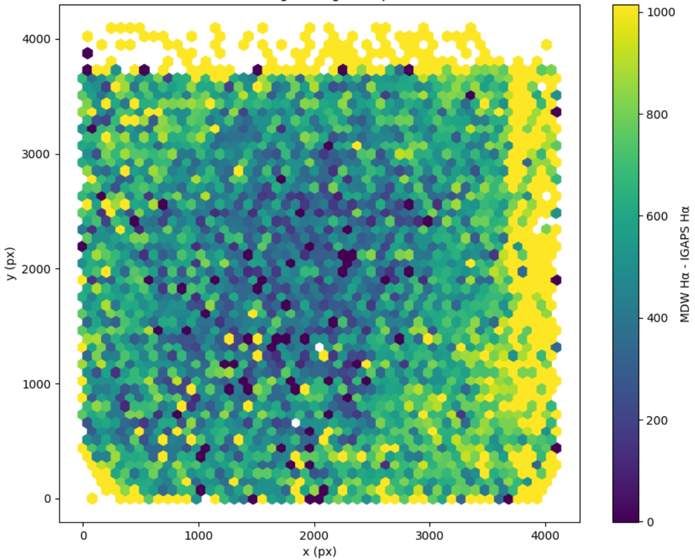
Field 0145 2D field distribution of (MDW H \alpha - Pan-STARRS r) Hexagon length: 82px
