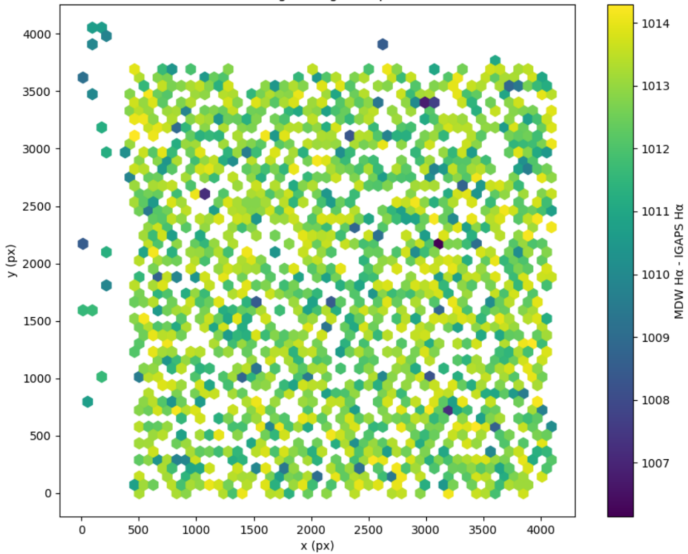
Field 2791 2D field distribution of (MDW H \alpha - Pan-STARRS r) Hexagon length: 82px
