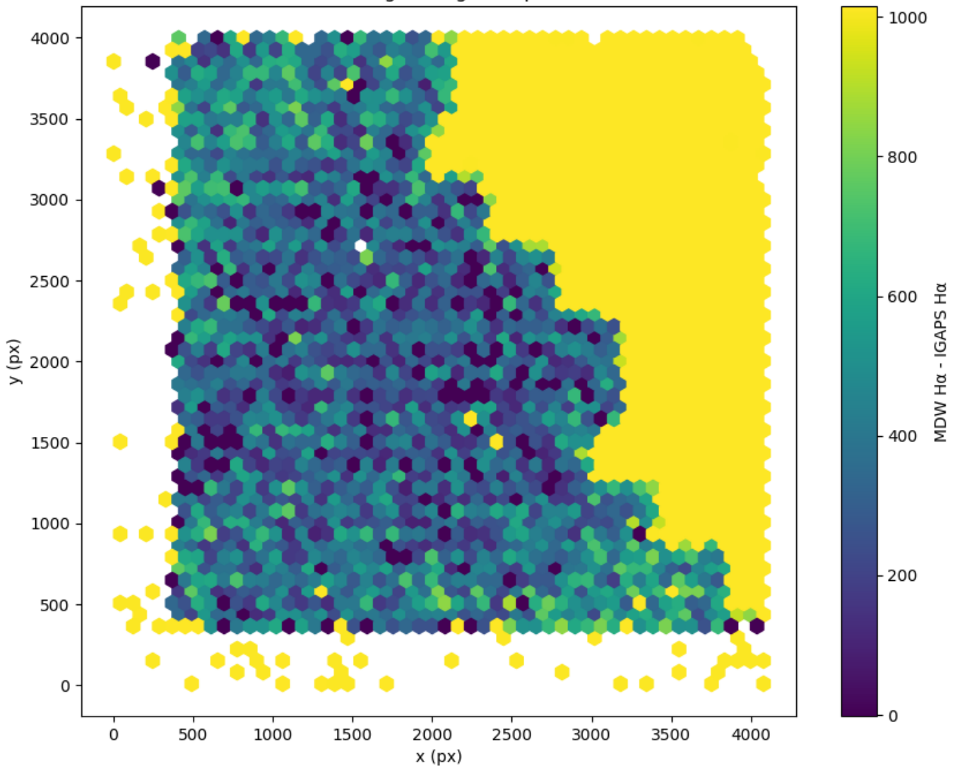
Field 0146 2D field distribution of (MDW H \alpha - Pan-STARRS r) Hexagon length: 82px
