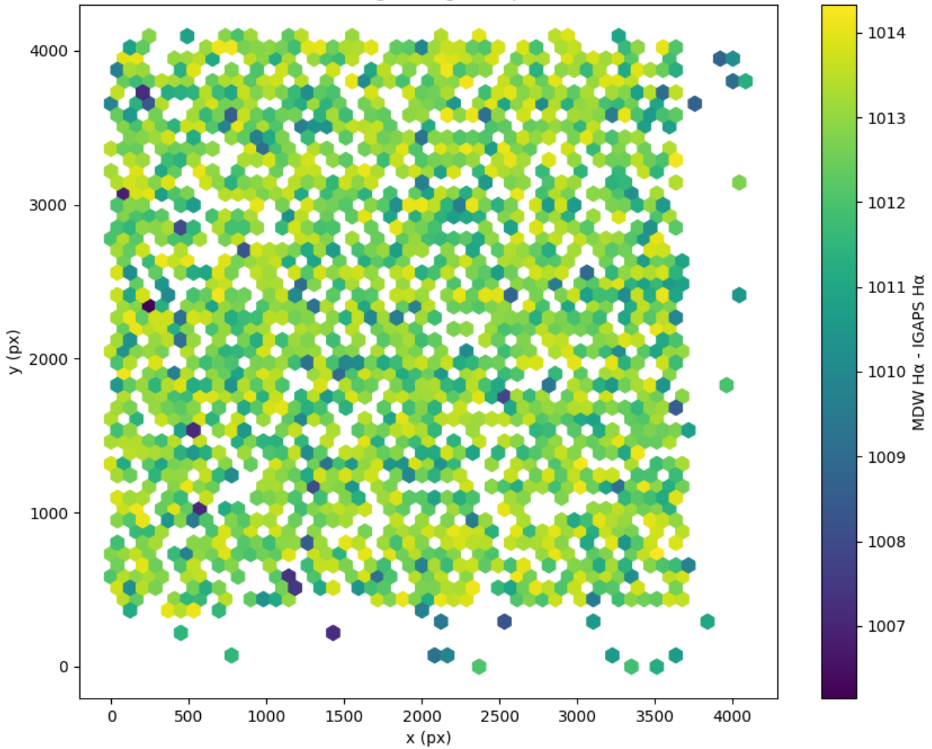
Field 2359 2D field distribution of (MDW H \alpha - Pan-STARRS r) Hexagon length: 82px
