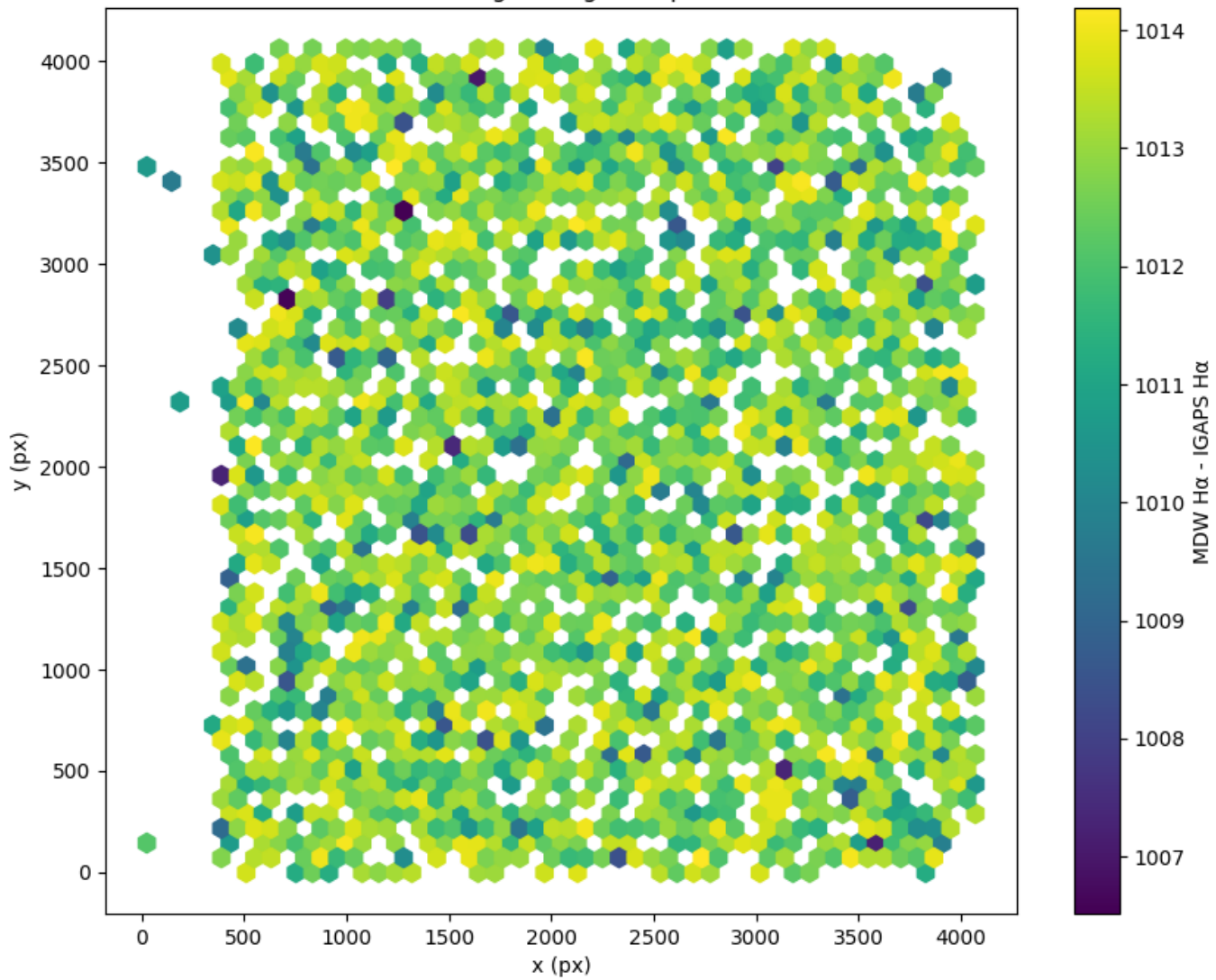
Field 2135 2D field distribution of (MDW H \alpha - Pan-STARRS r) Hexagon length: 81px
