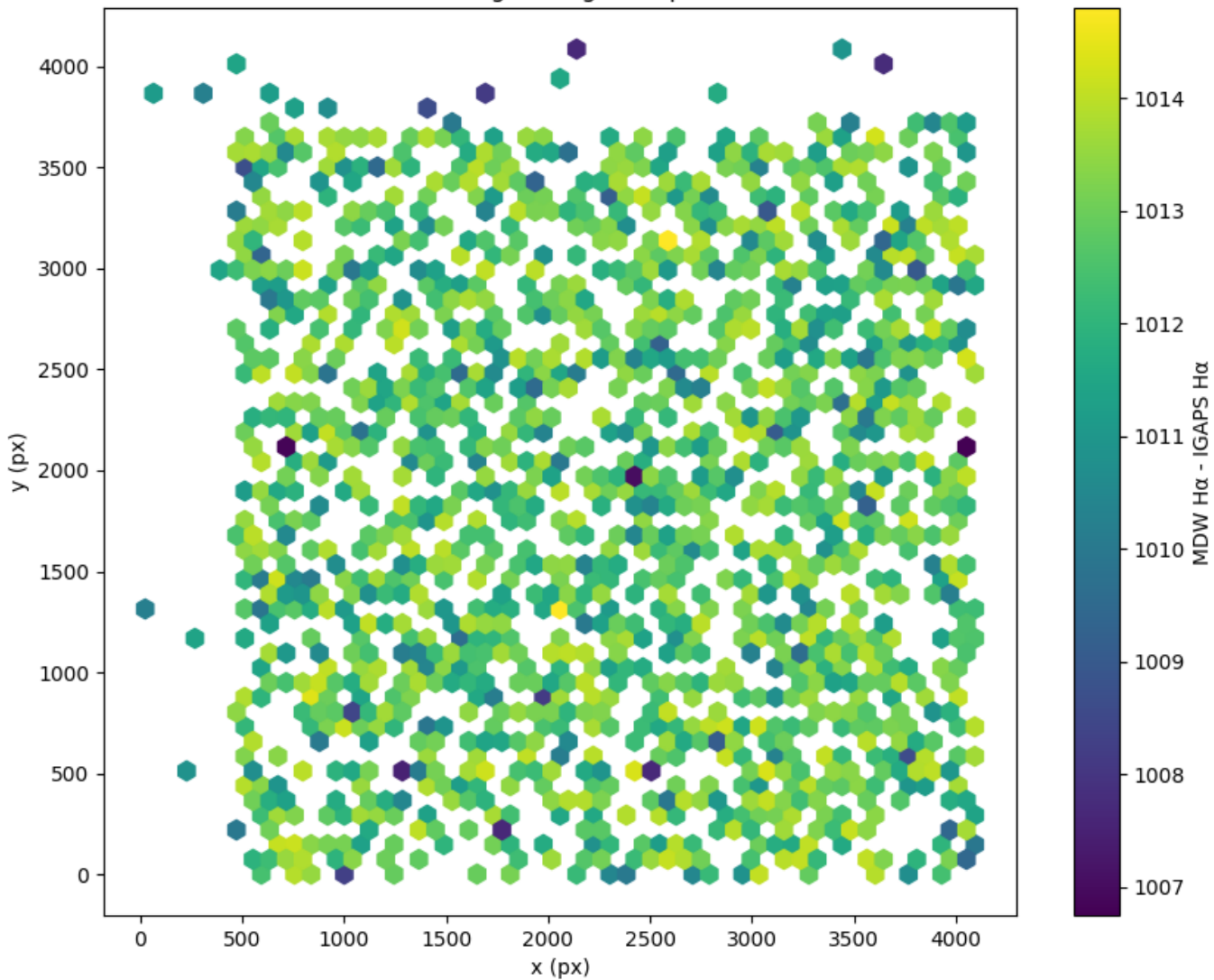
Field 2574 2D field distribution of (MDW H \alpha - Pan-STARRS r) Hexagon length: 81px
