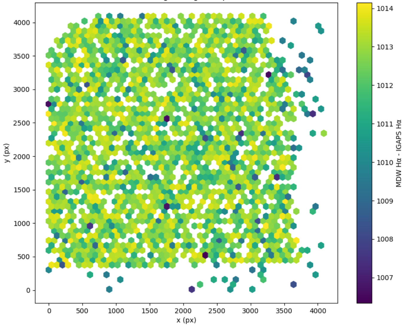
Field 2797 2D field distribution of (MDW H \alpha - Pan-STARRS r) Hexagon length: 82px
