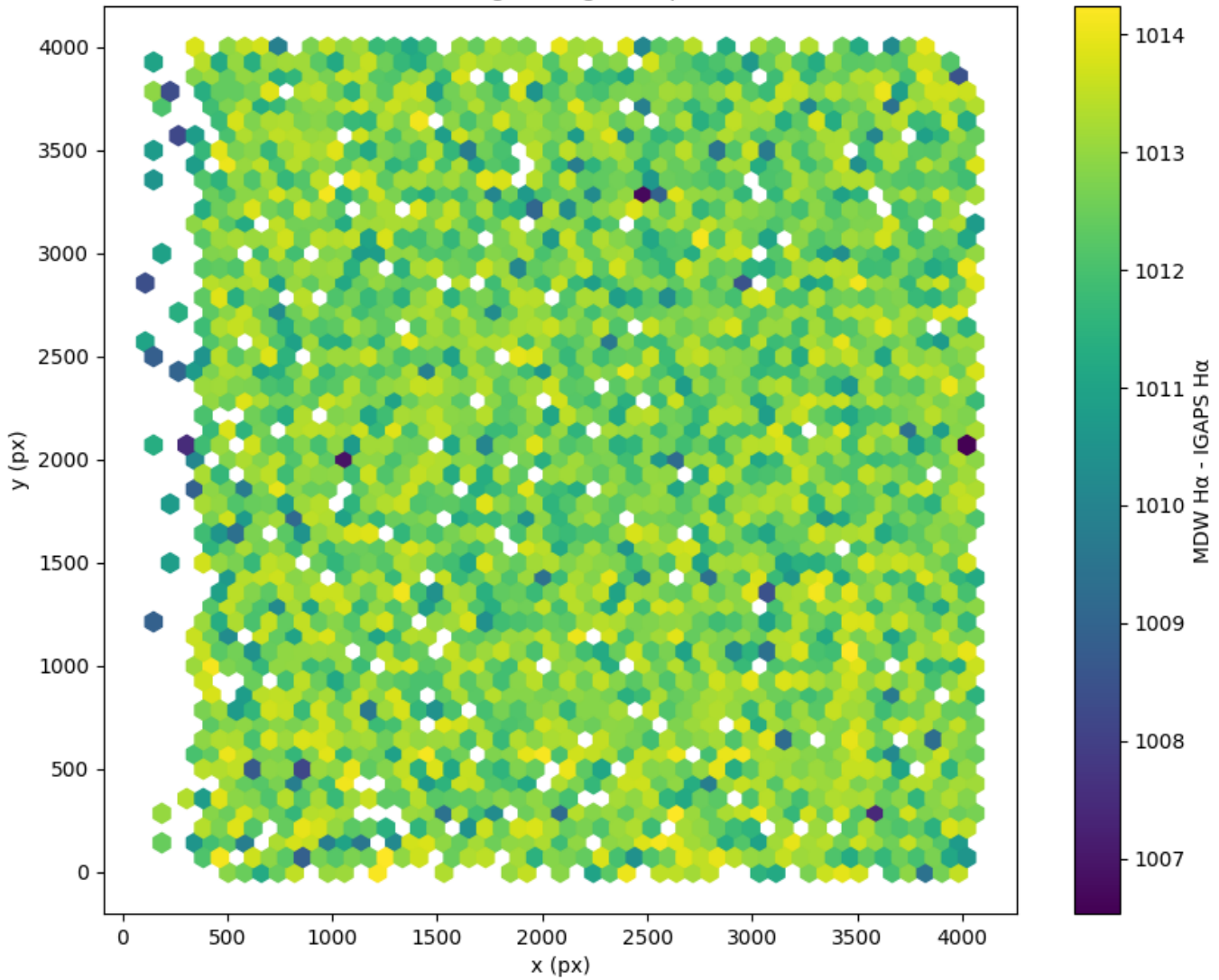
Field 0026 2D field distribution of (MDW H \alpha - Pan-STARRS r) Hexagon length: 79px
