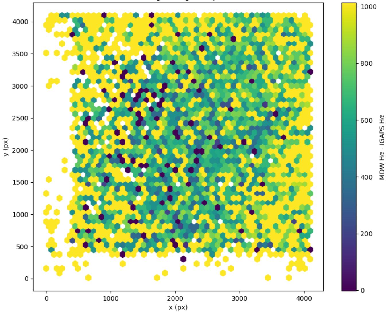
Field 0144 2D field distribution of (MDW H \alpha - Pan-STARRS r) Hexagon length: 82px
