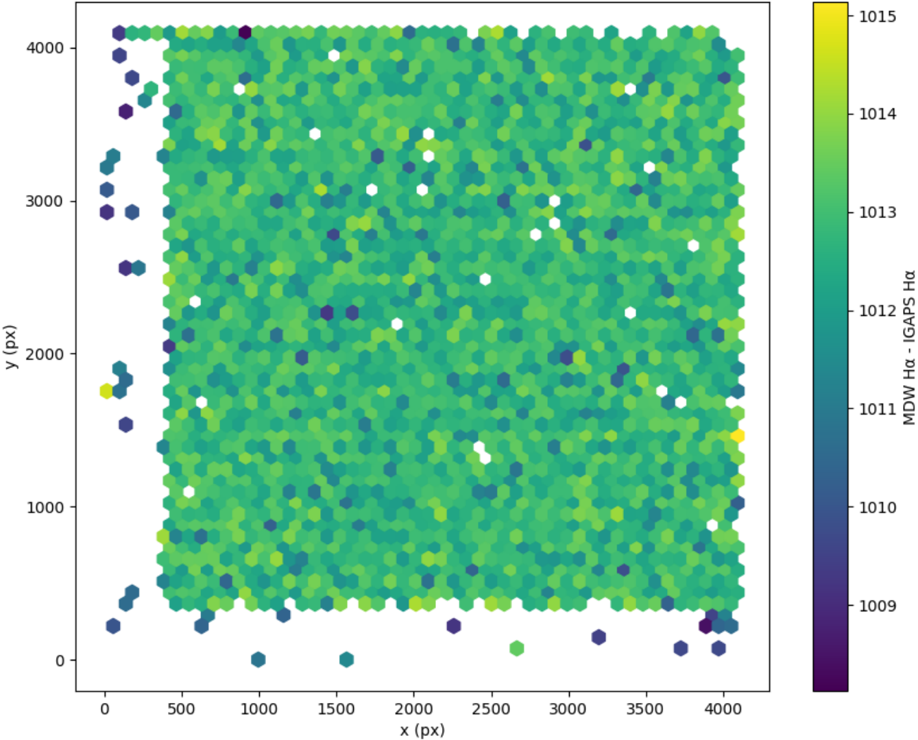
Field 0261 2D field distribution of (MDW H \alpha - Pan-STARRS r) Hexagon length: 81px
