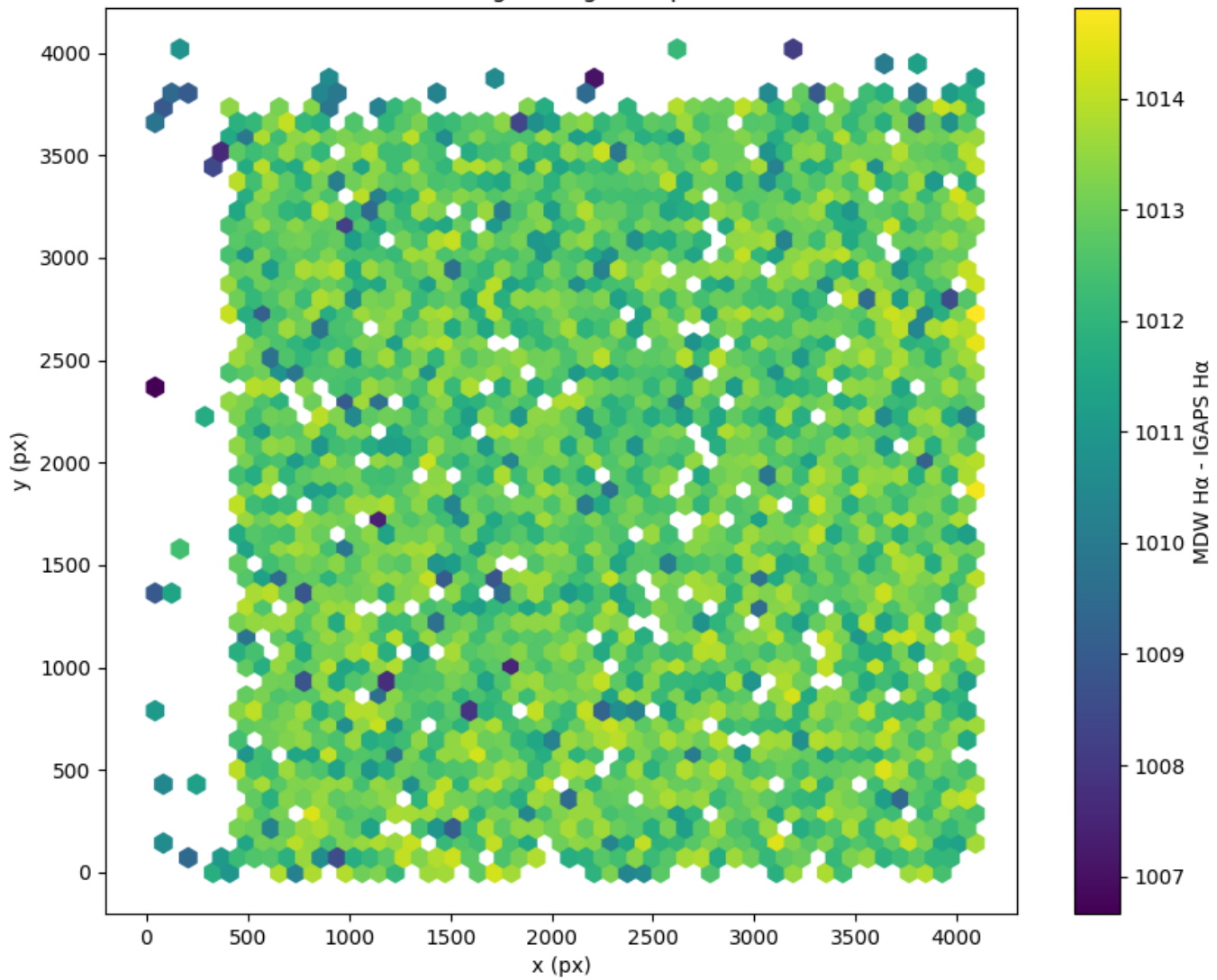
Field 2586 2D field distribution of (MDW H \alpha - Pan-STARRS r) Hexagon length: 82px
