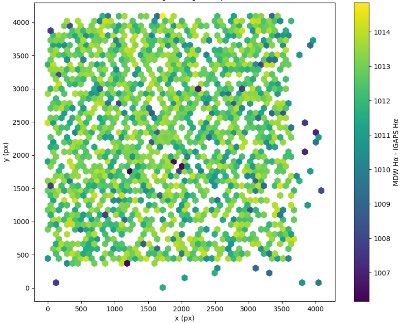
Field 2896 2D field distribution of (MDW H \alpha - Pan-STARRS r) Hexagon length: 82px
