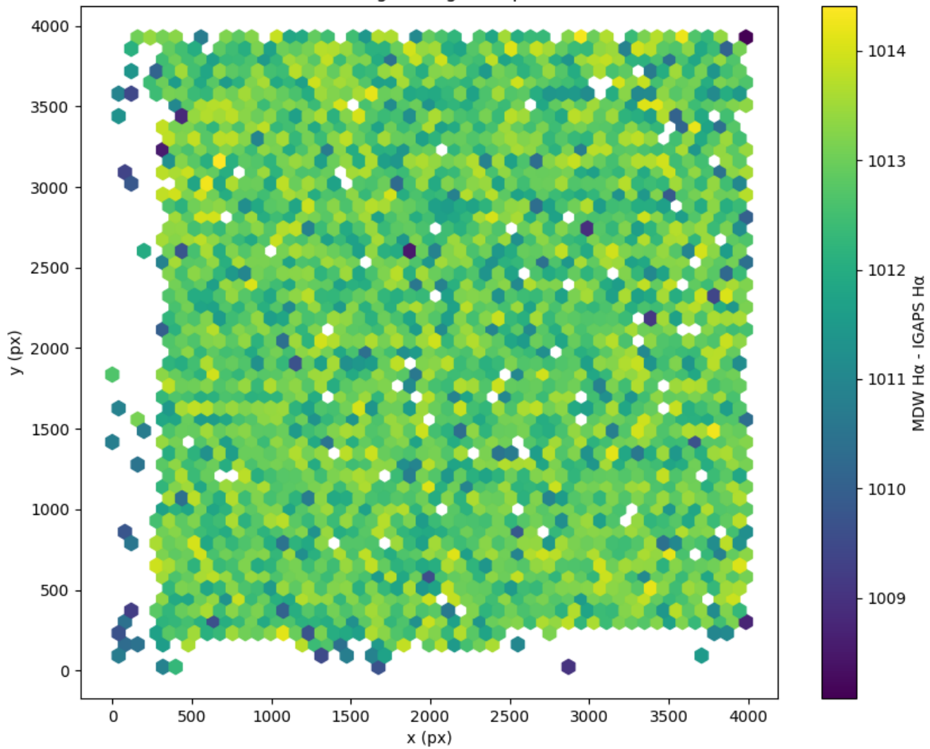
Field 0483 2D field distribution of (MDW H \alpha - Pan-STARRS r) Hexagon length: 80px
