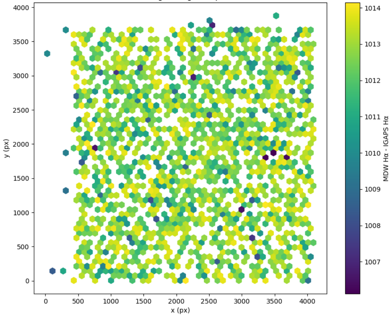
Field 2685 2D field distribution of (MDW H \alpha - Pan-STARRS r) Hexagon length: 81px
