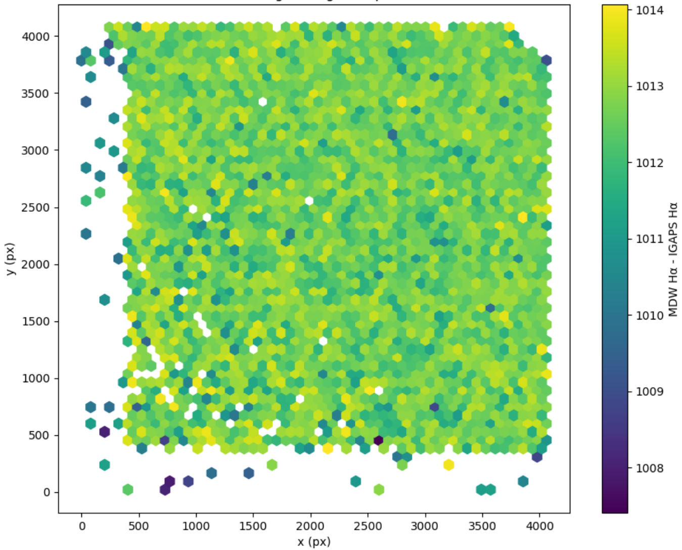
Field 0253 2D field distribution of (MDW H \alpha - Pan-STARRS r) Hexagon length: 81px
