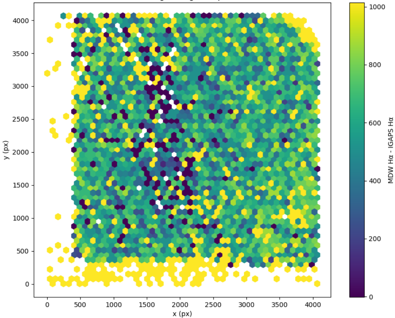
Field 0368 2D field distribution of (MDW H \alpha - Pan-STARRS r) Hexagon length: 81px
