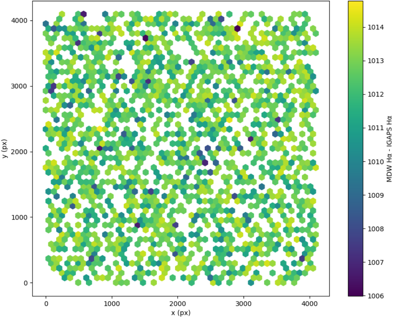
Field 2572 2D field distribution of (MDW H \alpha - Pan-STARRS r) Hexagon length: 82px
