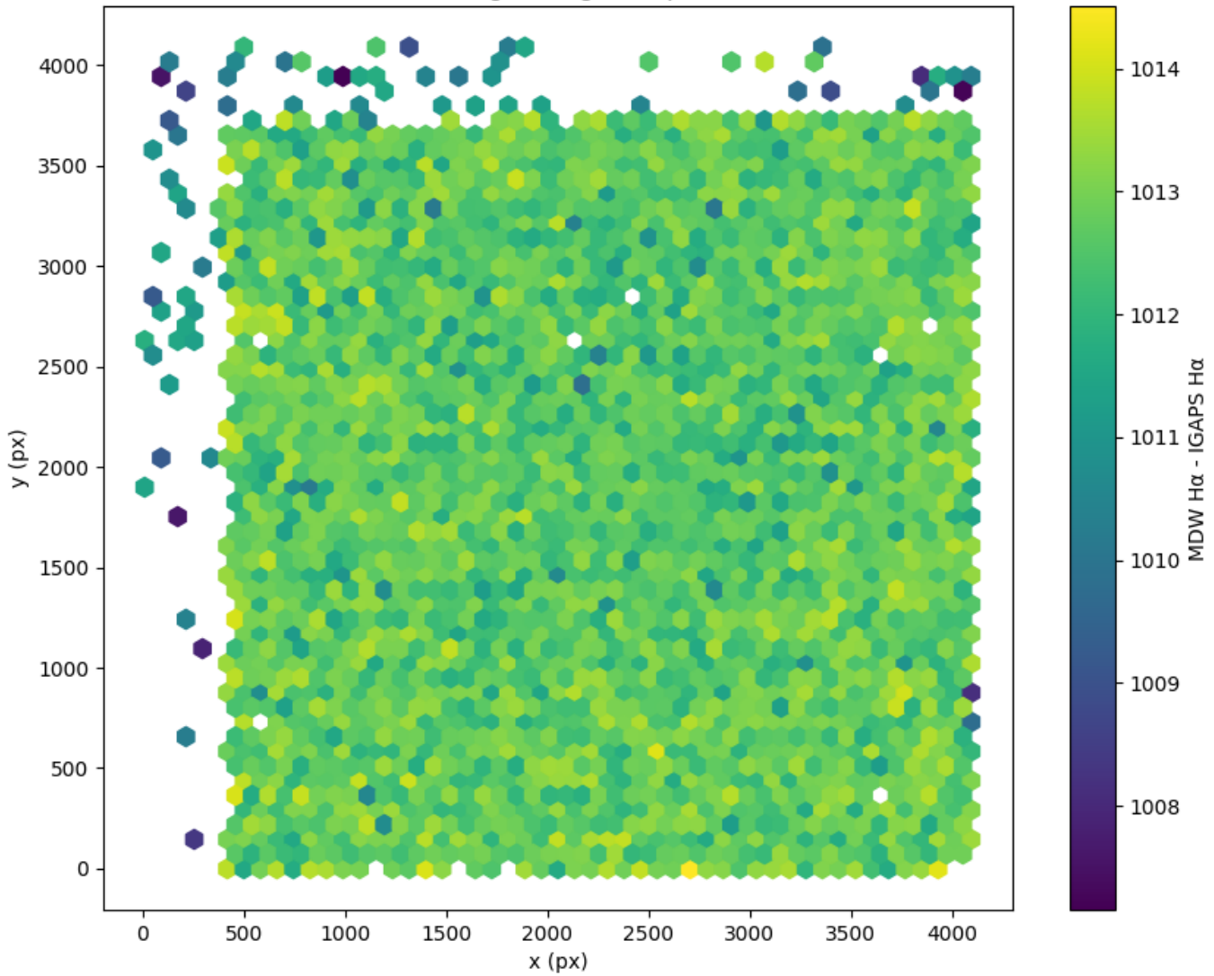
Field 2480 2D field distribution of (MDW H \alpha - Pan-STARRS r) Hexagon length: 82px
