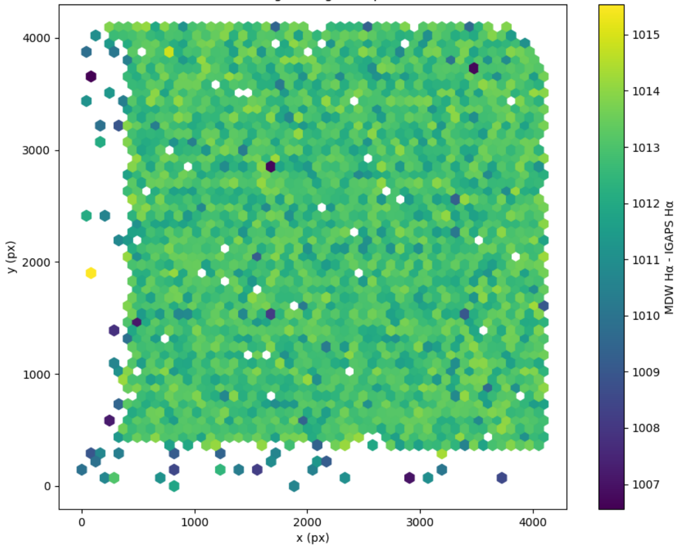
Field 0373 2D field distribution of (MDW H \alpha - Pan-STARRS r) Hexagon length: 82px
