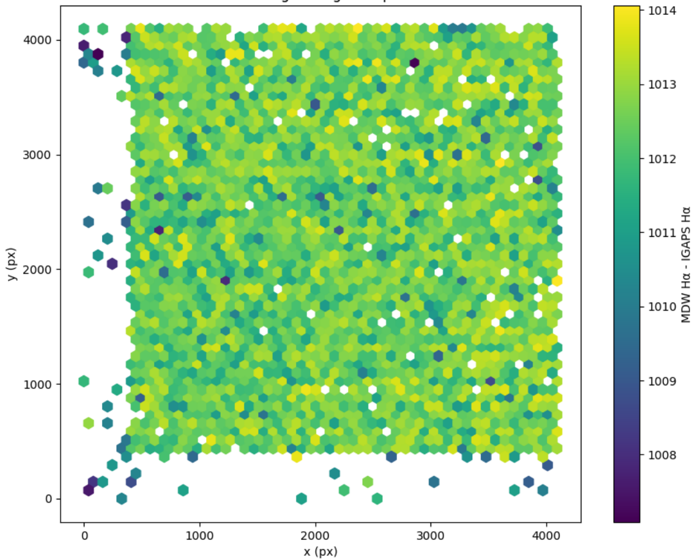
Field 0139 2D field distribution of (MDW H \alpha - Pan-STARRS r) Hexagon length: 82px
