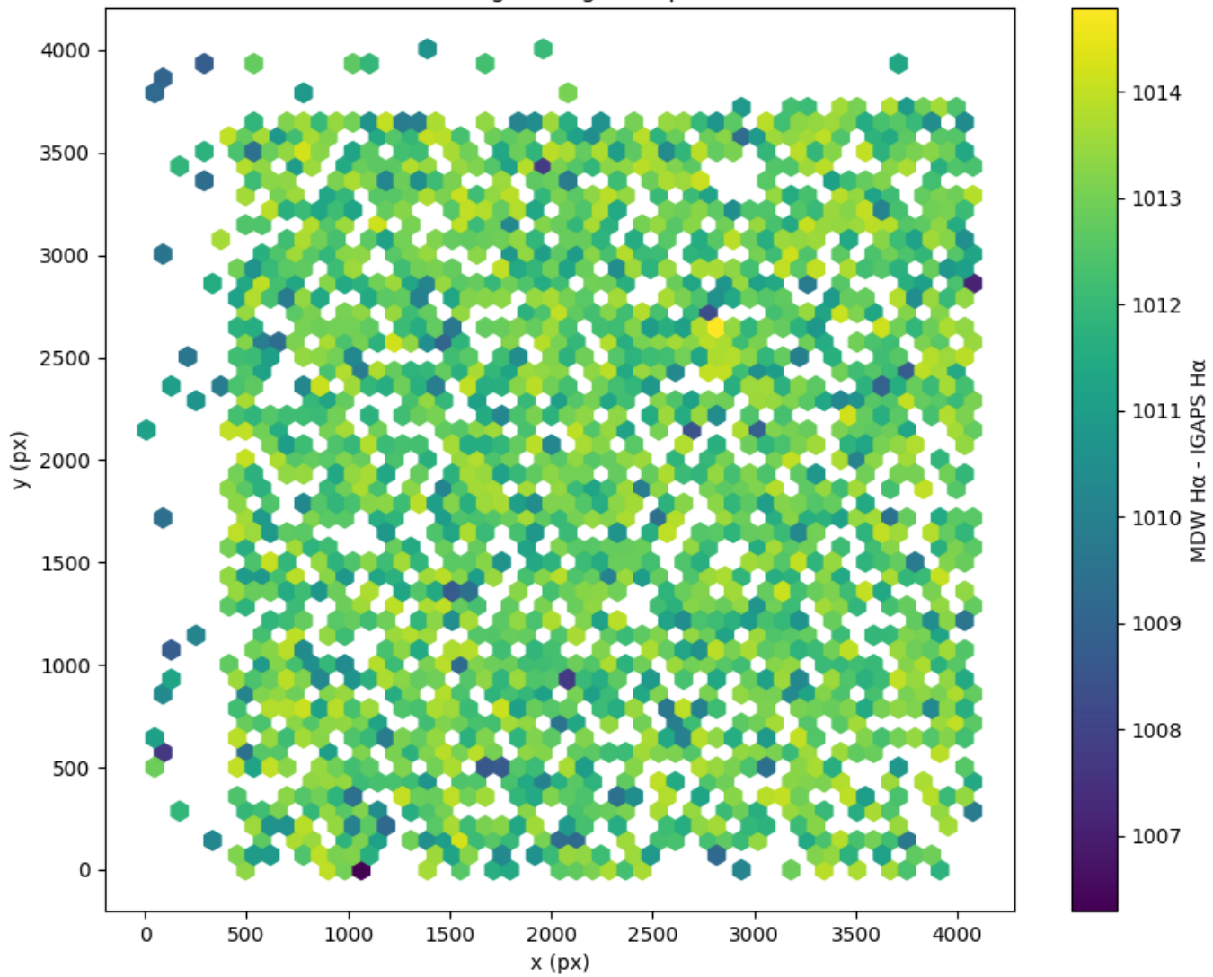
Field 2470 2D field distribution of (MDW H \alpha - Pan-STARRS r) Hexagon length: 81px
