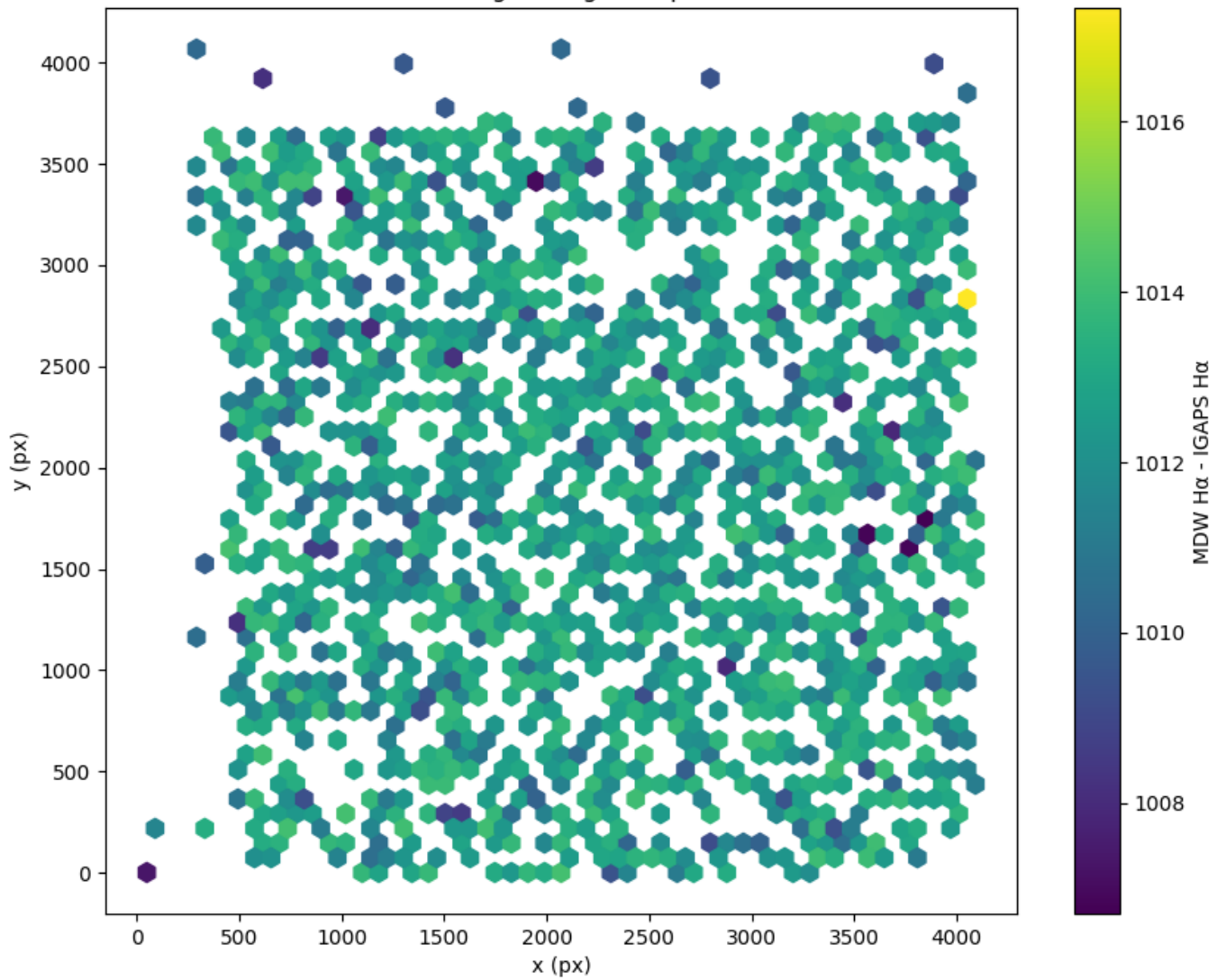
Field 2893 2D field distribution of (MDW H \alpha - Pan-STARRS r) Hexagon length: 81px
