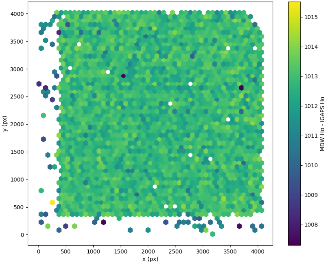
Field 0371 2D field distribution of (MDW H \alpha - Pan-STARRS r) Hexagon length: 81px
