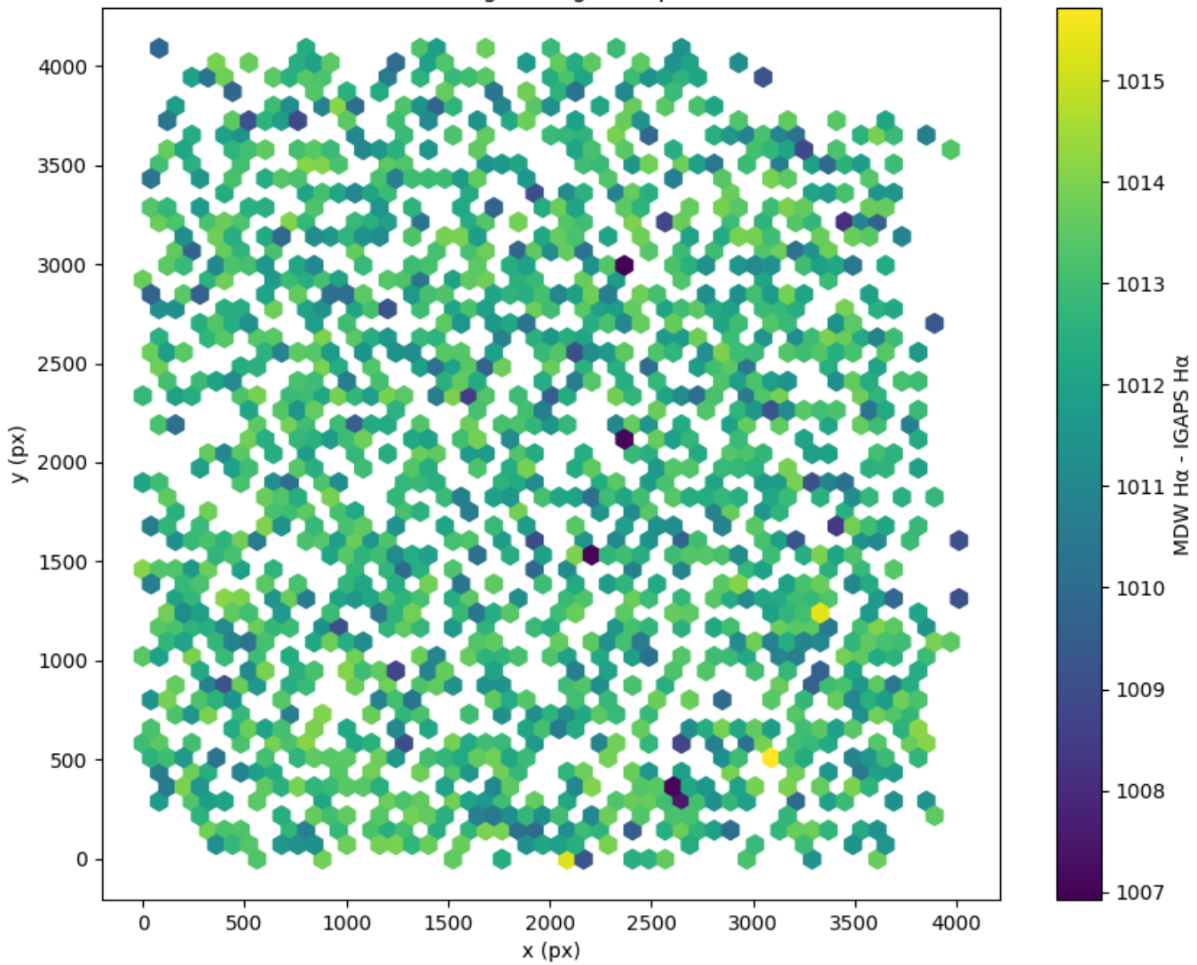
Field 2680 2D field distribution of (MDW H \alpha - Pan-STARRS r) Hexagon length: 80px
