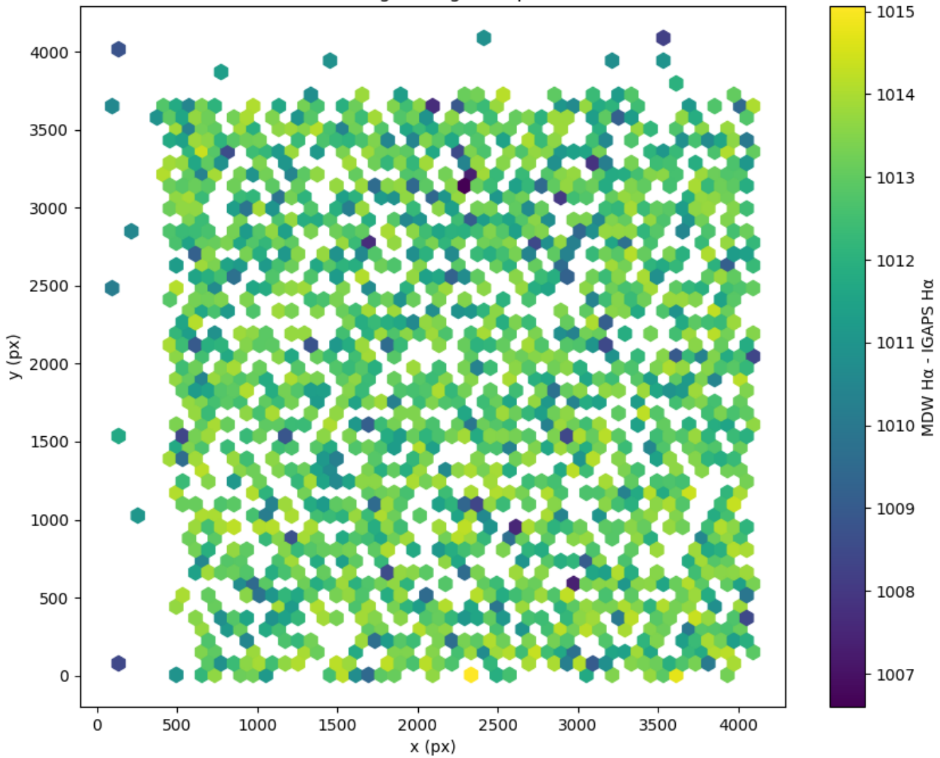
Field 2897 2D field distribution of (MDW H \alpha - Pan-STARRS r) Hexagon length: 80px
