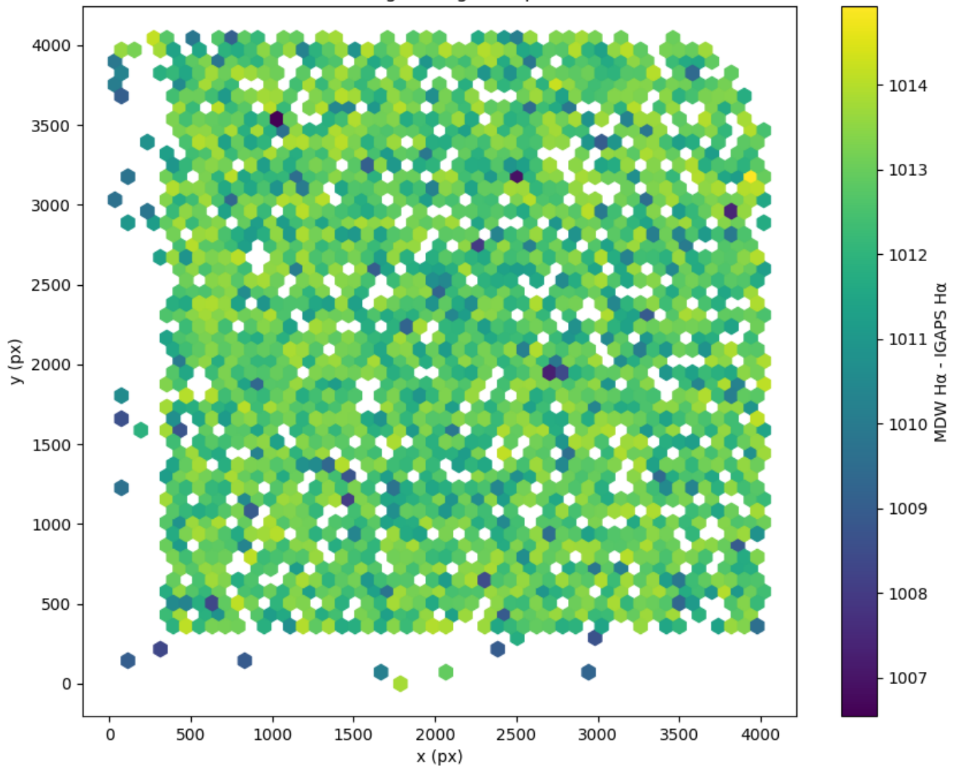
Field 0704 2D field distribution of (MDW H \alpha - Pan-STARRS r) Hexagon length: 80px
