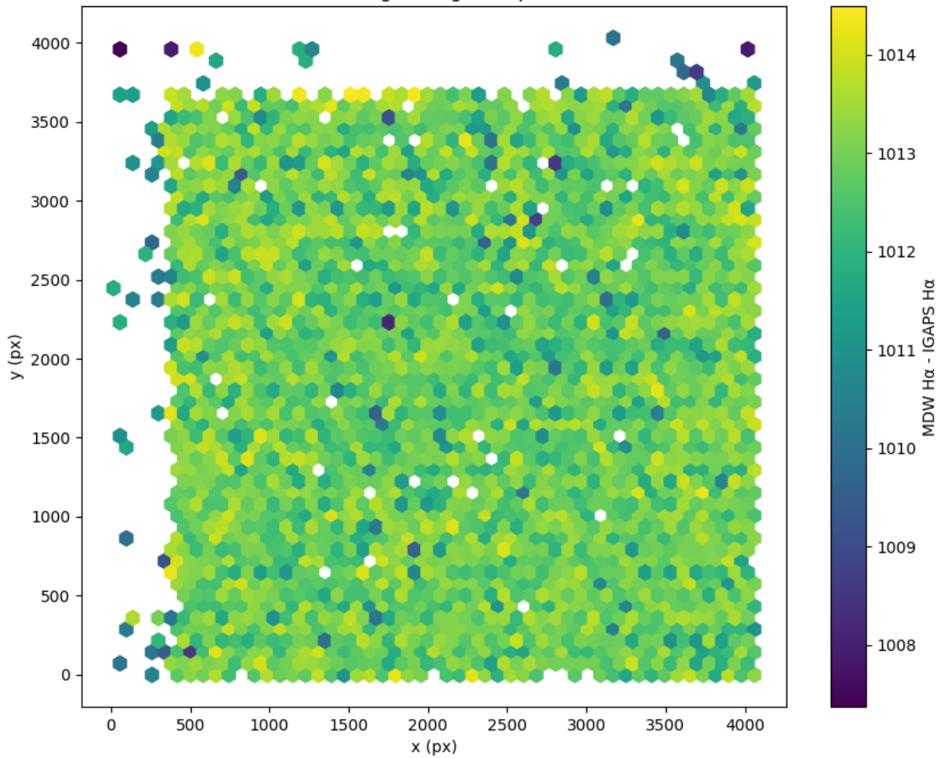
Field 2479 2D field distribution of (MDW H \alpha - Pan-STARRS r) Hexagon length: 81px
