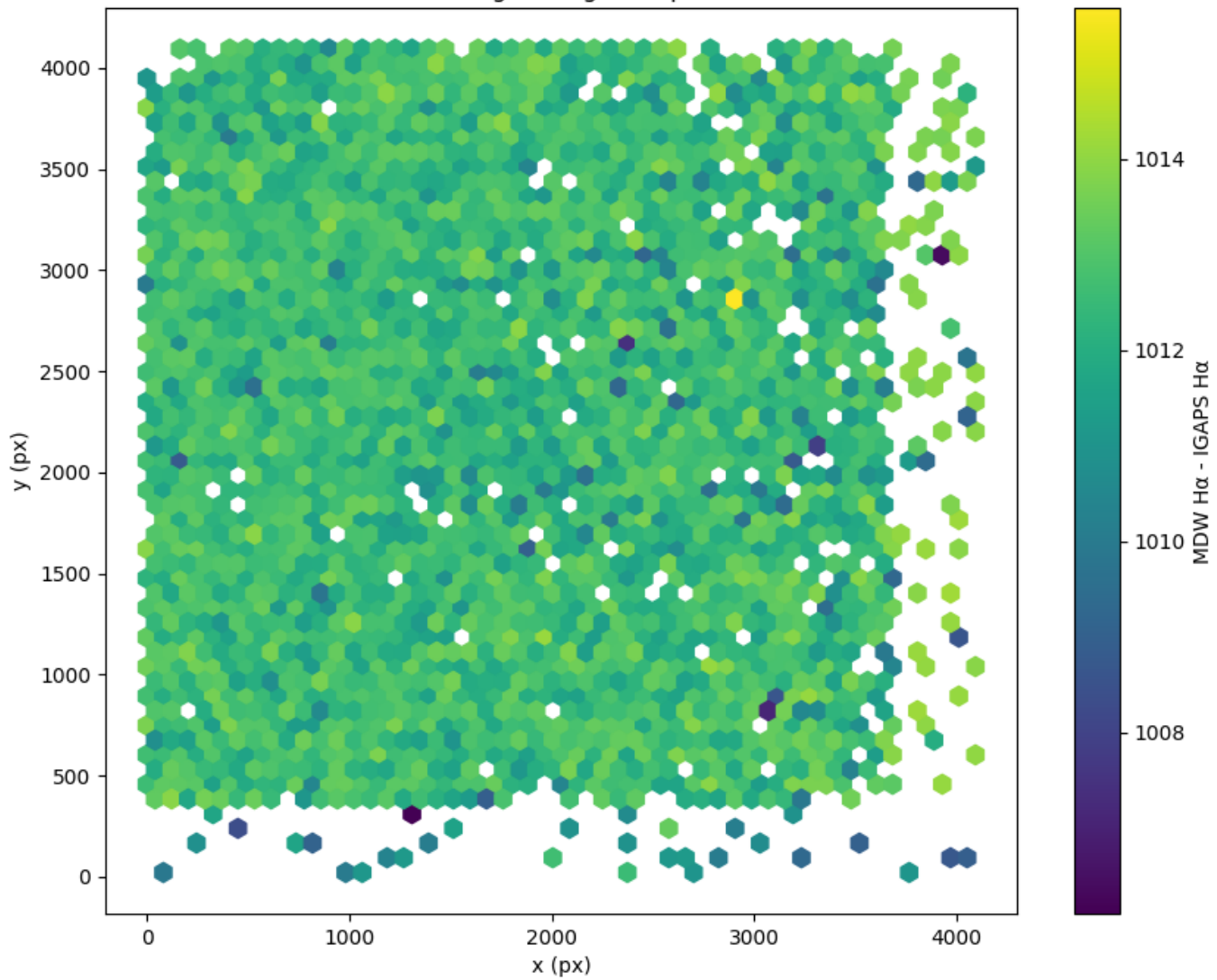
Field 2256 2D field distribution of (MDW H \alpha - Pan-STARRS r) Hexagon length: 82px
