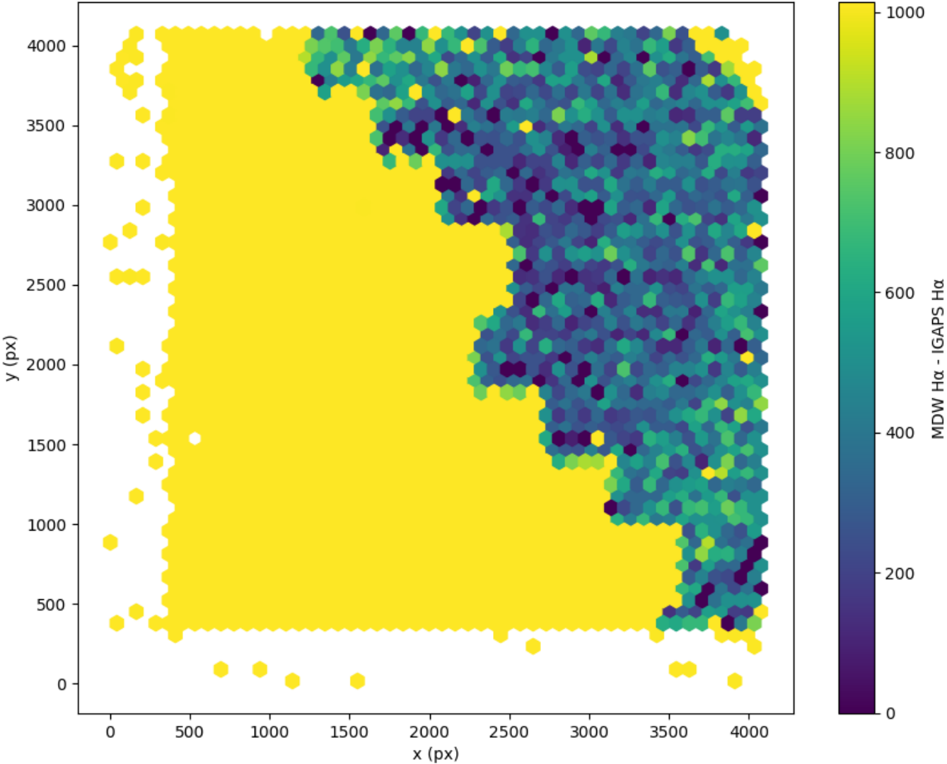
Field 0254 2D field distribution of (MDW H \alpha - Pan-STARRS r) Hexagon length: 81px
