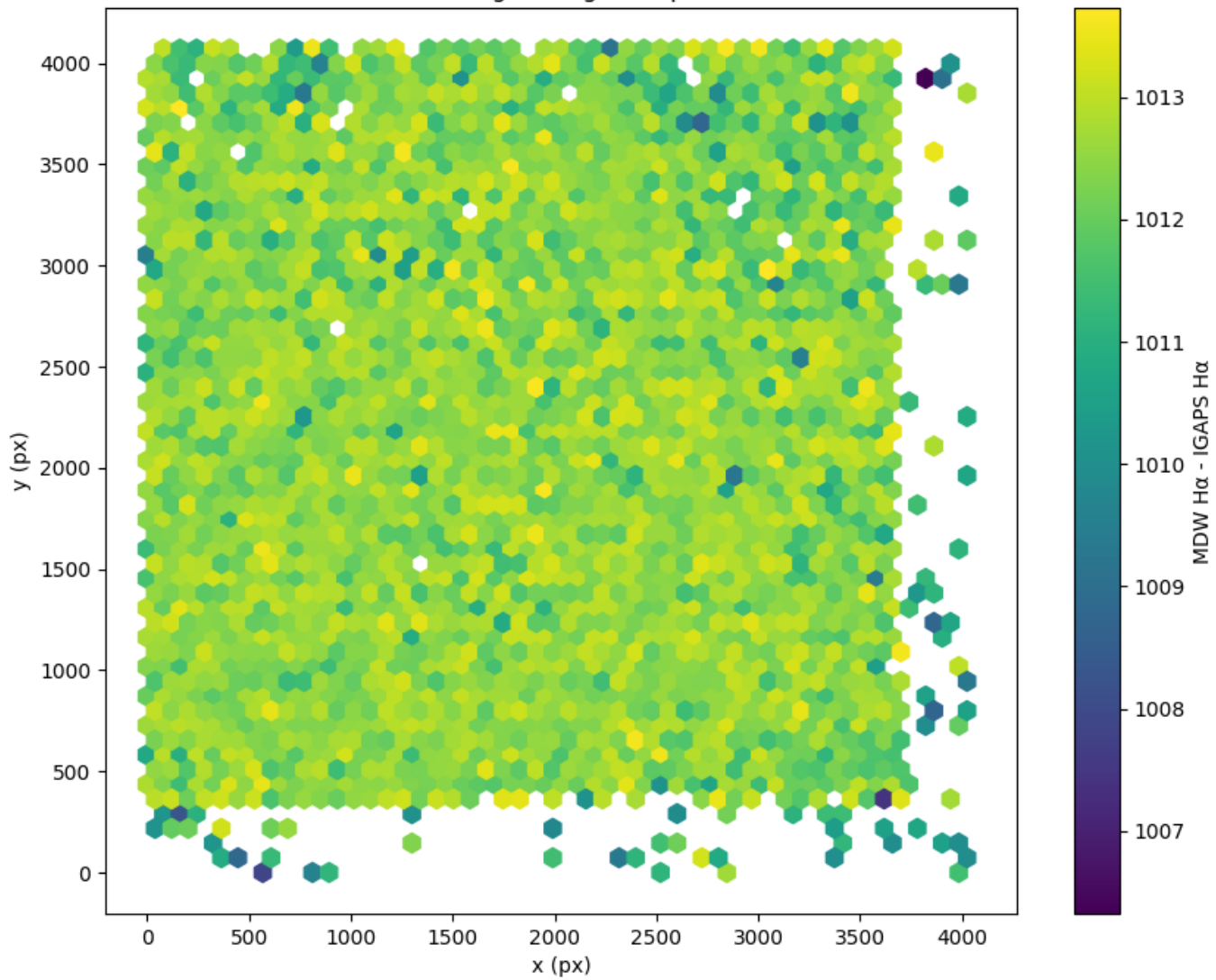
Field 2372 2D field distribution of (MDW H \alpha - Pan-STARRS r) Hexagon length: 81px
