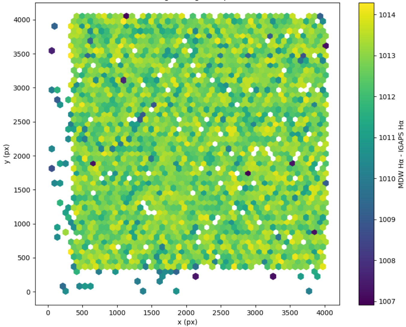
Field 0263 2D field distribution of (MDW H \alpha - Pan-STARRS r) Hexagon length: 80px
