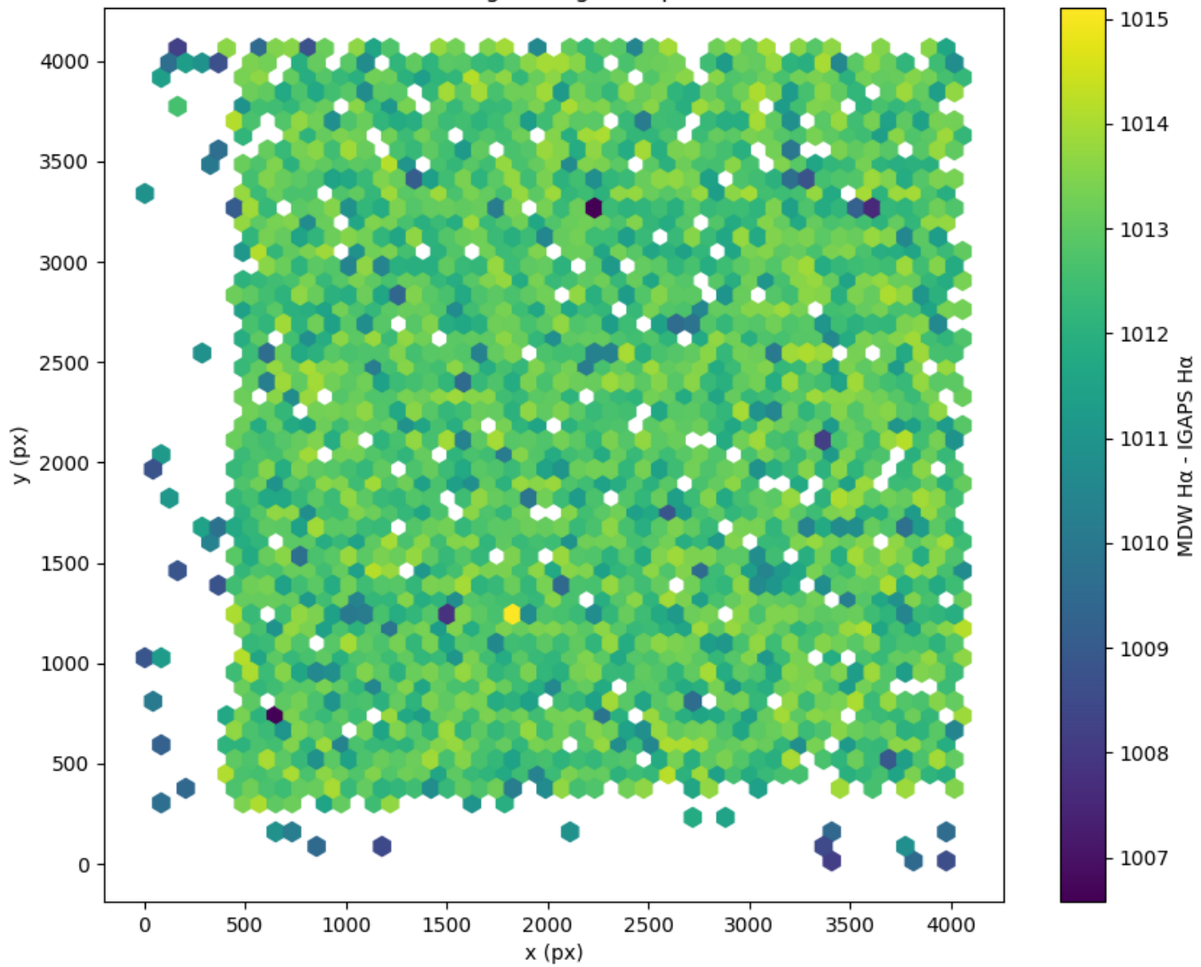
Field 0808 2D field distribution of (MDW H \alpha - Pan-STARRS r) Hexagon length: 81px
