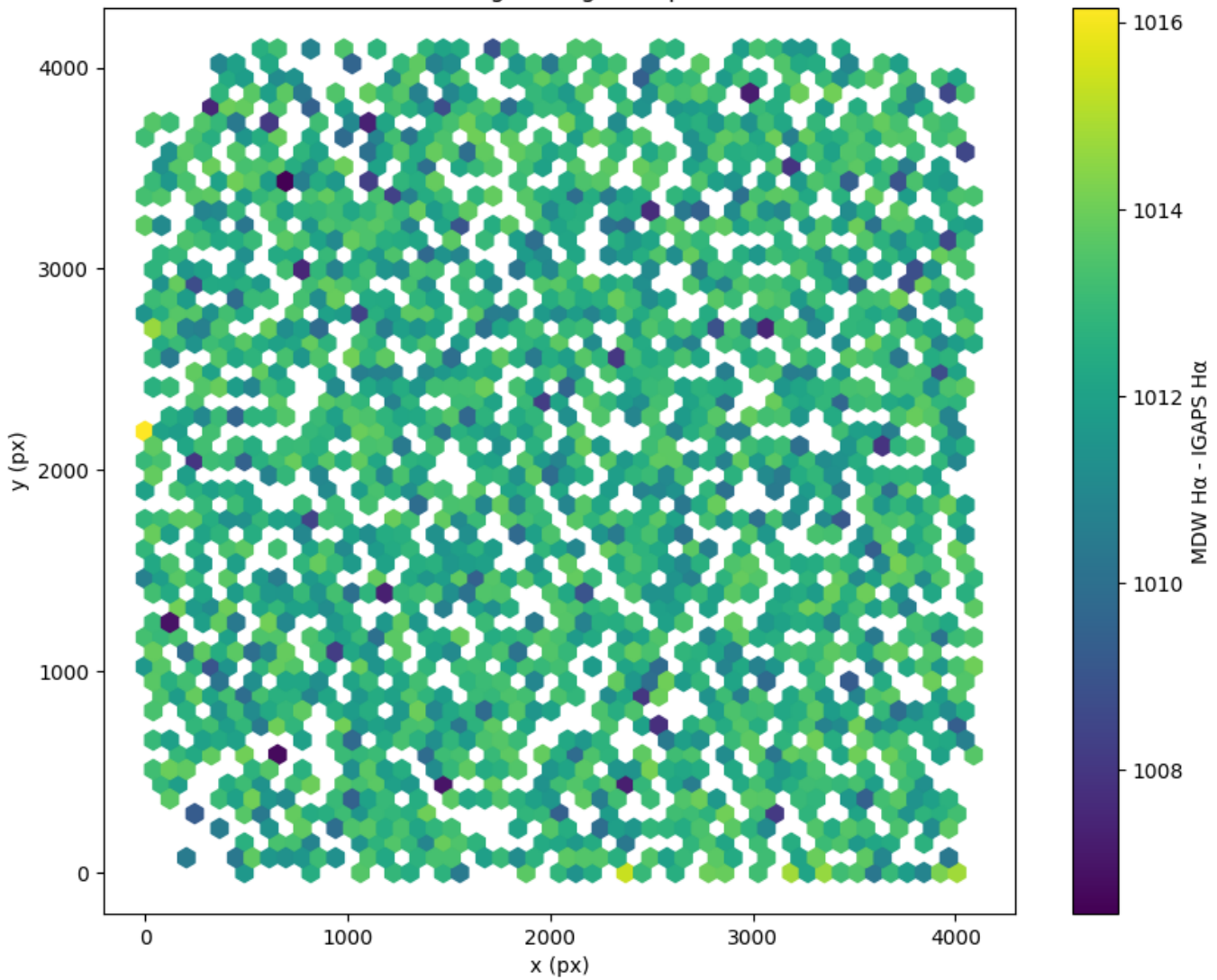
Field 2245 2D field distribution of (MDW H \alpha - Pan-STARRS r) Hexagon length: 82px
