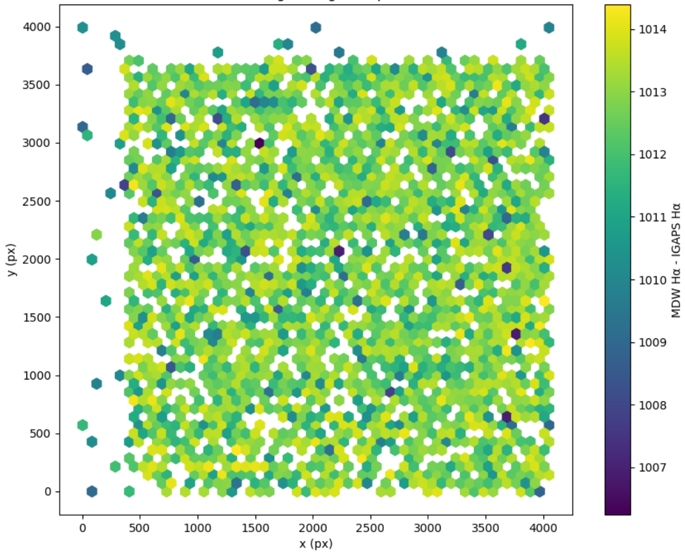
Field 2361 2D field distribution of (MDW H \alpha - Pan-STARRS r) Hexagon length: 81px
