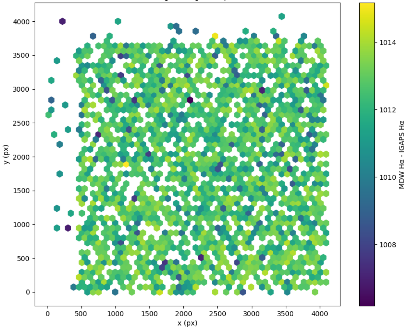
Field 2688 2D field distribution of (MDW H \alpha - Pan-STARRS r) Hexagon length: 81px
