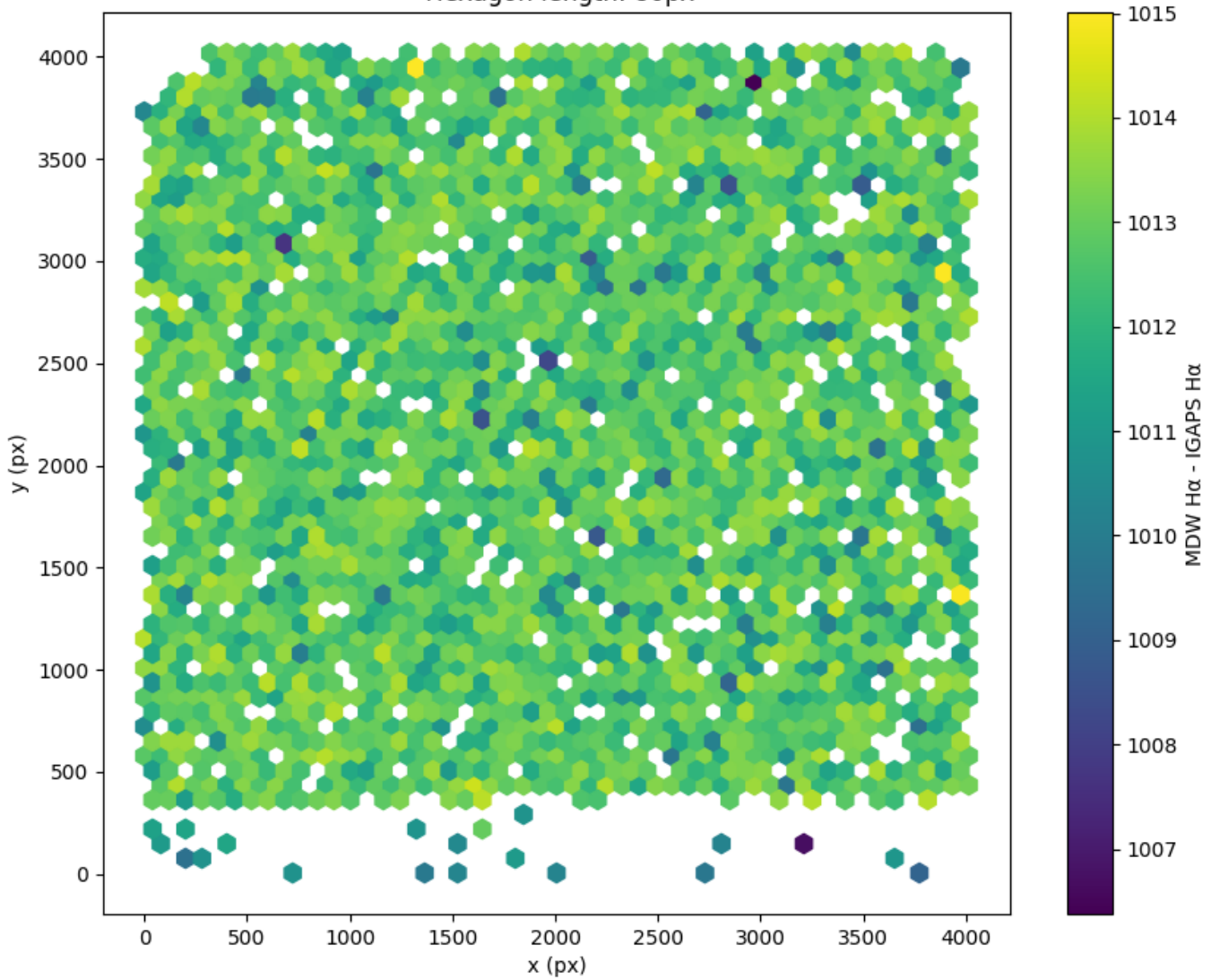
Field 0912 2D field distribution of (MDW H \alpha - Pan-STARRS r) Hexagon length: 80px
