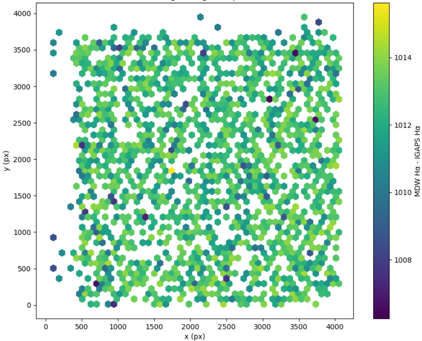
Field 2575 2D field distribution of (MDW H \alpha - Pan-STARRS r) Hexagon length: 80px
