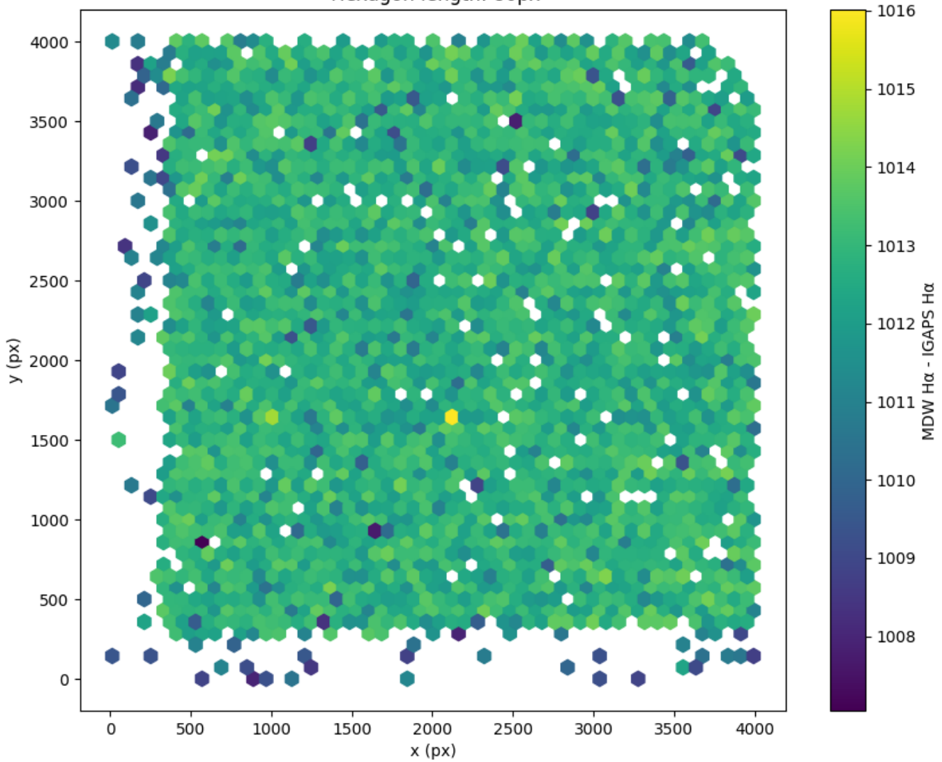
Field 0701 2D field distribution of (MDW H \alpha - Pan-STARRS r) Hexagon length: 80px
