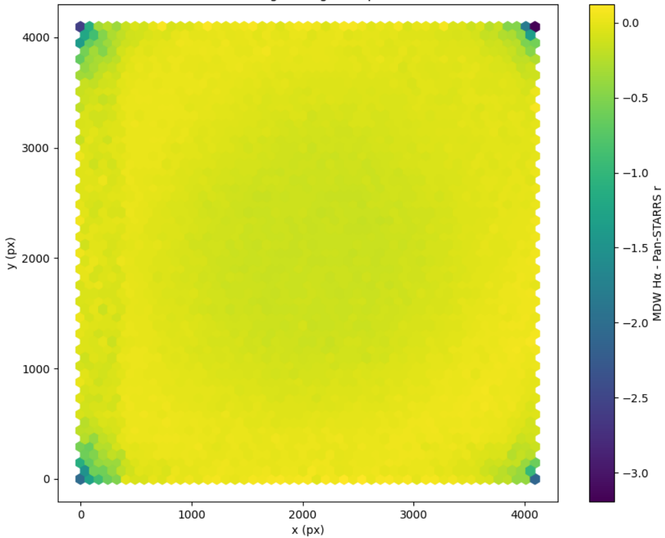
Across all fields 2D field distribution of (MDW H \alpha - Pan-STARRS r) Hexagon length: 82px
