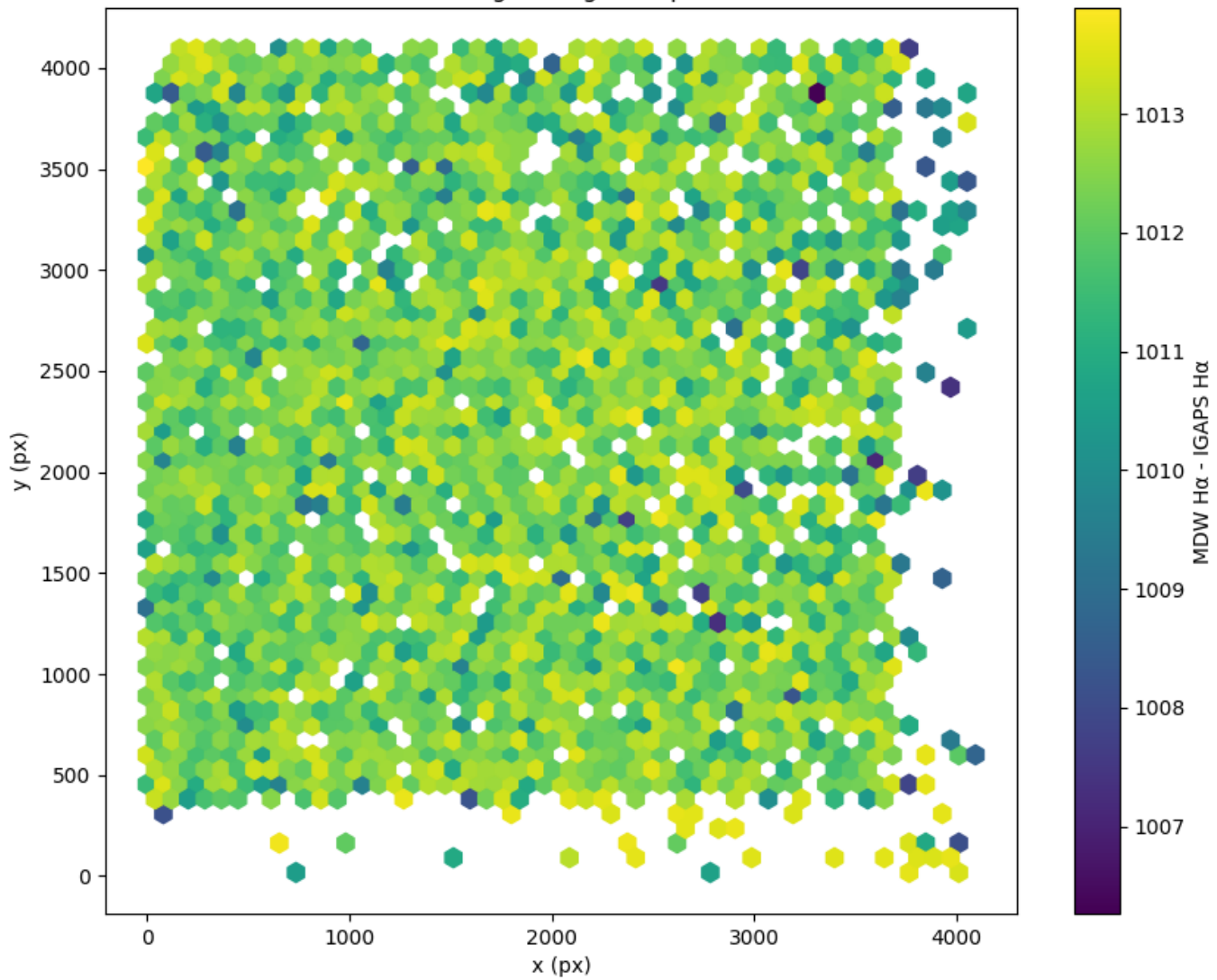
Field 2143 2D field distribution of (MDW H \alpha - Pan-STARRS r) Hexagon length: 82px
