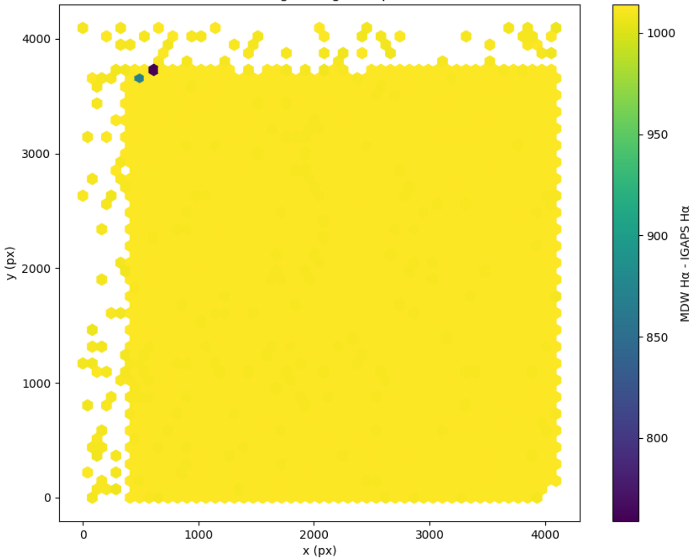
Field 2148 2D field distribution of (MDW H \alpha - Pan-STARRS r) Hexagon length: 82px
