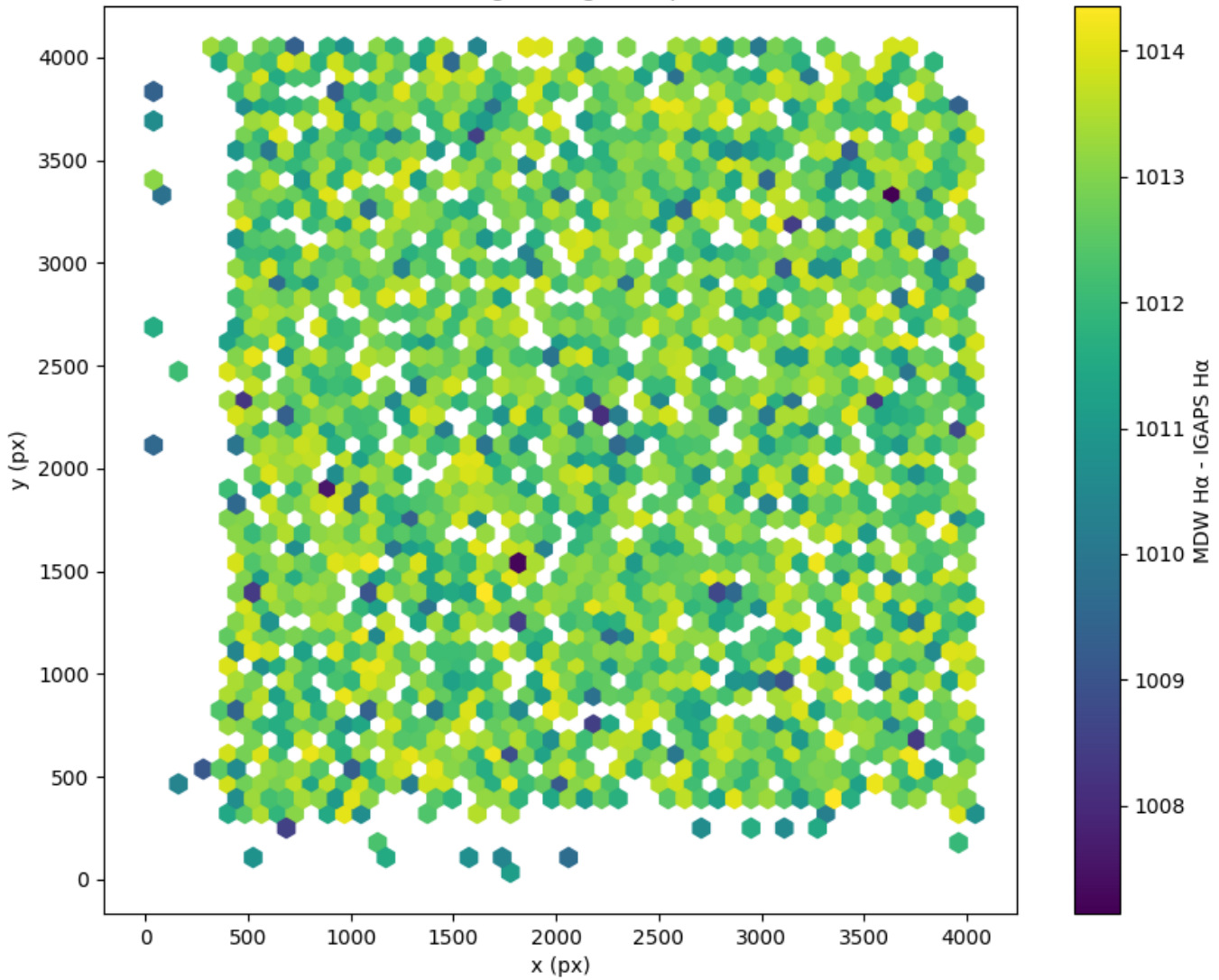
Field 0705 2D field distribution of (MDW H \alpha - Pan-STARRS r) Hexagon length: 81px
