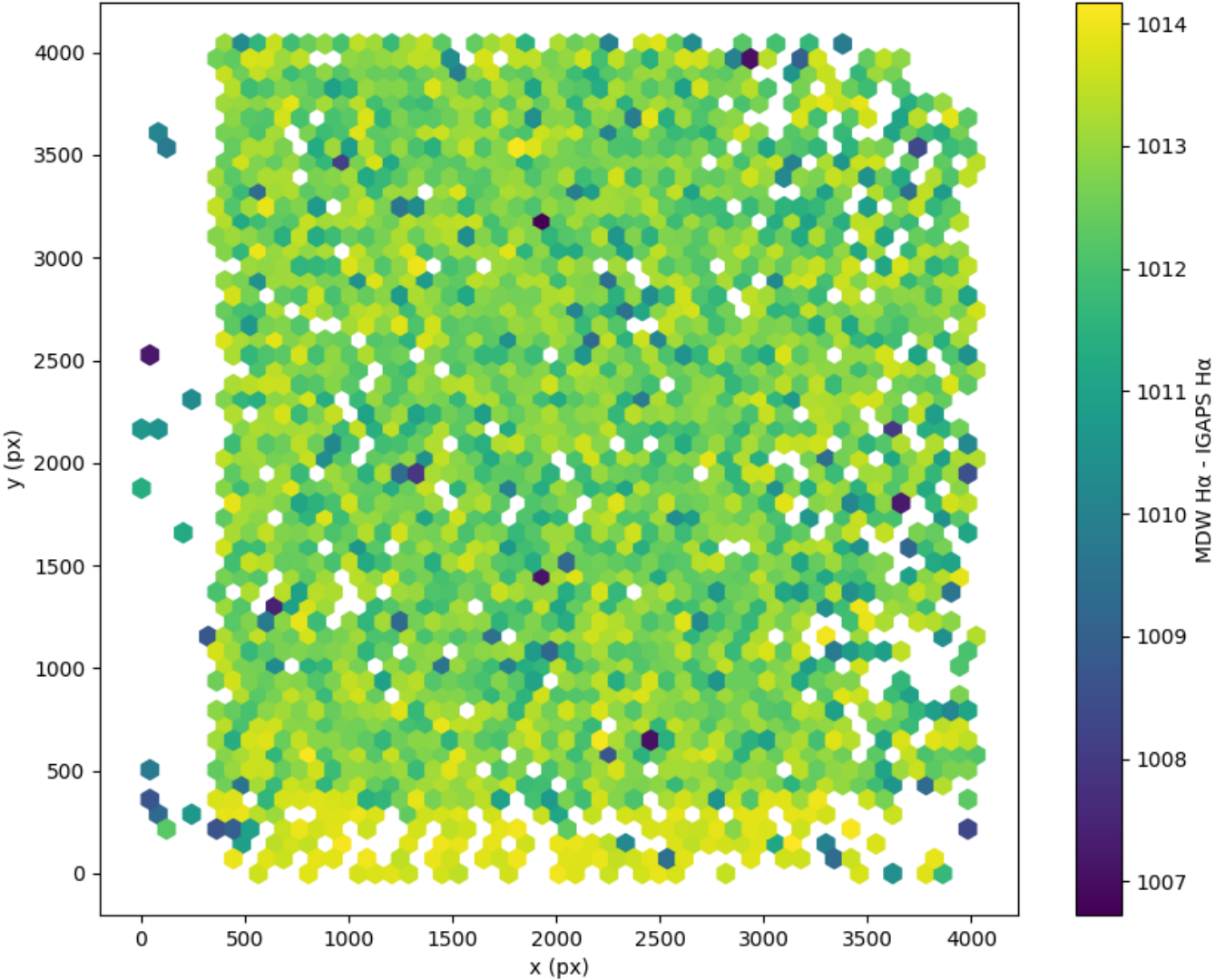
Field 0140 2D field distribution of (MDW H \alpha - Pan-STARRS r) Hexagon length: 80px
