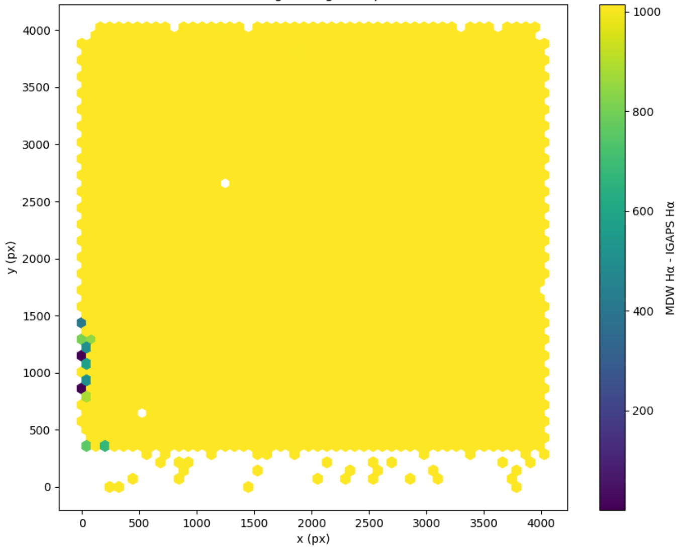
Field 0697 2D field distribution of (MDW H \alpha - Pan-STARRS r) Hexagon length: 81px
