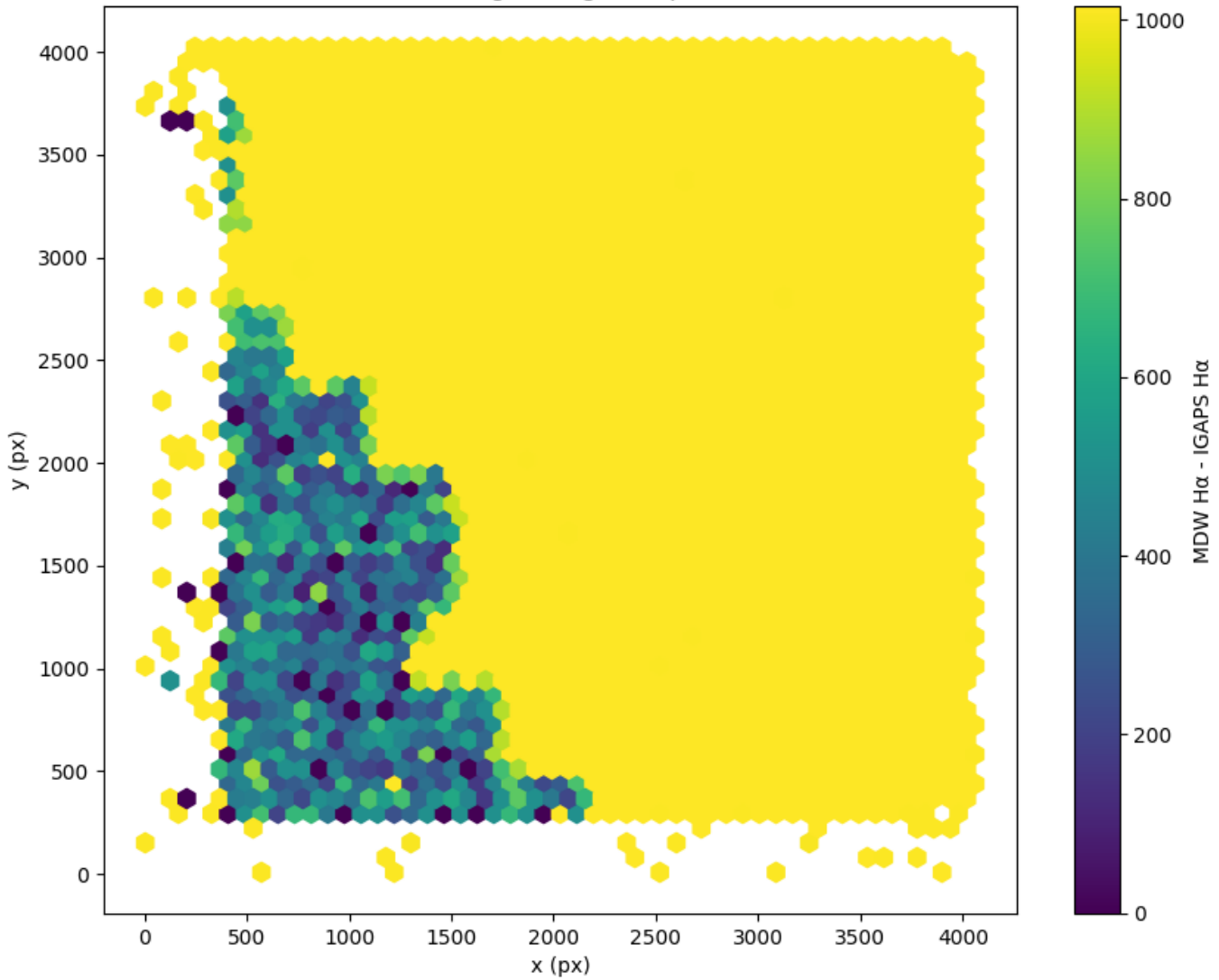
Field 0258 2D field distribution of (MDW H \alpha - Pan-STARRS r) Hexagon length: 81px
