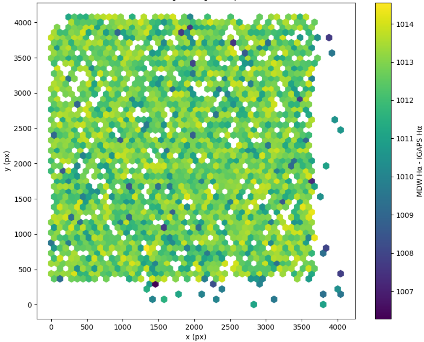
Field 2363 2D field distribution of (MDW H \alpha - Pan-STARRS r) Hexagon length: 81px
