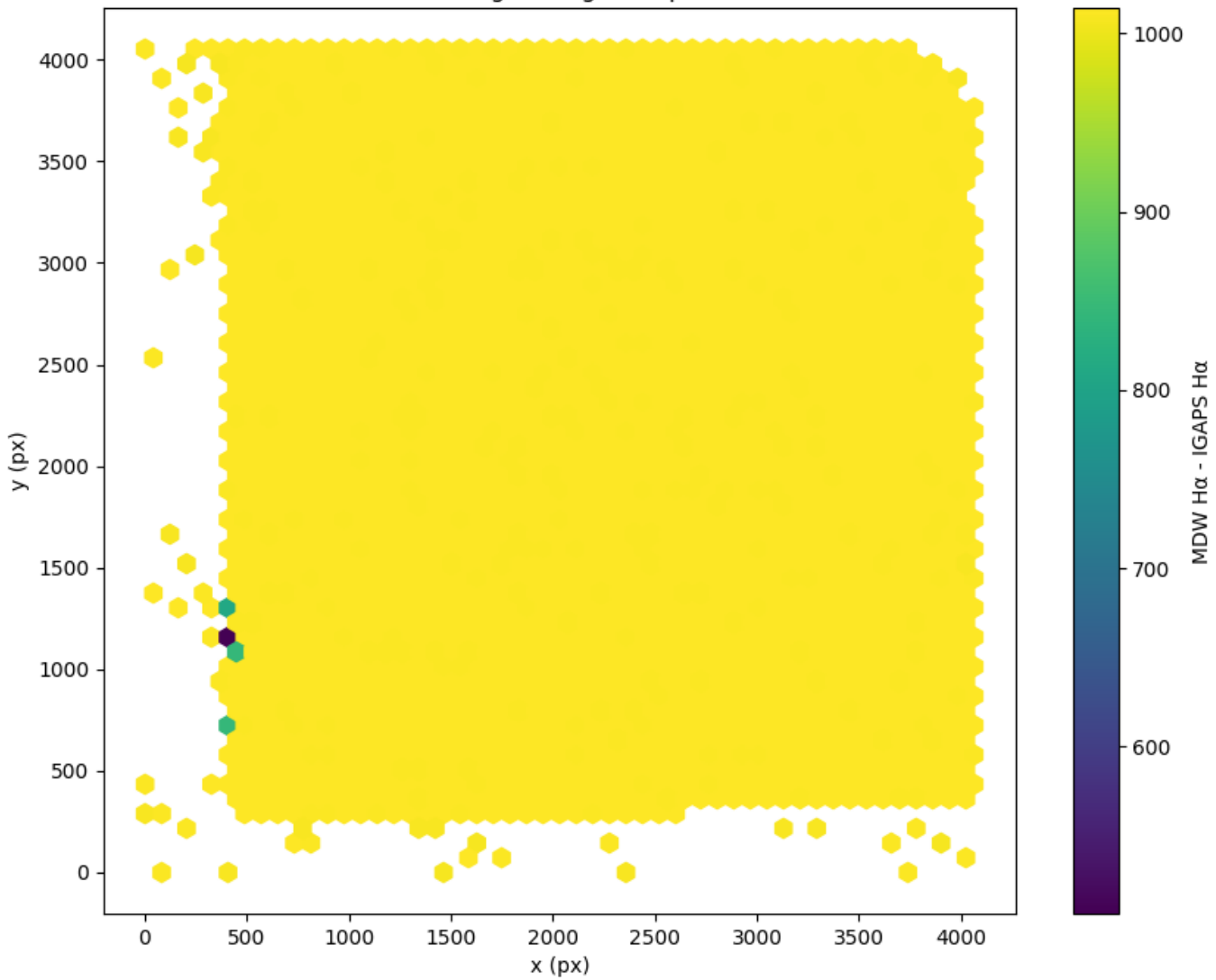
Field 0589 2D field distribution of (MDW H \alpha - Pan-STARRS r) Hexagon length: 81px
