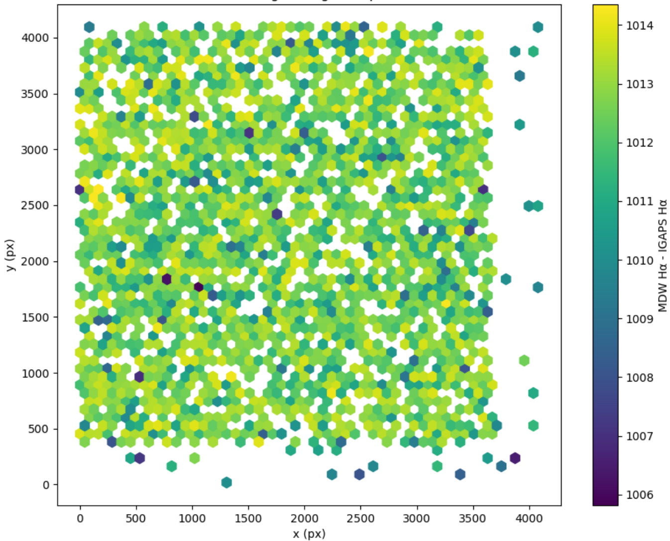
Field 2247 2D field distribution of (MDW H \alpha - Pan-STARRS r) Hexagon length: 82px
