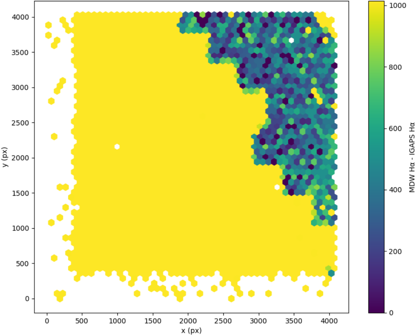
Field 0365 2D field distribution of (MDW H \alpha - Pan-STARRS r) Hexagon length: 81px
