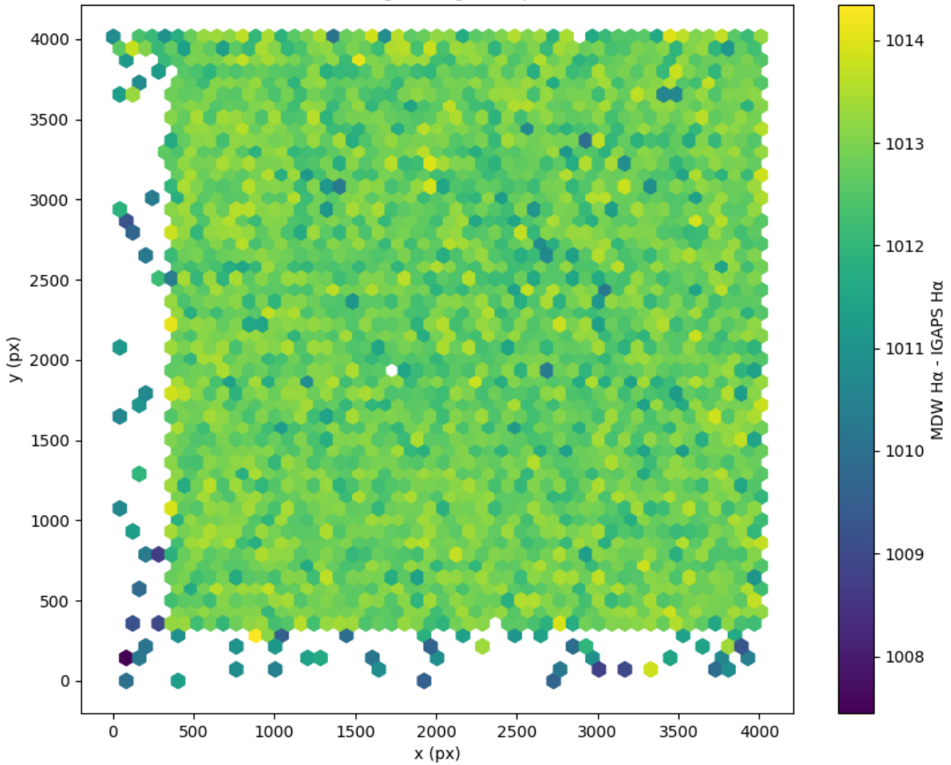
Field 0147 2D field distribution of (MDW H \alpha - Pan-STARRS r) Hexagon length: 80px
