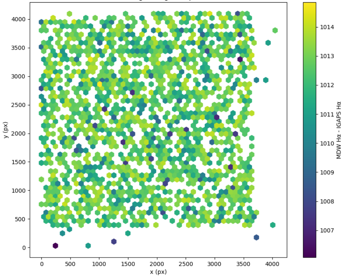
Field 2466 2D field distribution of (MDW H \alpha - Pan-STARRS r) Hexagon length: 81px
