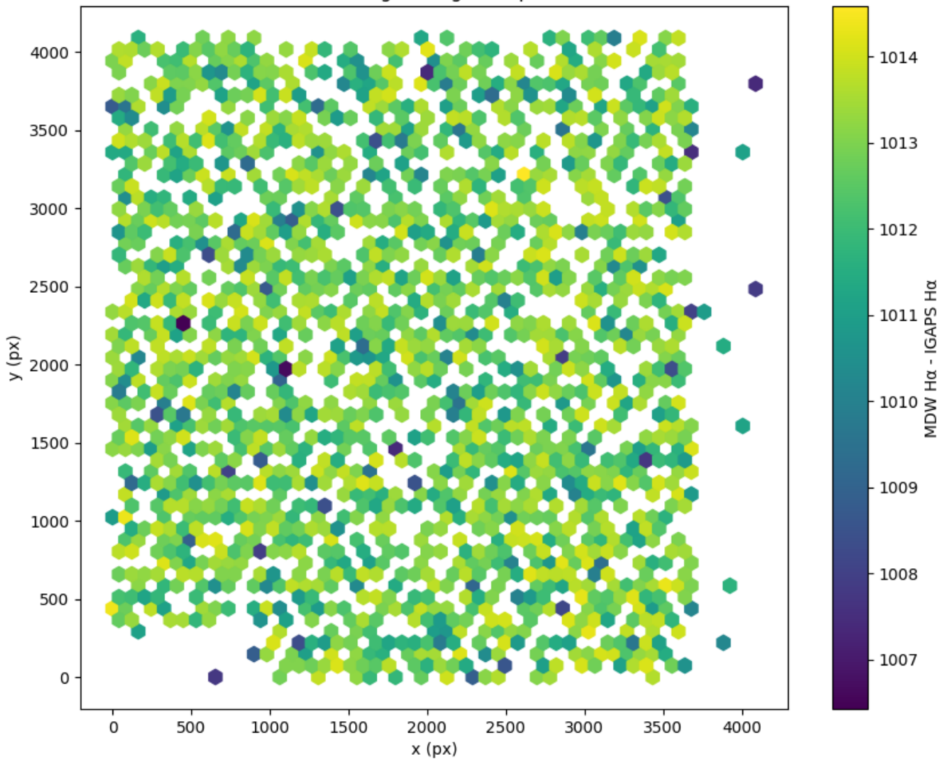
Field 2356 2D field distribution of (MDW H \alpha - Pan-STARRS r) Hexagon length: 82px
