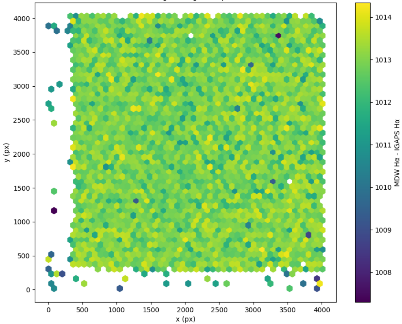
Field 0698 2D field distribution of (MDW H \alpha - Pan-STARRS r) Hexagon length: 80px
