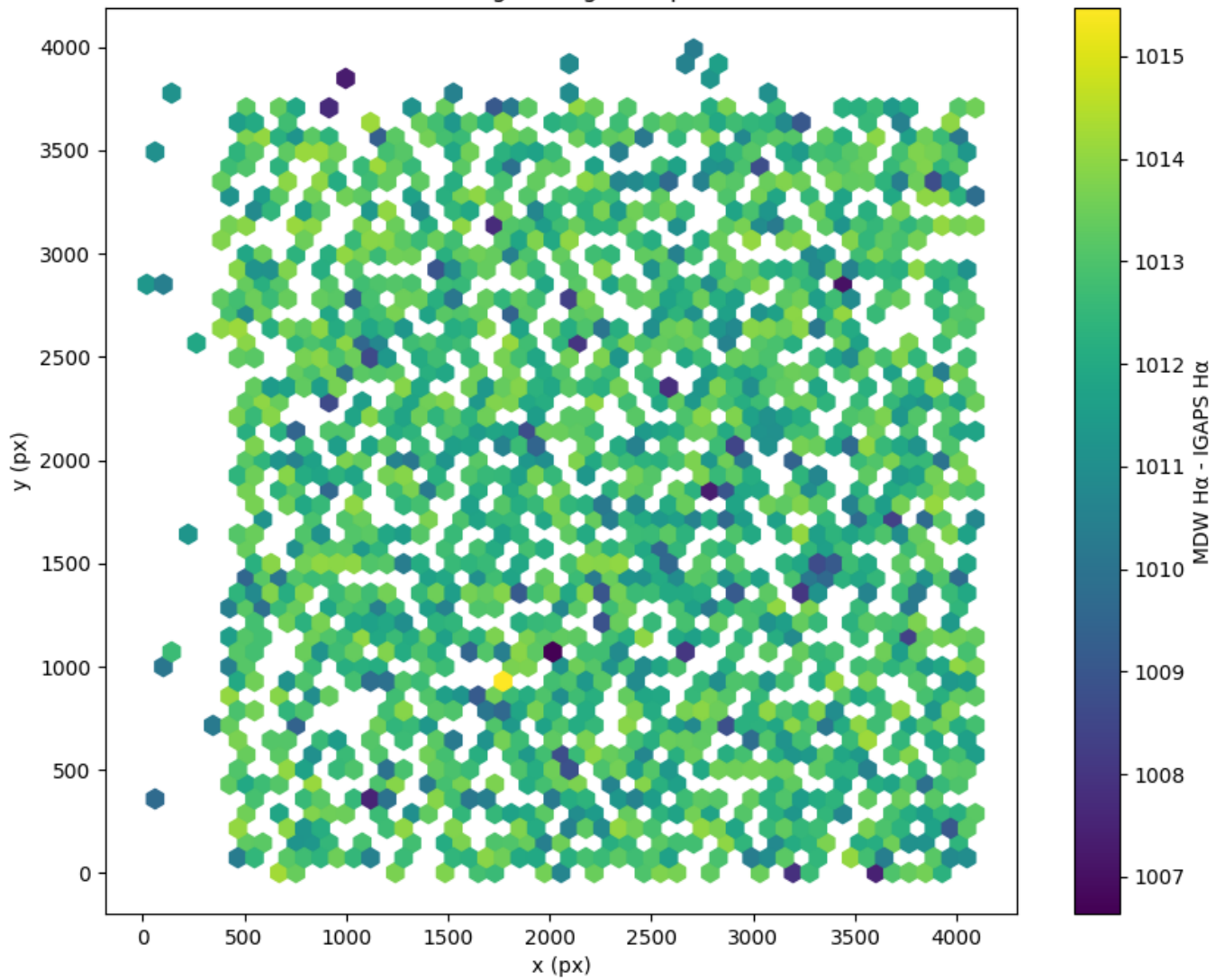
Field 2357 2D field distribution of (MDW H \alpha - Pan-STARRS r) Hexagon length: 81px
