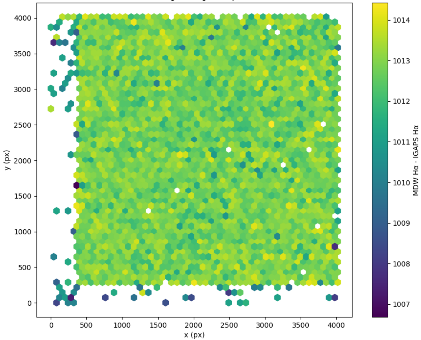
Field 0481 2D field distribution of (MDW H \alpha - Pan-STARRS r) Hexagon length: 80px
