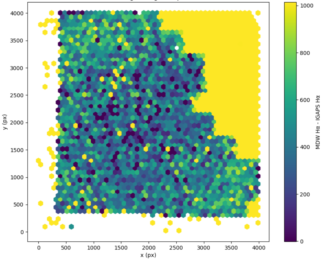
Field 0588 2D field distribution of (MDW H \alpha - Pan-STARRS r) Hexagon length: 80px
