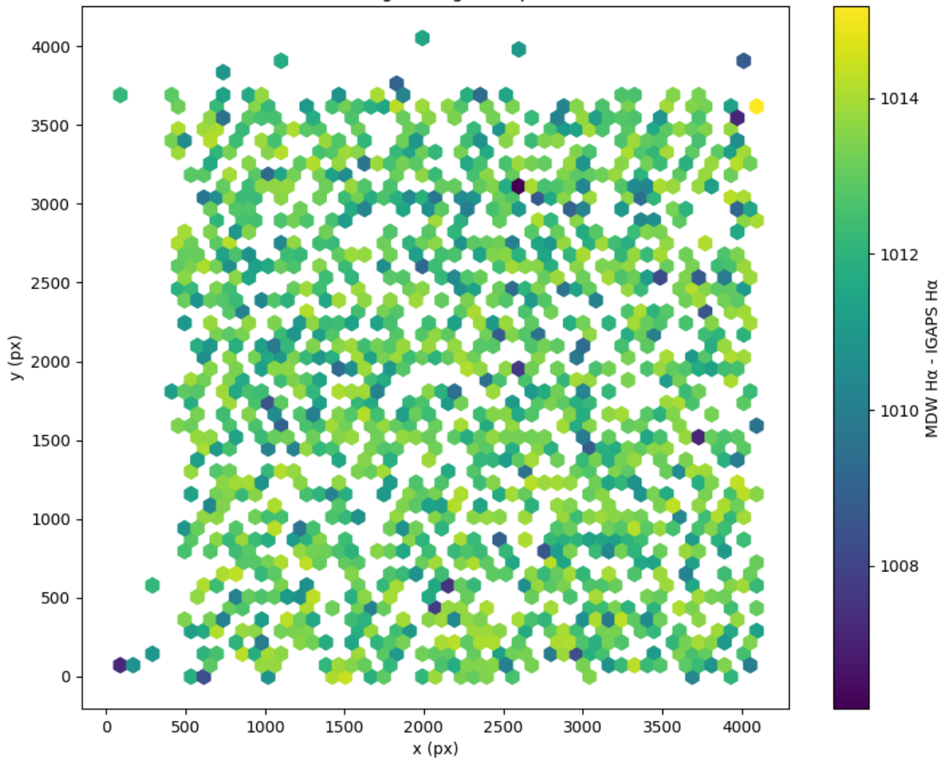
Field 2788 2D field distribution of (MDW H \alpha - Pan-STARRS r) Hexagon length: 81px
