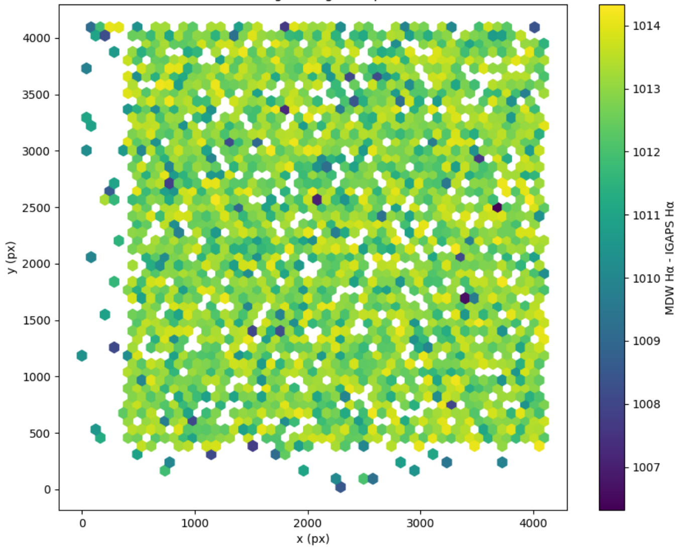
Field 0377 2D field distribution of (MDW H \alpha - Pan-STARRS r) Hexagon length: 82px
