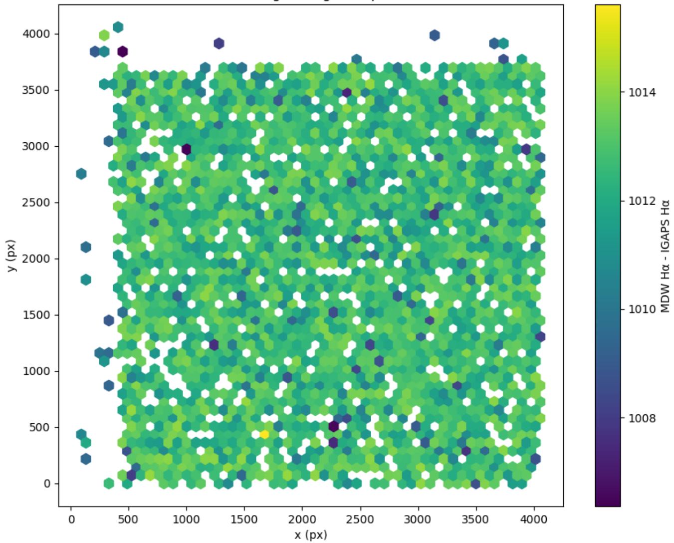
Field 2693 2D field distribution of (MDW H \alpha - Pan-STARRS r) Hexagon length: 79px
