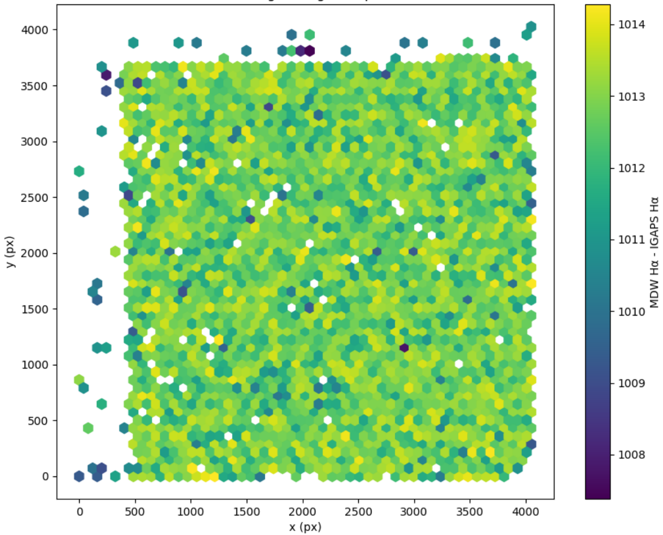
Field 2588 2D field distribution of (MDW H \alpha - Pan-STARRS r) Hexagon length: 81px
