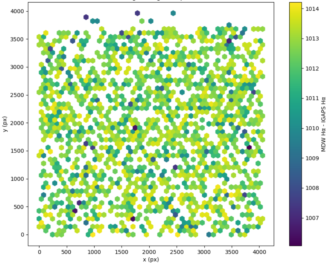
Field 2787 2D field distribution of (MDW H \alpha - Pan-STARRS r) Hexagon length: 81px
