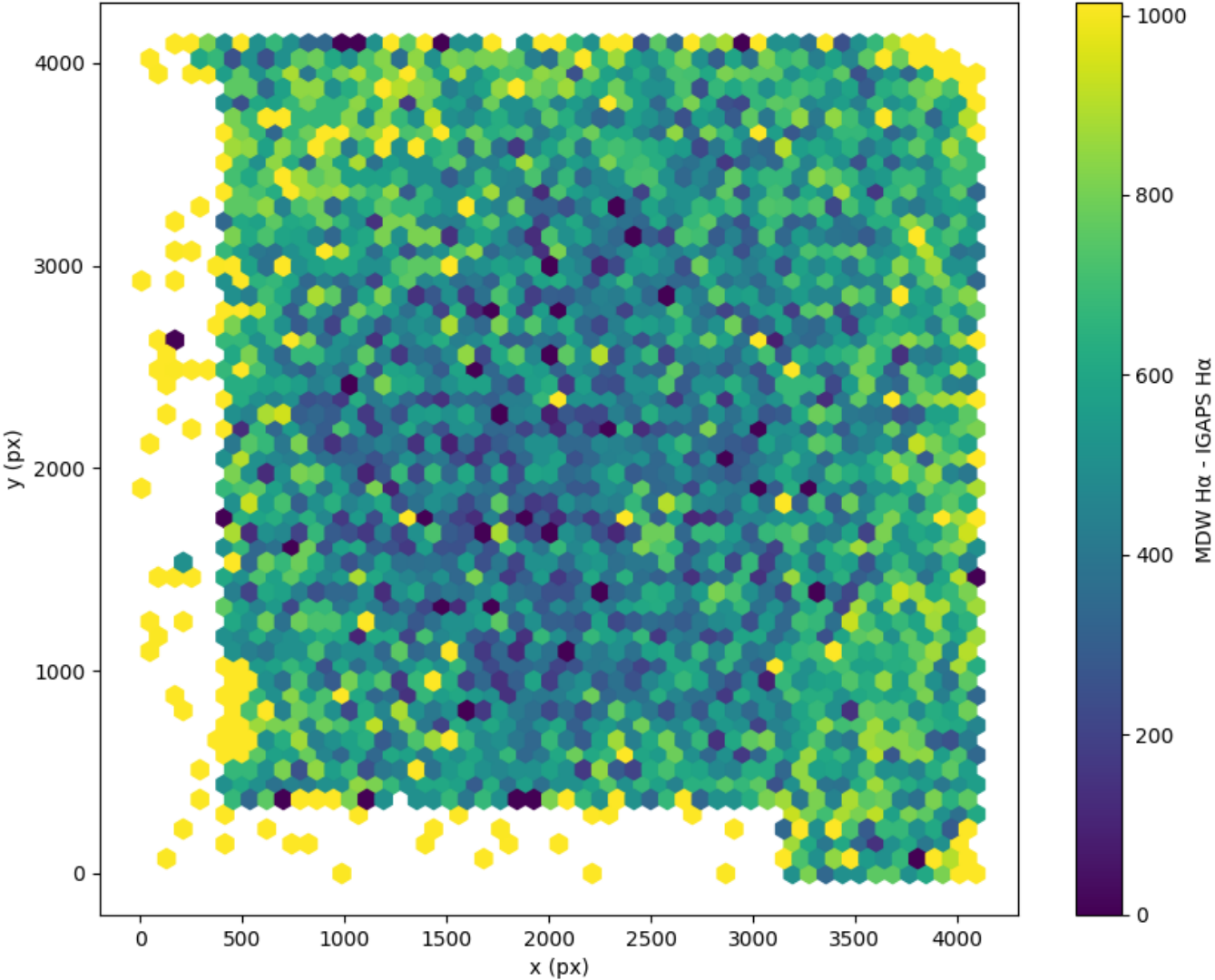
Field 0366 2D field distribution of (MDW H \alpha - Pan-STARRS r) Hexagon length: 82px
