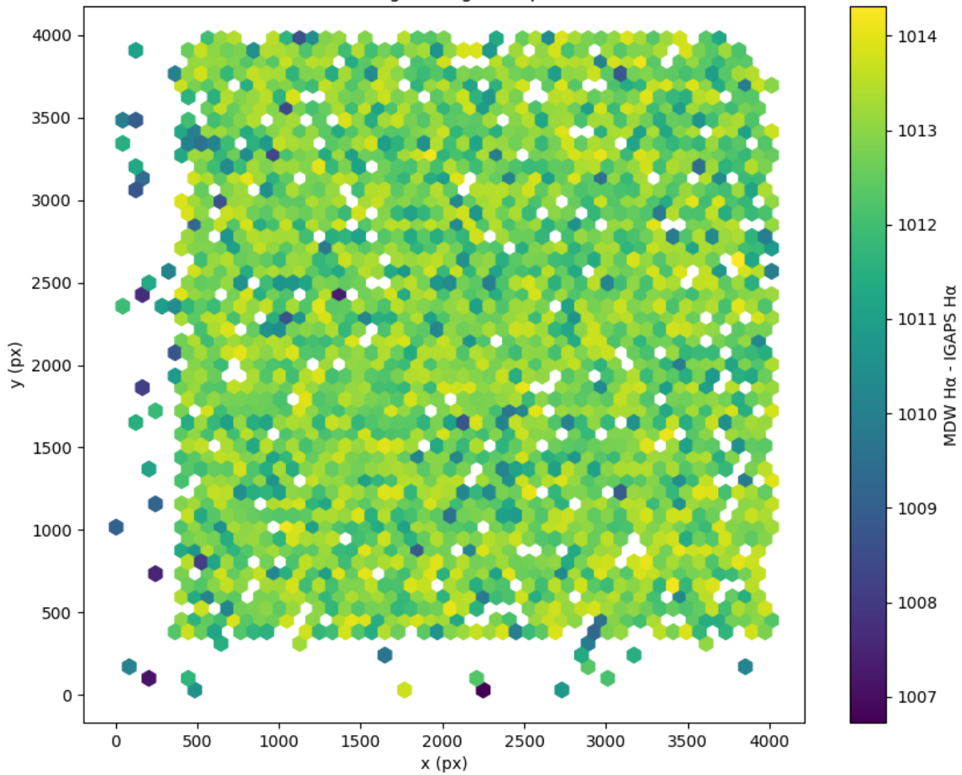
Field 0703 2D field distribution of (MDW H \alpha - Pan-STARRS r) Hexagon length: 80px
