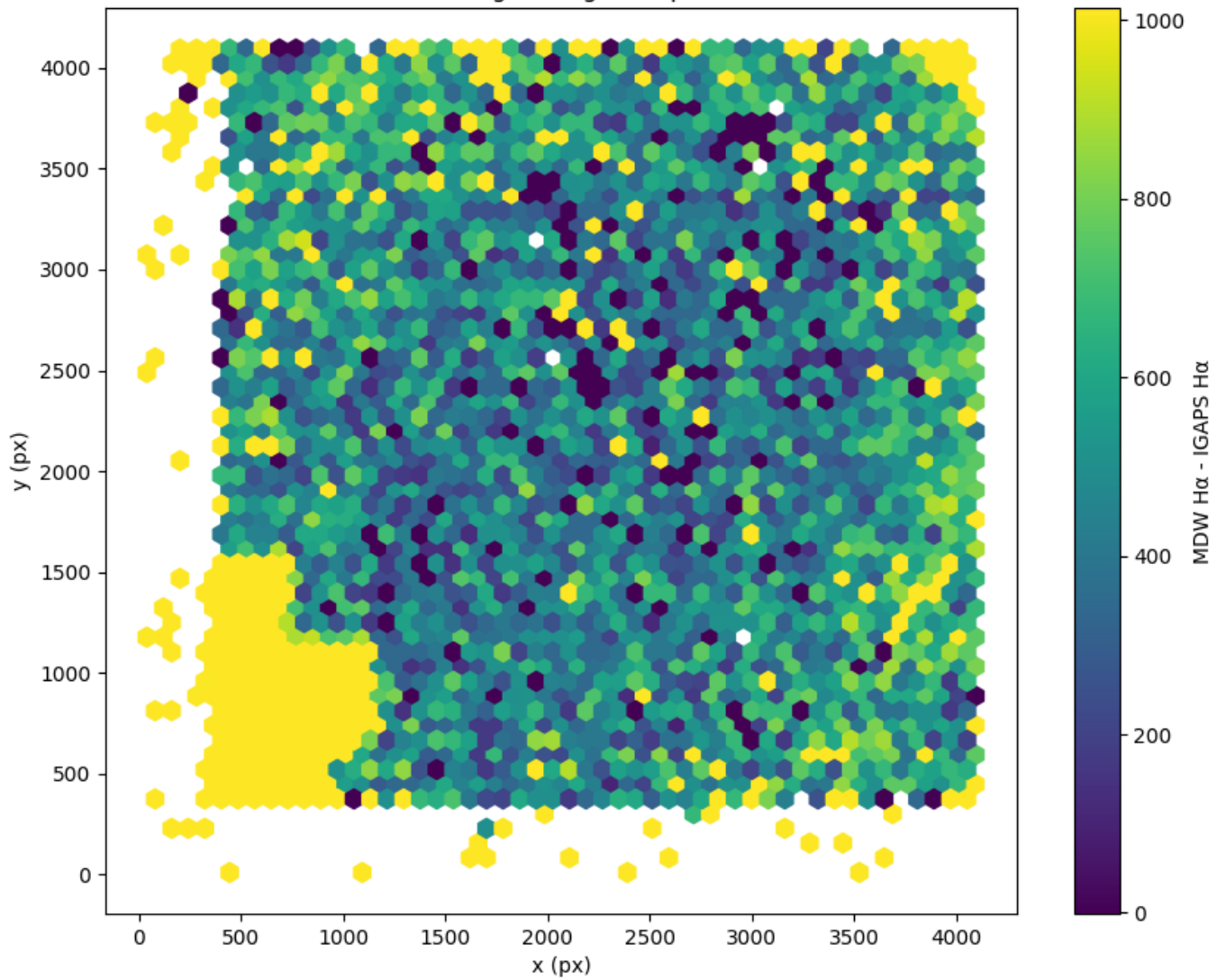
Field 0476 2D field distribution of (MDW H \alpha - Pan-STARRS r) Hexagon length: 81px
