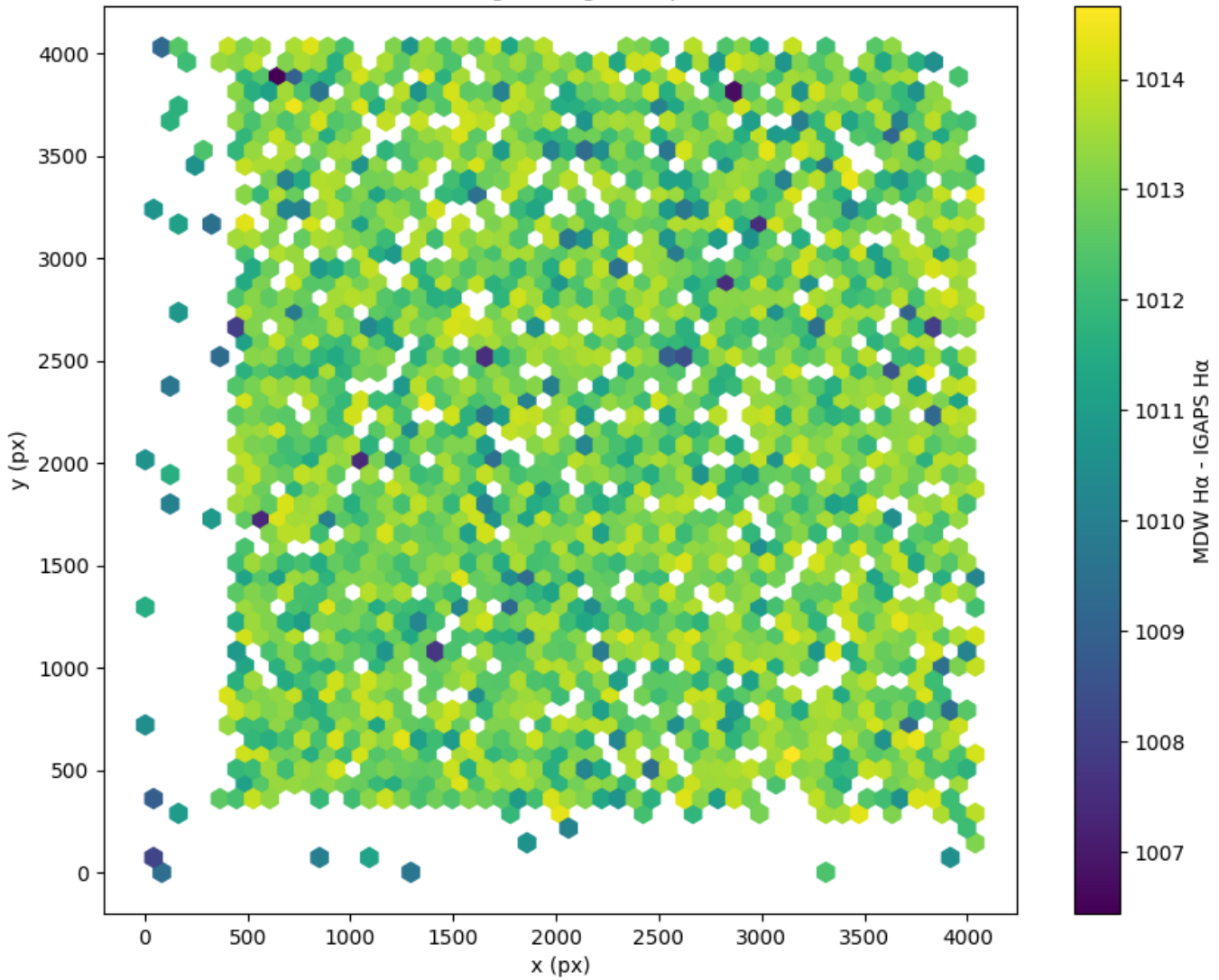
Field 0914 2D field distribution of (MDW H \alpha - Pan-STARRS r) Hexagon length: 81px
