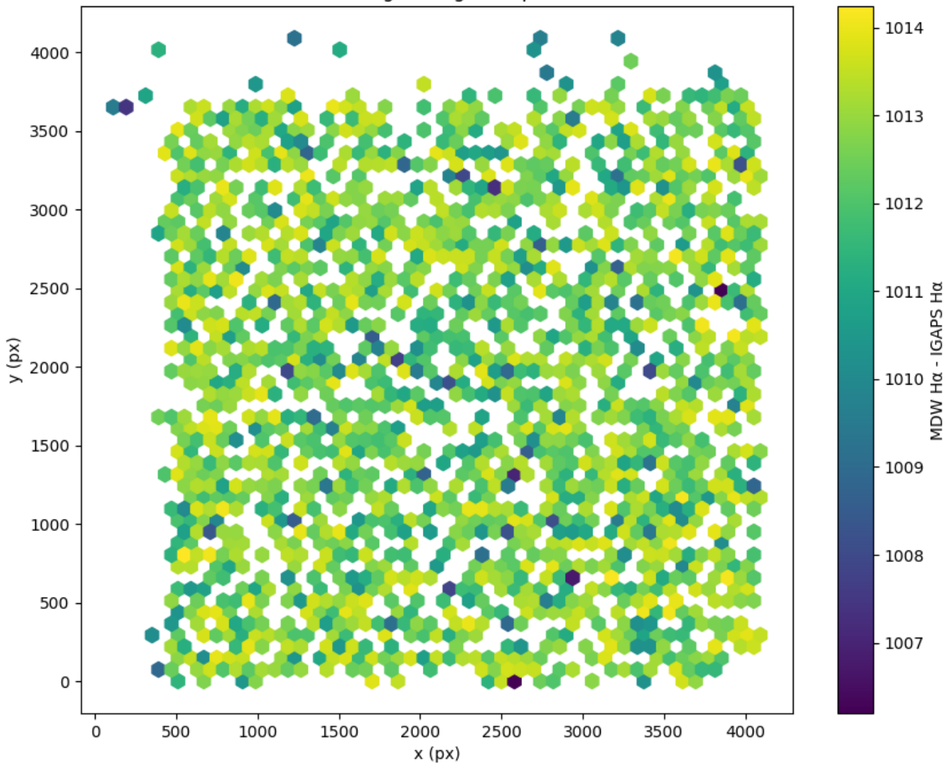
Field 2578 2D field distribution of (MDW H \alpha - Pan-STARRS r) Hexagon length: 80px
