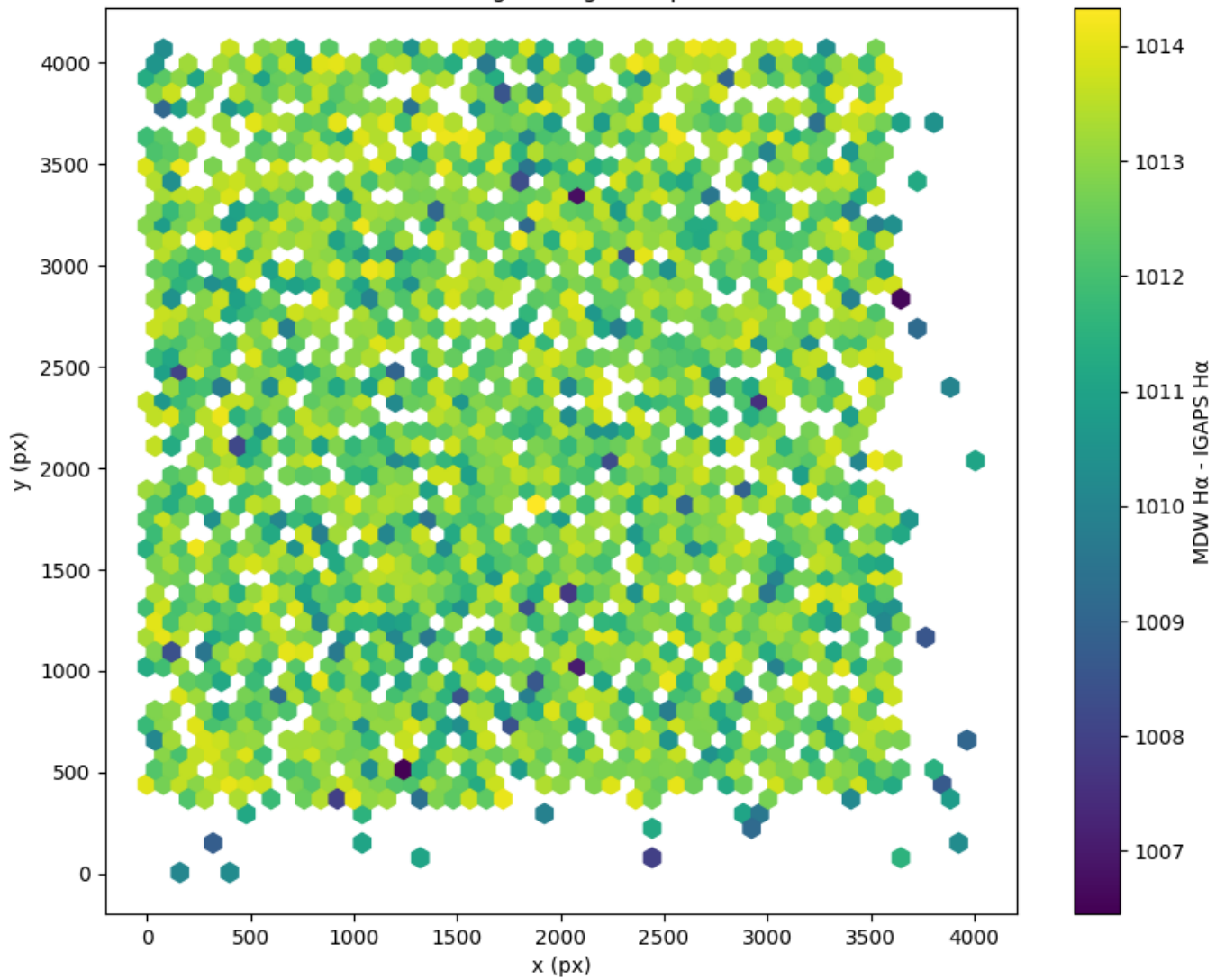
Field 2798 2D field distribution of (MDW H \alpha - Pan-STARRS r) Hexagon length: 80px
