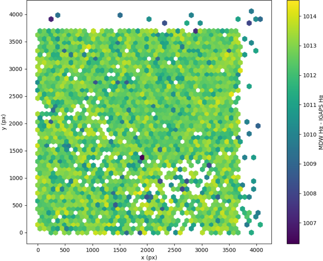
Field 0250 2D field distribution of (MDW H \alpha - Pan-STARRS r) Hexagon length: 81px
