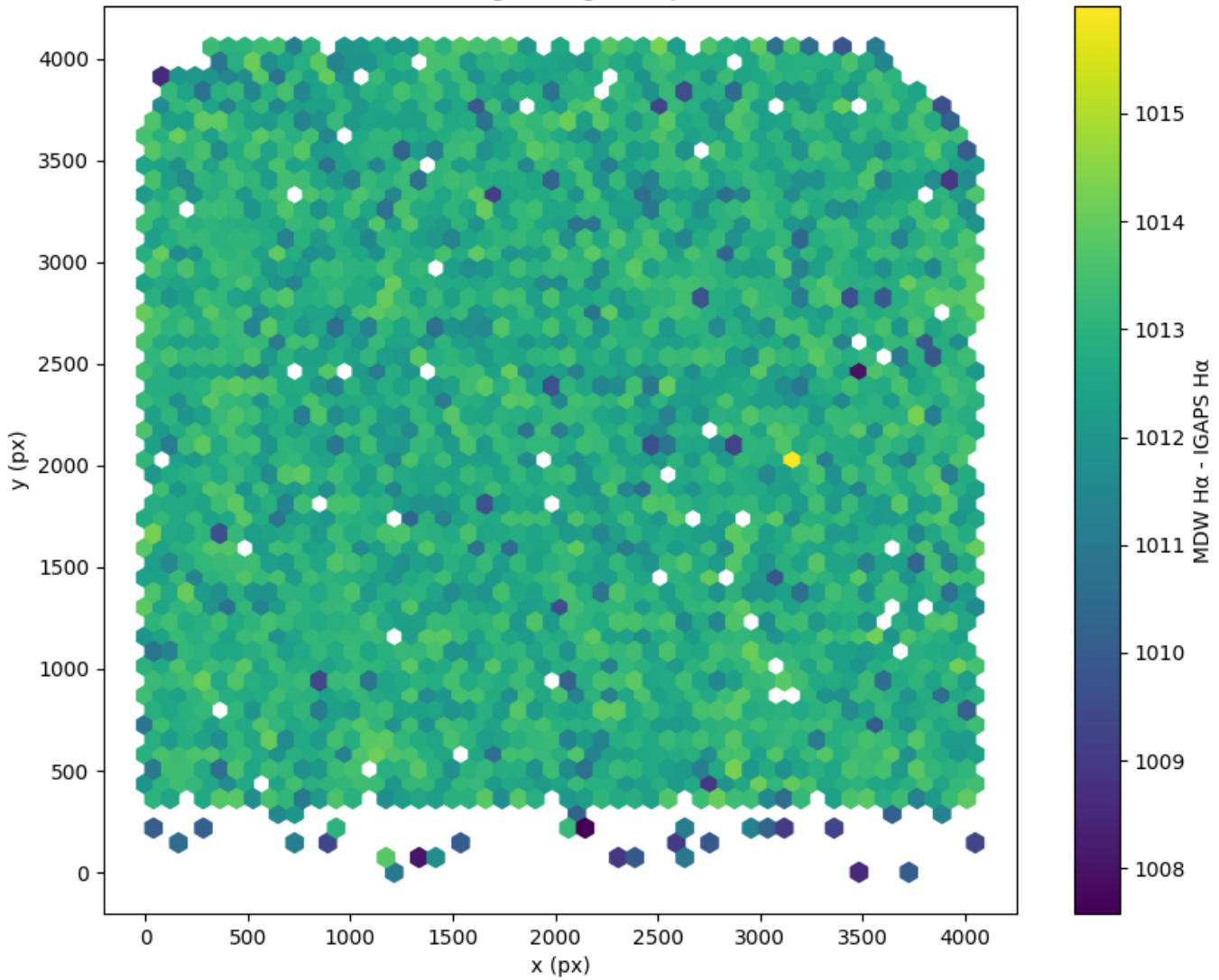
Field 0806 2D field distribution of (MDW H \alpha - Pan-STARRS r) Hexagon length: 81px
