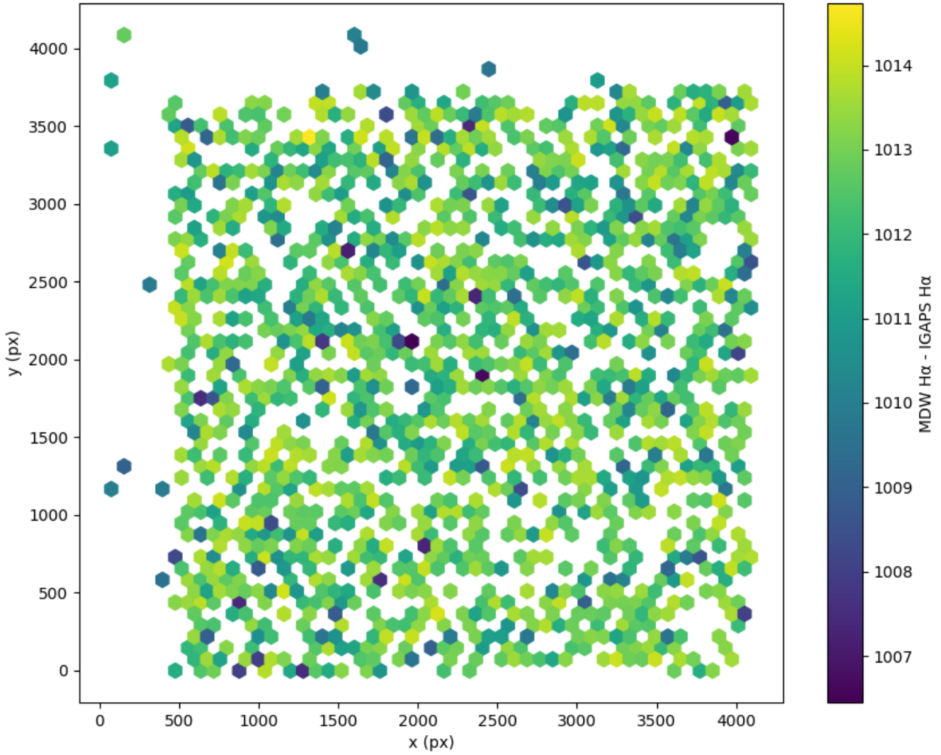
Field 2683 2D field distribution of (MDW H \alpha - Pan-STARRS r) Hexagon length: 80px
