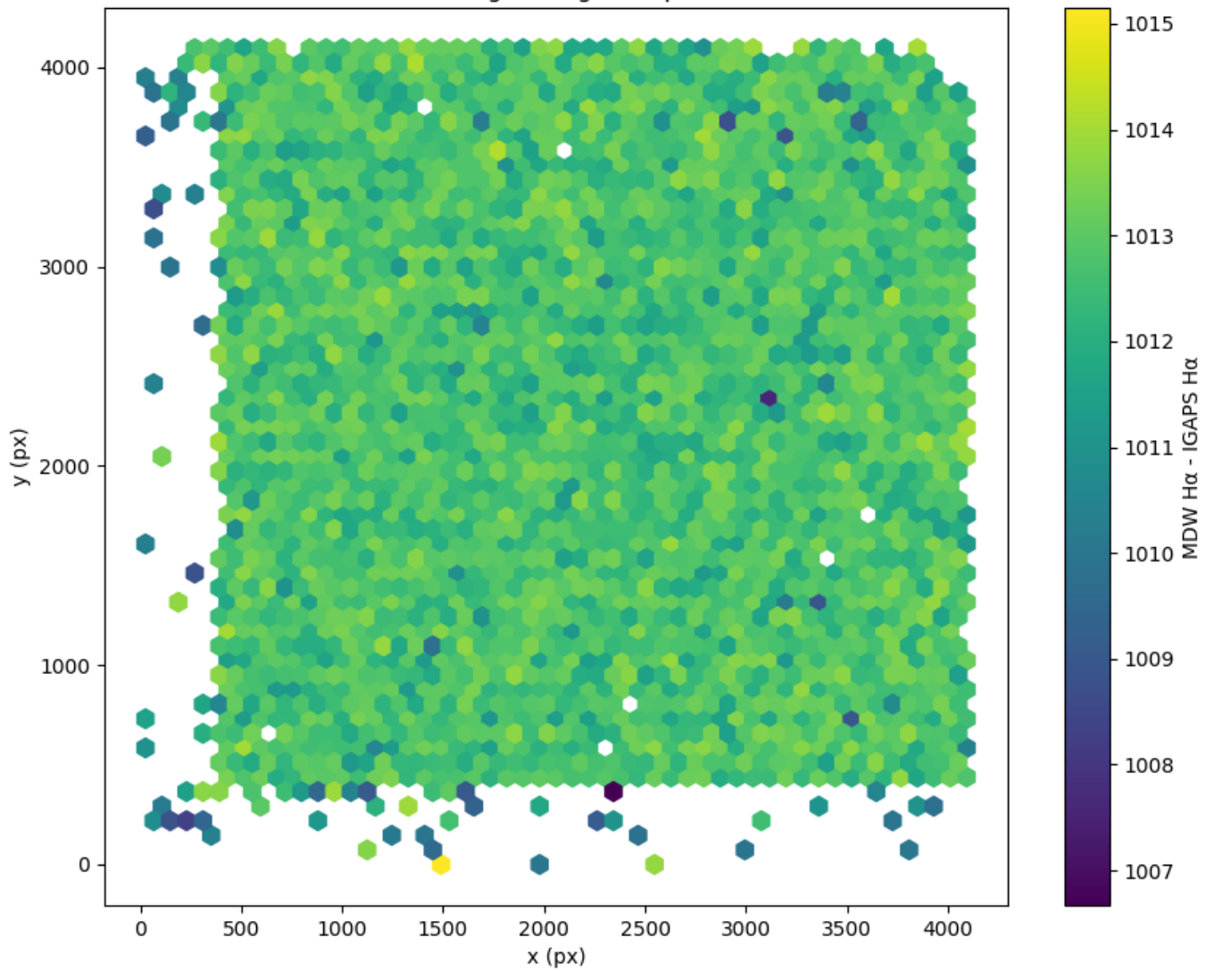
Field 0260 2D field distribution of (MDW H \alpha - Pan-STARRS r) Hexagon length: 81px
