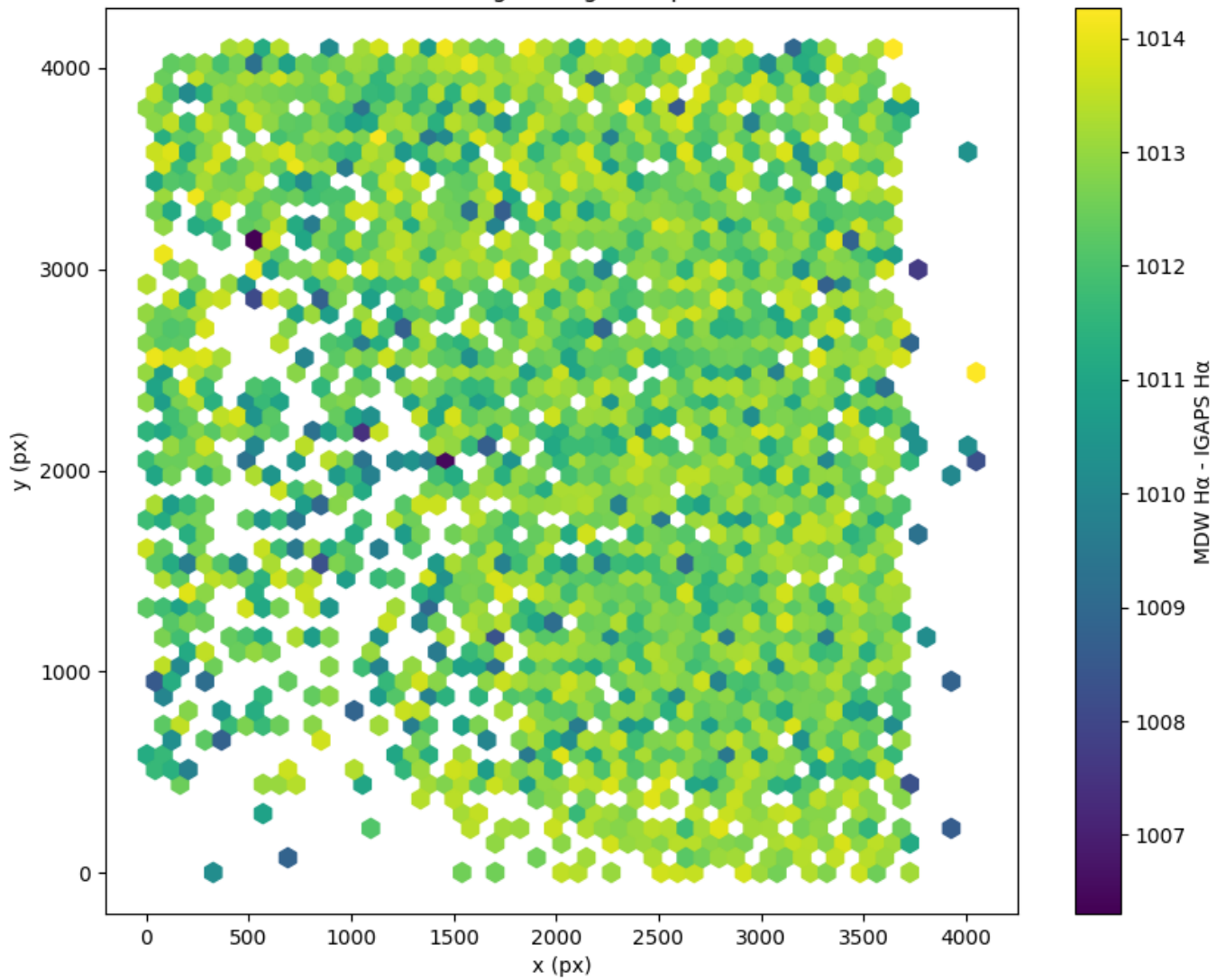
Field 2365 2D field distribution of (MDW H \alpha - Pan-STARRS r) Hexagon length: 81px
