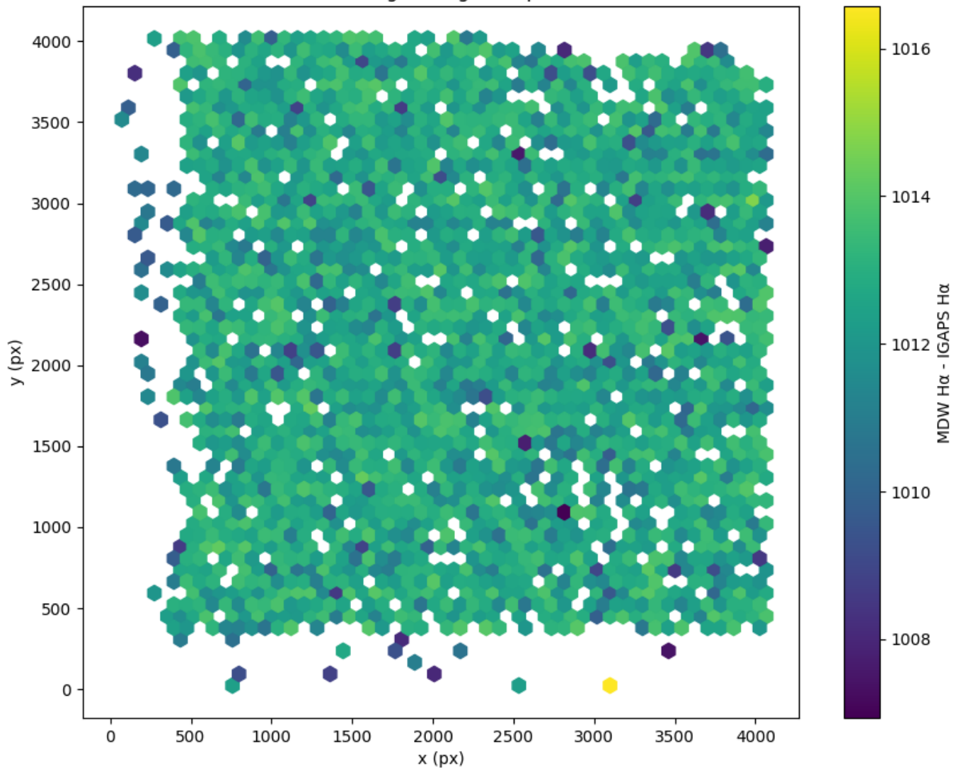
Field 0913 2D field distribution of (MDW H \alpha - Pan-STARRS r) Hexagon length: 81px
