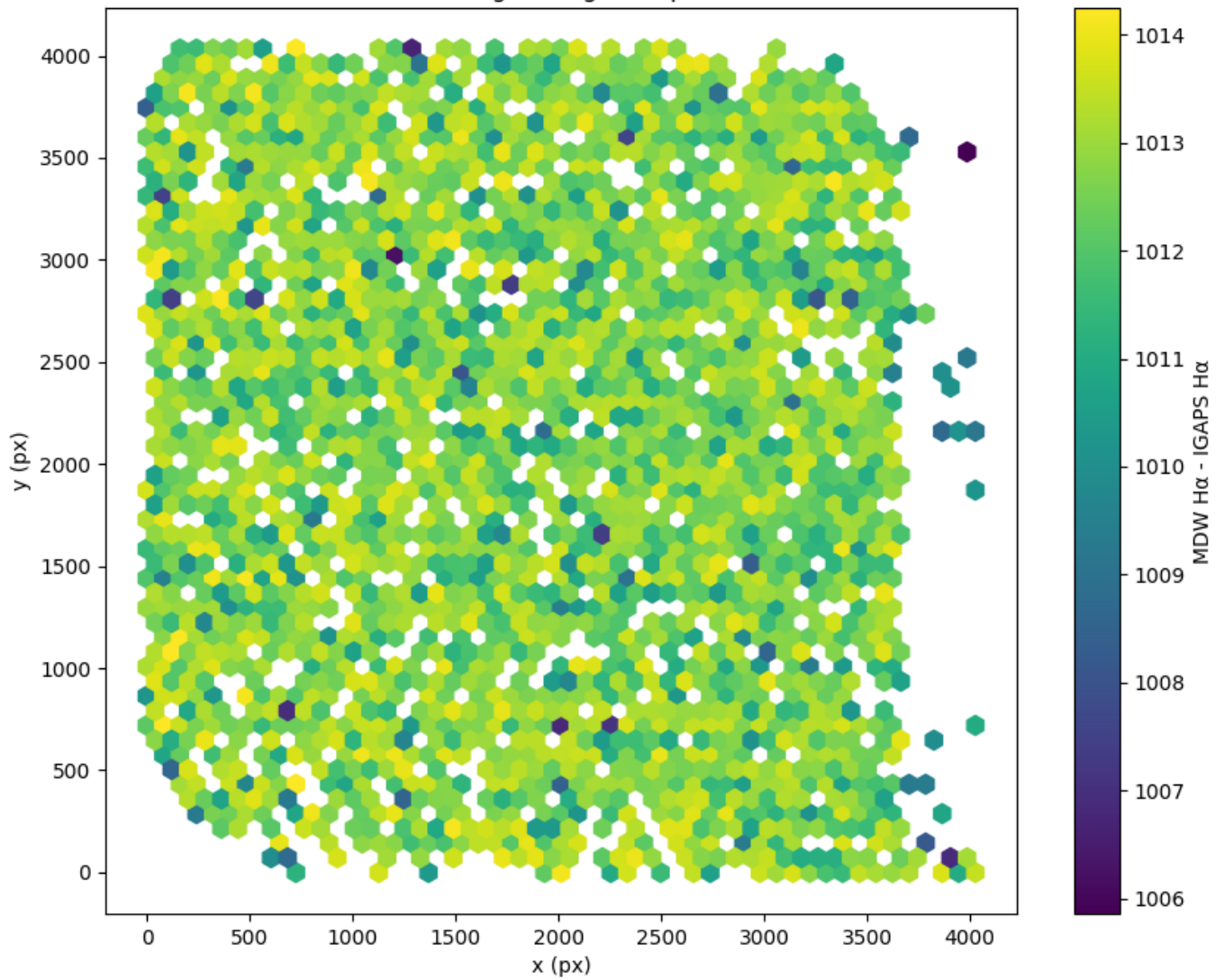
Field 0154 2D field distribution of (MDW H \alpha - Pan-STARRS r) Hexagon length: 81px
