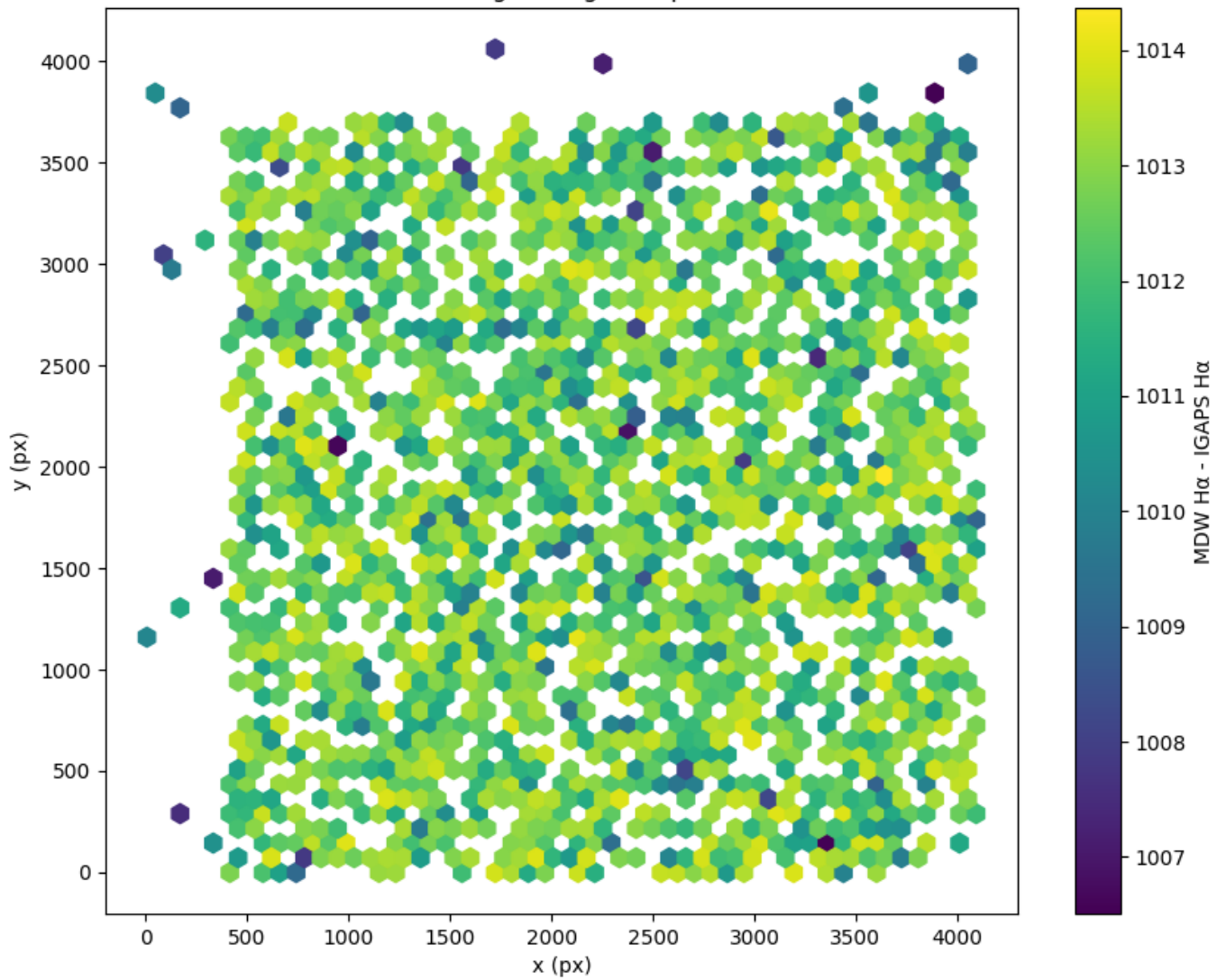
Field 2246 2D field distribution of (MDW H \alpha - Pan-STARRS r) Hexagon length: 82px
