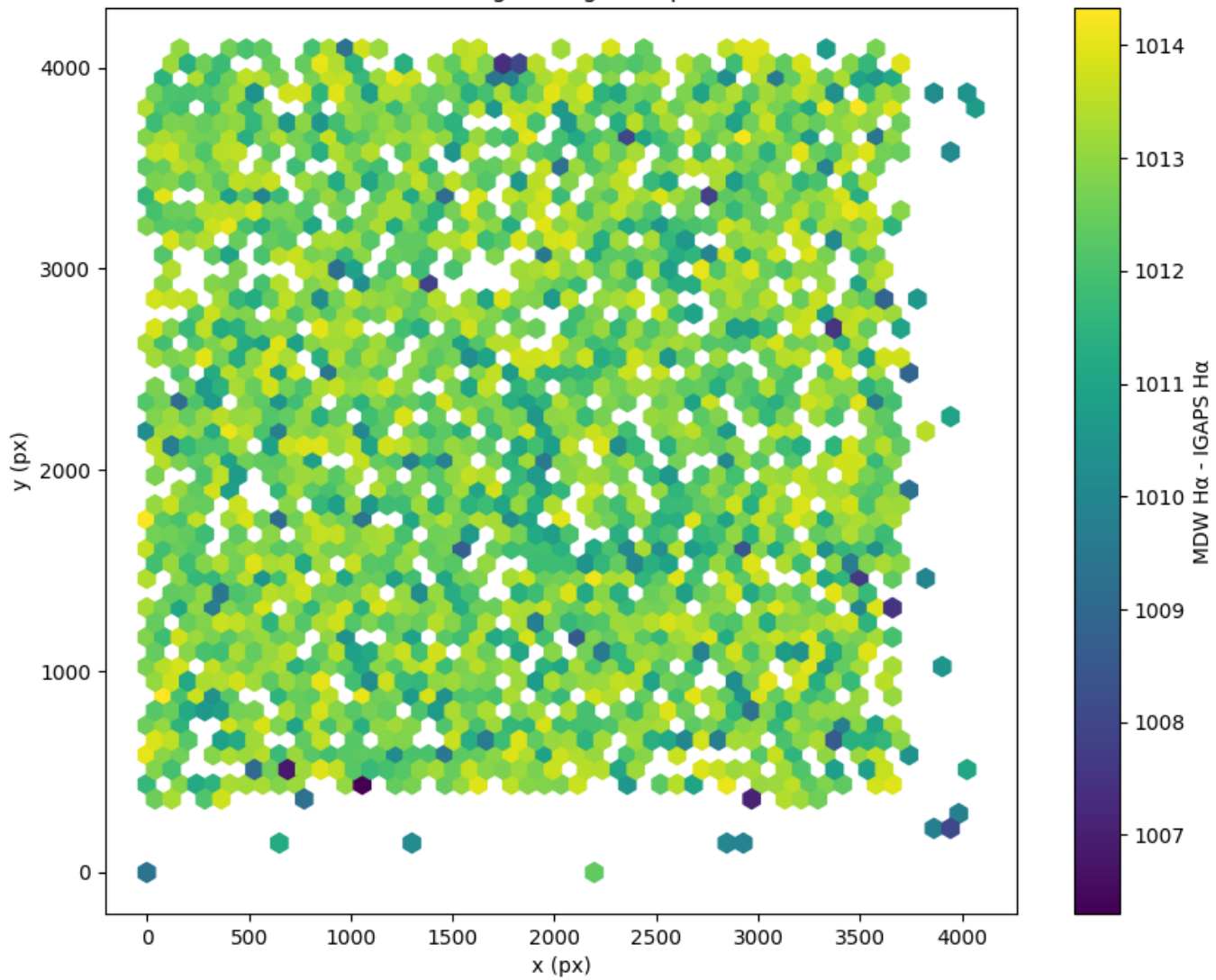
Field 2136 2D field distribution of (MDW H \alpha - Pan-STARRS r) Hexagon length: 81px
