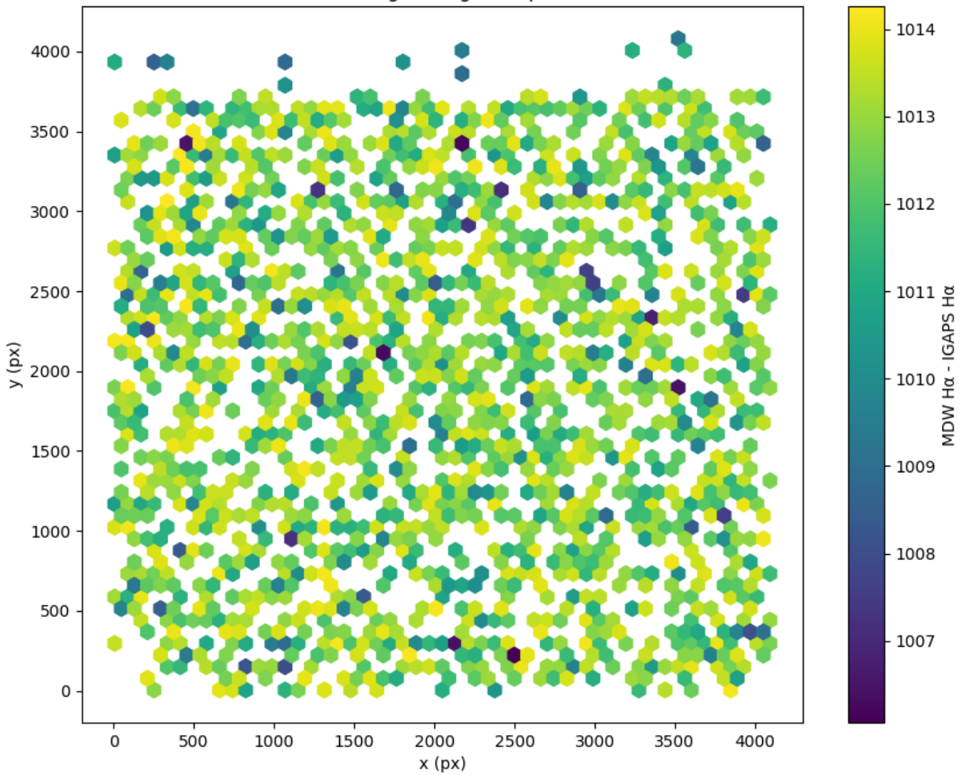
Field 2994 2D field distribution of (MDW H \alpha - Pan-STARRS r) Hexagon length: 82px
