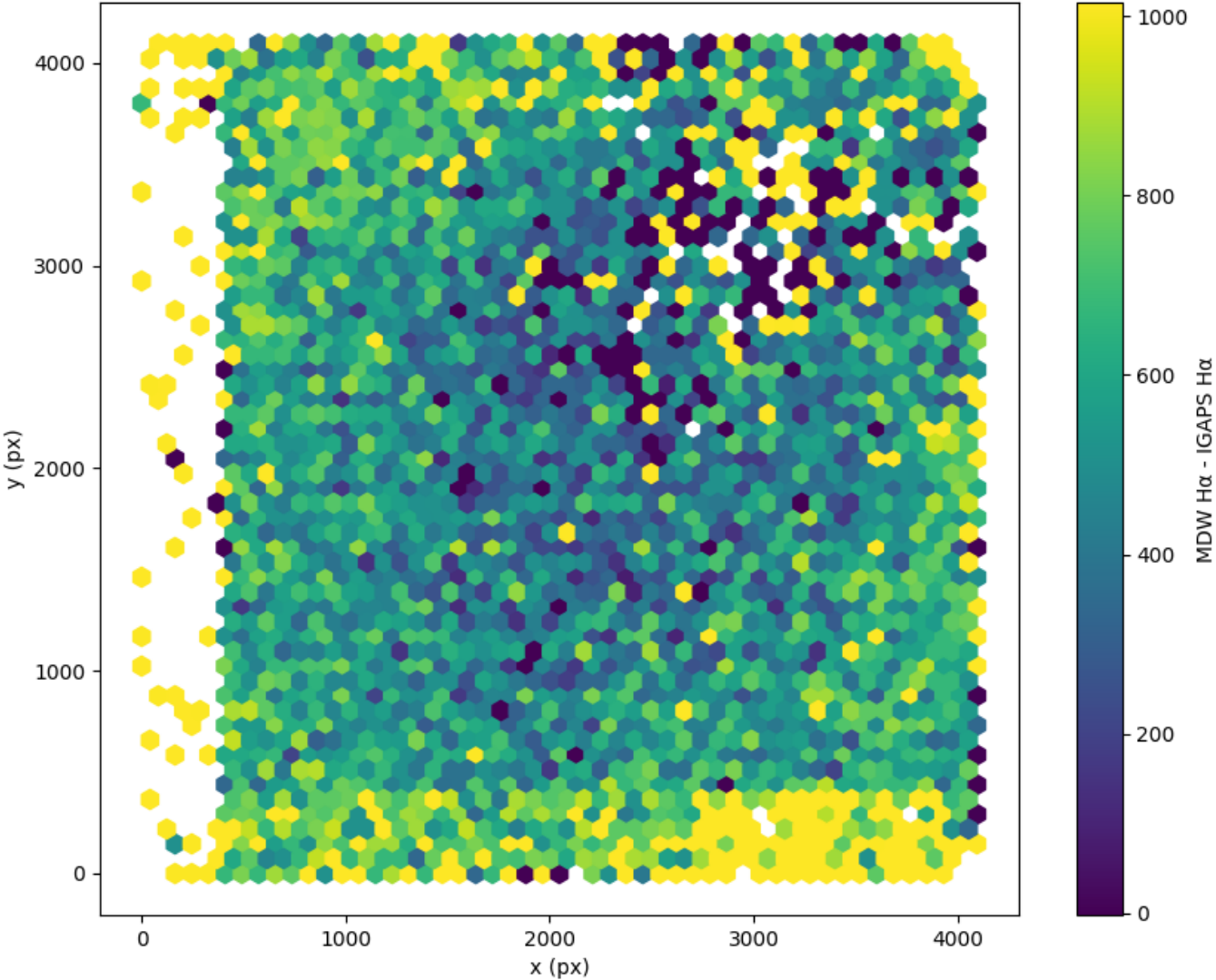
Field 0367 2D field distribution of (MDW H \alpha - Pan-STARRS r) Hexagon length: 82px
