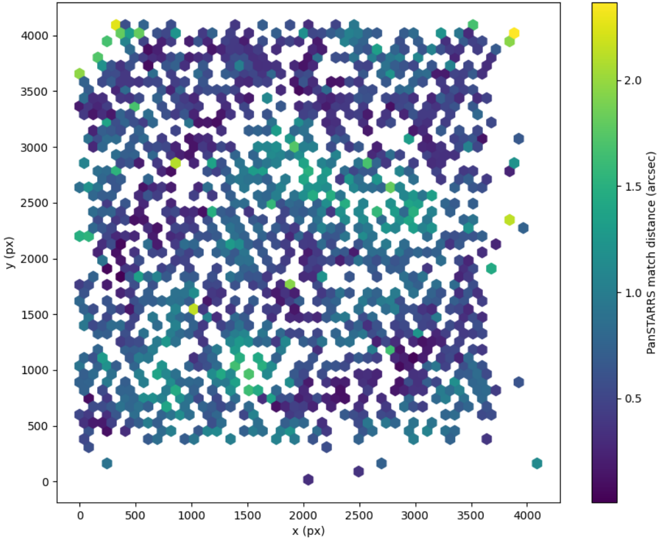
Field 2682 2D field distribution of catalog-matching distance (arcsec) to Pan-STARRS Hexagon length: 82px
