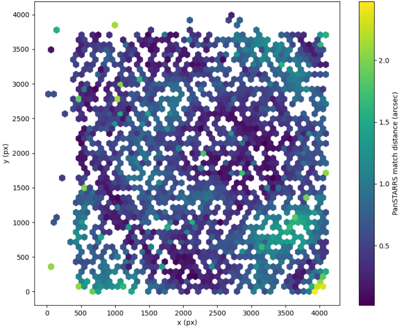
Field 2357 2D field distribution of catalog-matching distance (arcsec) to Pan-STARRS Hexagon length: 81px
