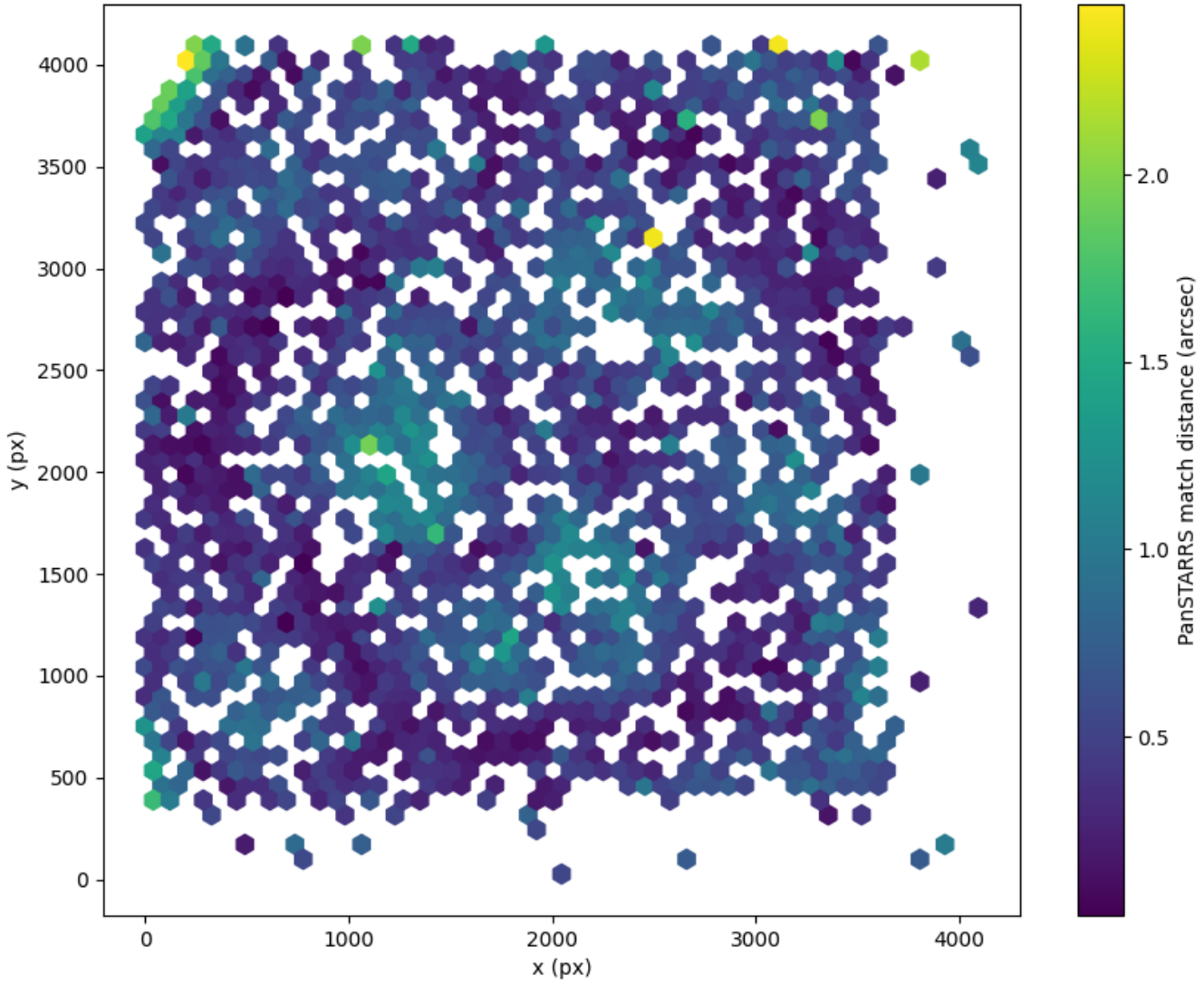
Field 2795 2D field distribution of catalog-matching distance (arcsec) to Pan-STARRS Hexagon length: 82px
