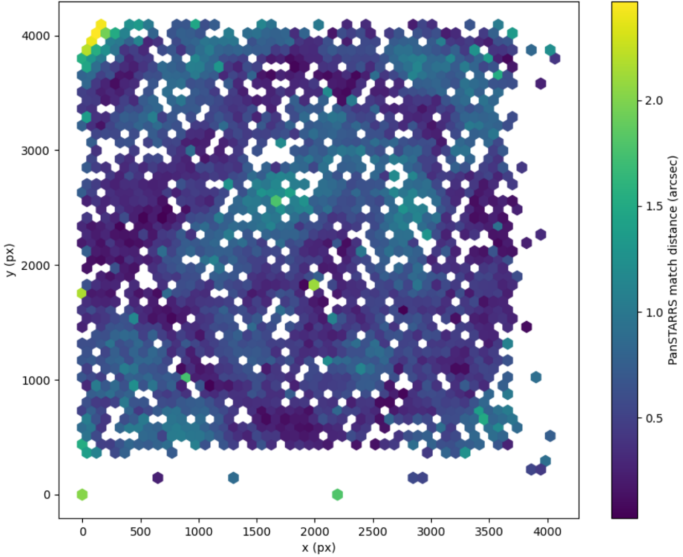
Field 2136 2D field distribution of catalog-matching distance (arcsec) to Pan-STARRS Hexagon length: 81px
