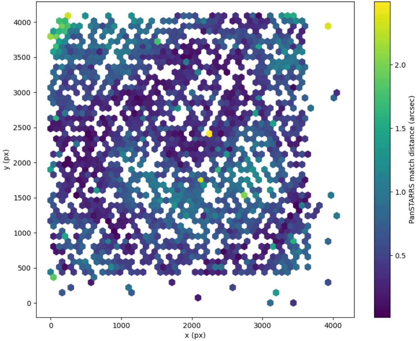
Field 2793 2D field distribution of catalog-matching distance (arcsec) to Pan-STARRS Hexagon length: 82px
