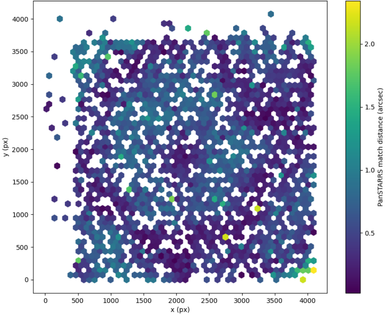
Field 2688 2D field distribution of catalog-matching distance (arcsec) to Pan-STARRS Hexagon length: 81px
