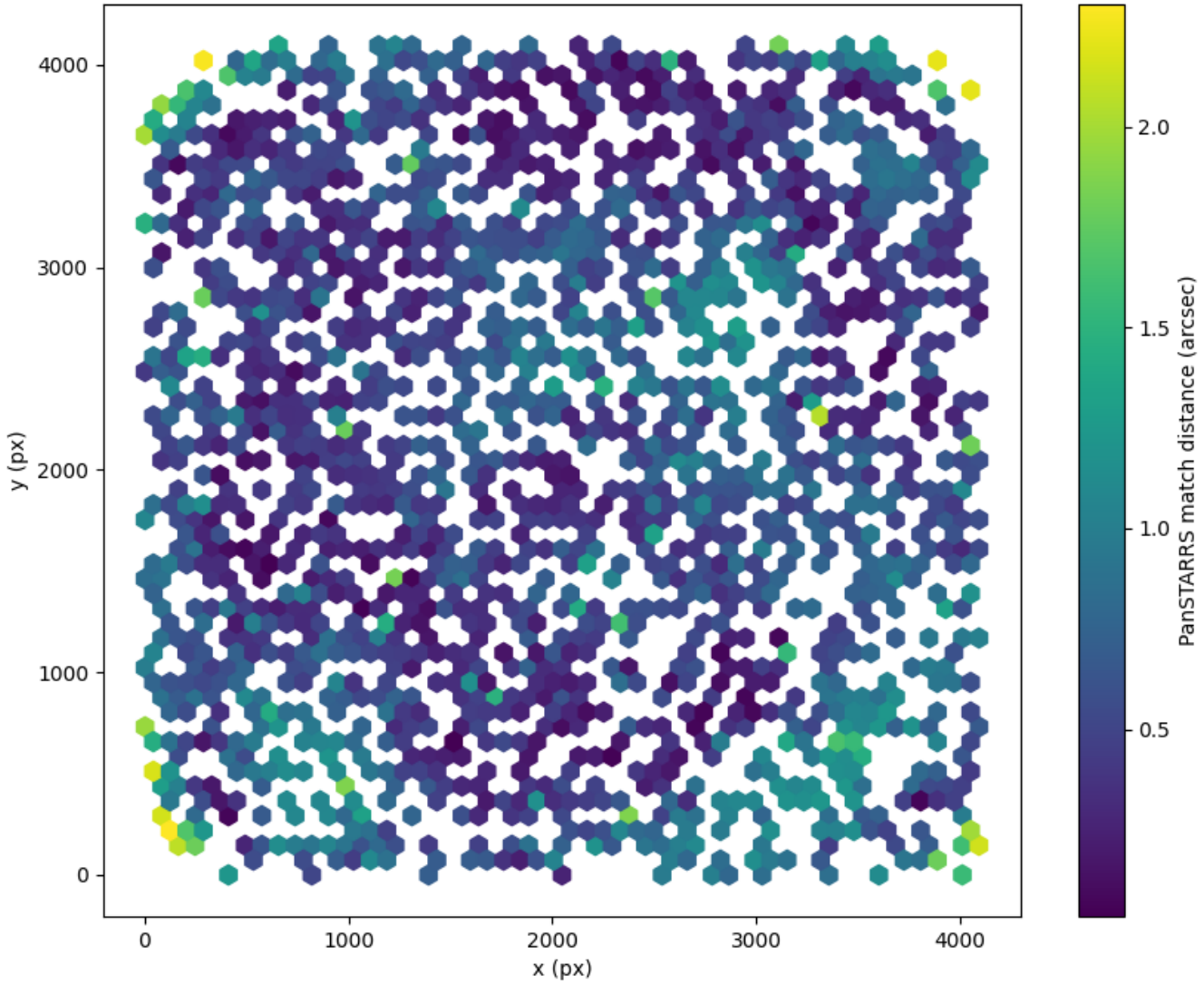
Field 2464 2D field distribution of catalog-matching distance (arcsec) to Pan-STARRS Hexagon length: 82px
