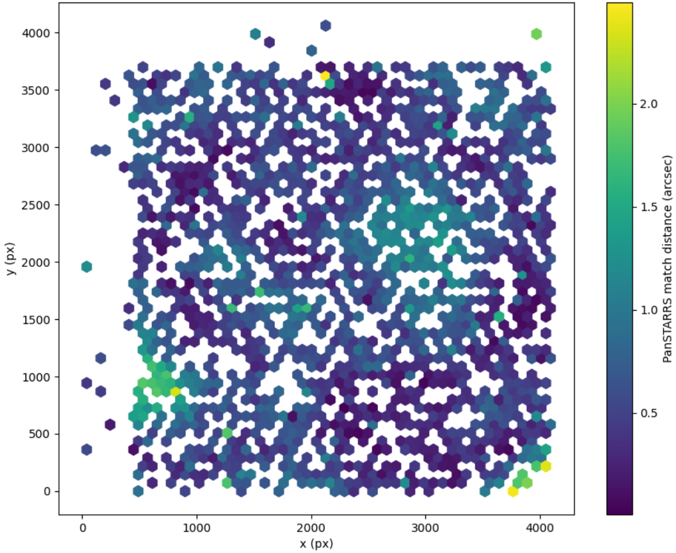
Field 2686 2D field distribution of catalog-matching distance (arcsec) to Pan-STARRS Hexagon length: 82px
