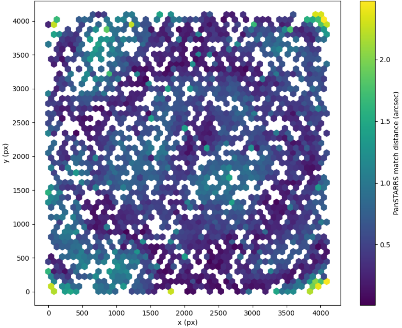
Field 2134 2D field distribution of catalog-matching distance (arcsec) to Pan-STARRS Hexagon length: 82px
