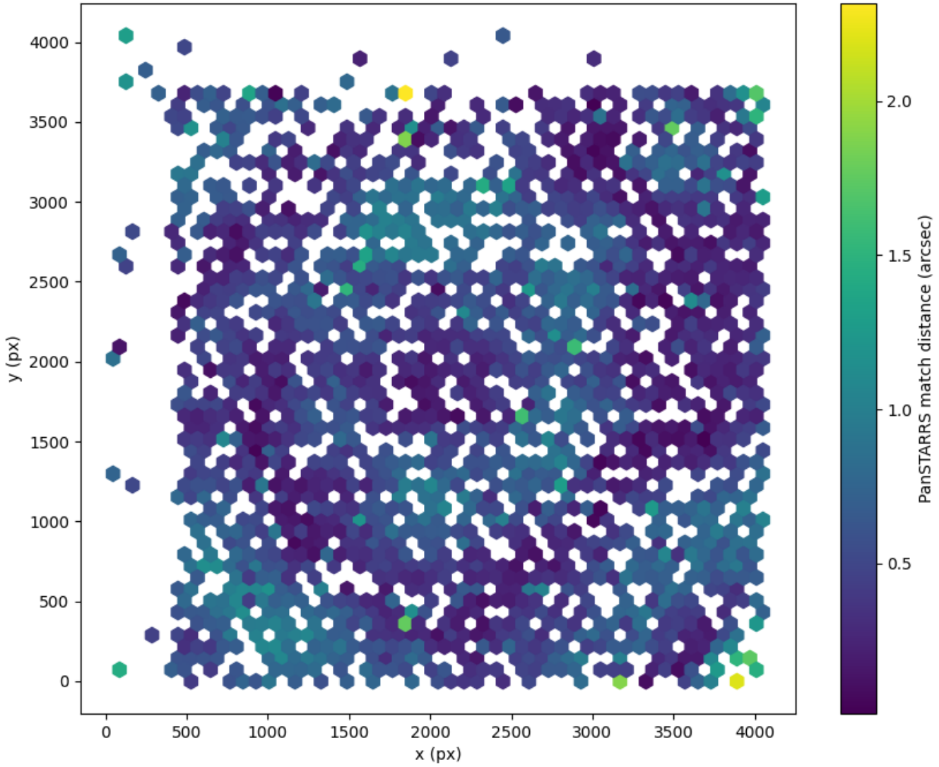
Field 2581 2D field distribution of catalog-matching distance (arcsec) to Pan-STARRS Hexagon length: 80px
