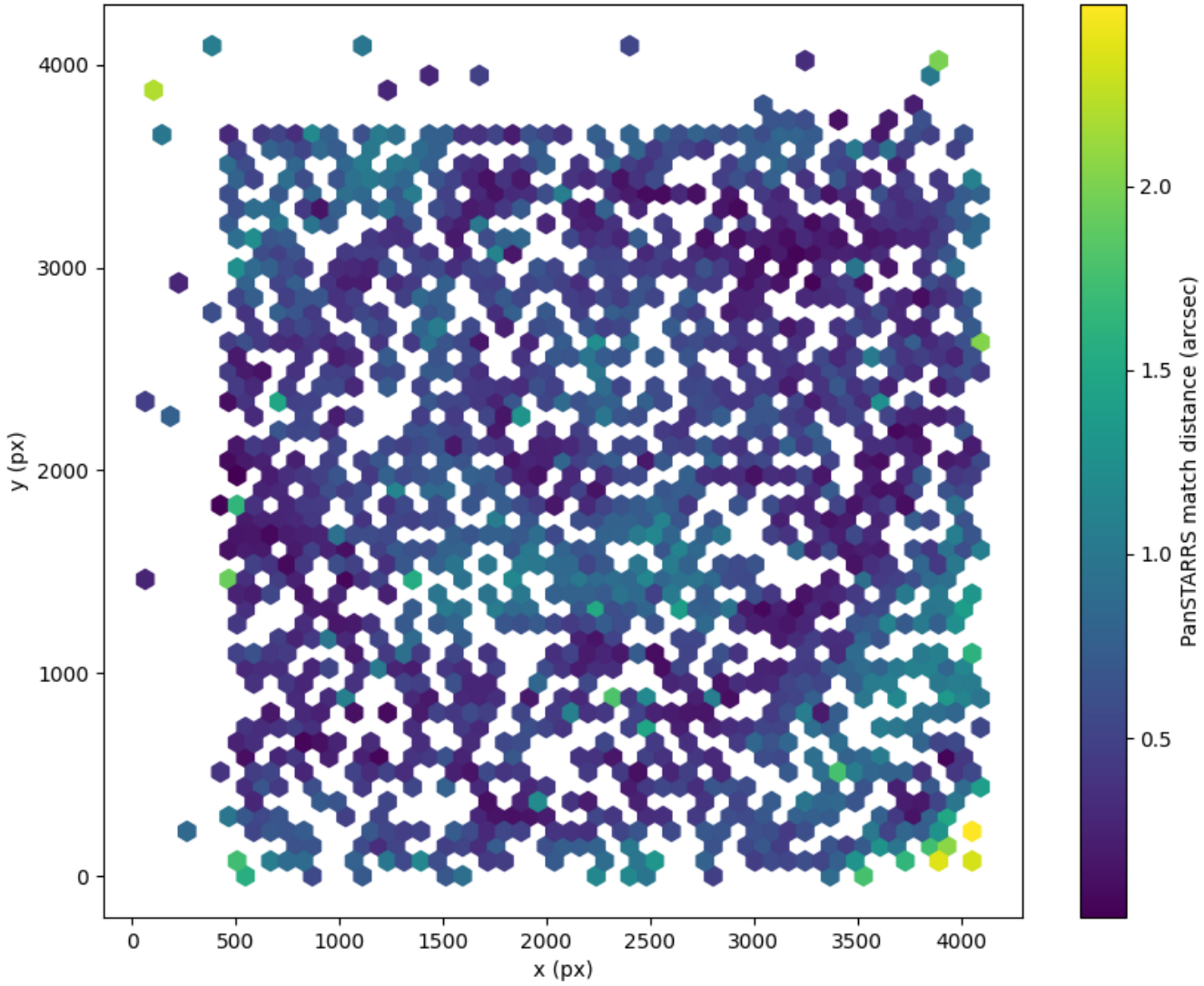
Field 2577 2D field distribution of catalog-matching distance (arcsec) to Pan-STARRS Hexagon length: 81px
