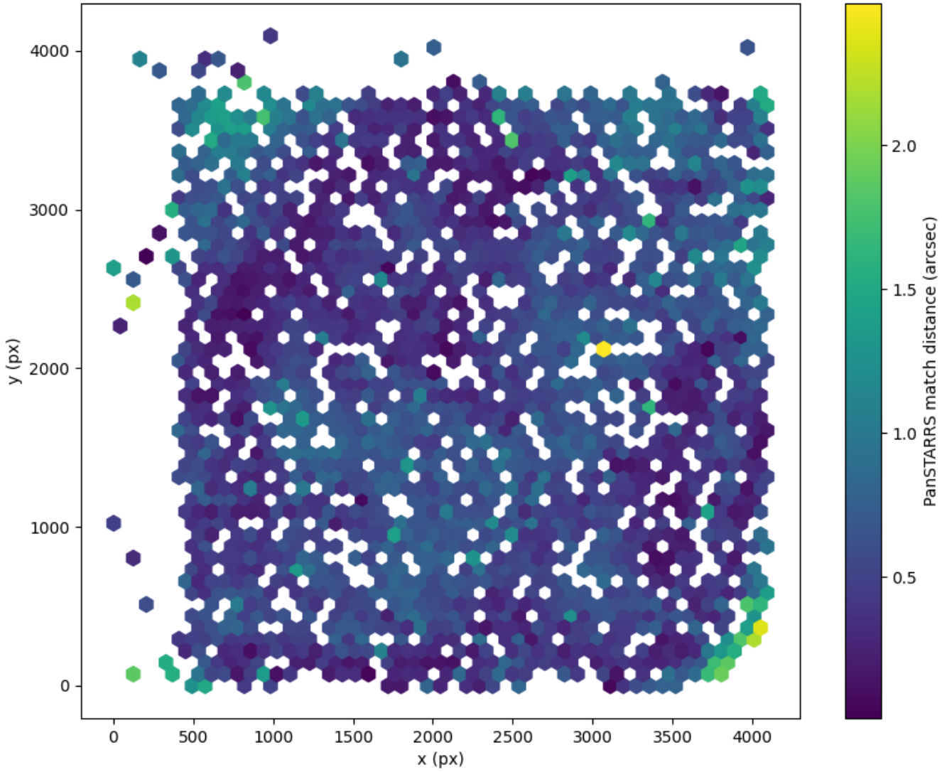
Field 2582 2D field distribution of catalog-matching distance (arcsec) to Pan-STARRS Hexagon length: 82px
