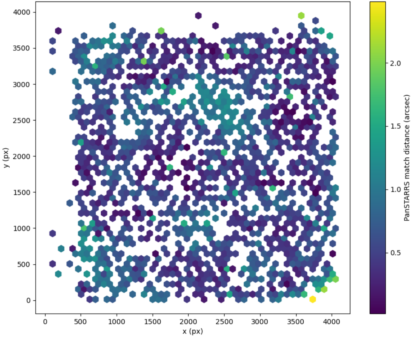
Field 2575 2D field distribution of catalog-matching distance (arcsec) to Pan-STARRS Hexagon length: 80px
