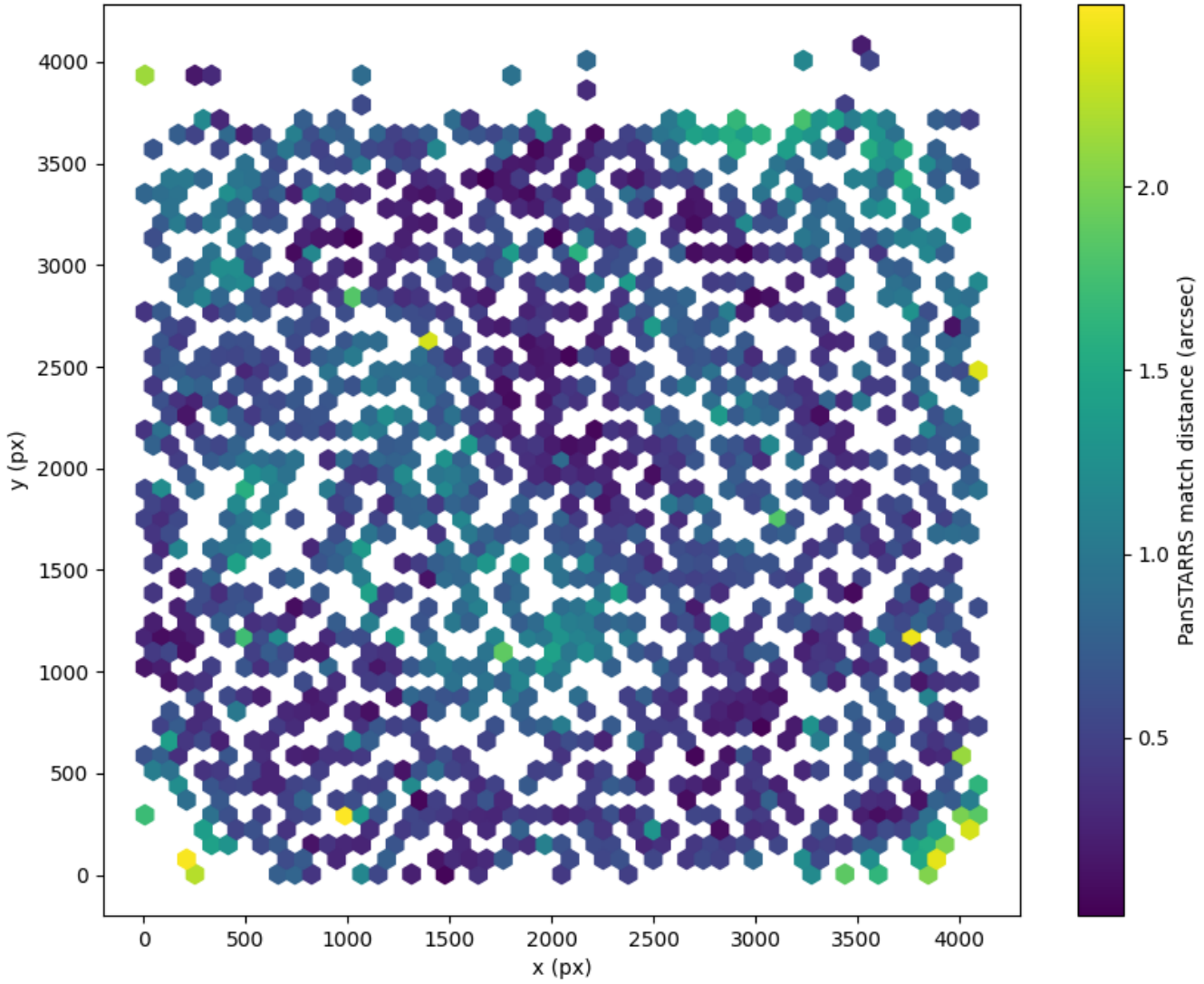
Field 2994 2D field distribution of catalog-matching distance (arcsec) to Pan-STARRS Hexagon length: 82px
