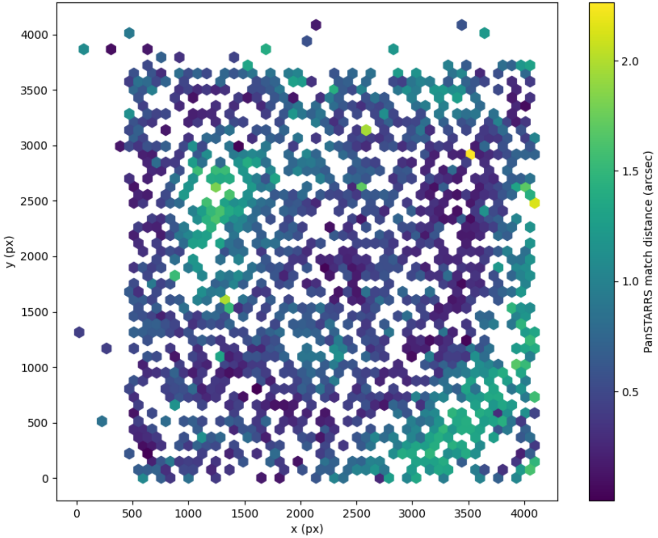
Field 2574 2D field distribution of catalog-matching distance (arcsec) to Pan-STARRS Hexagon length: 81px
