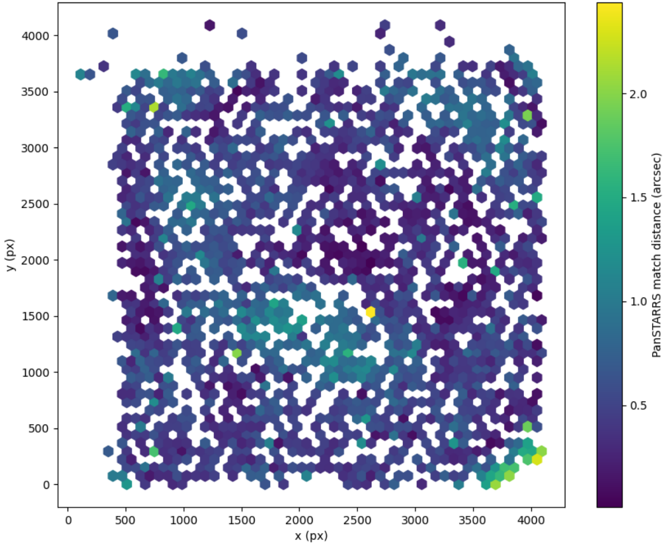
Field 2578 2D field distribution of catalog-matching distance (arcsec) to Pan-STARRS Hexagon length: 80px
