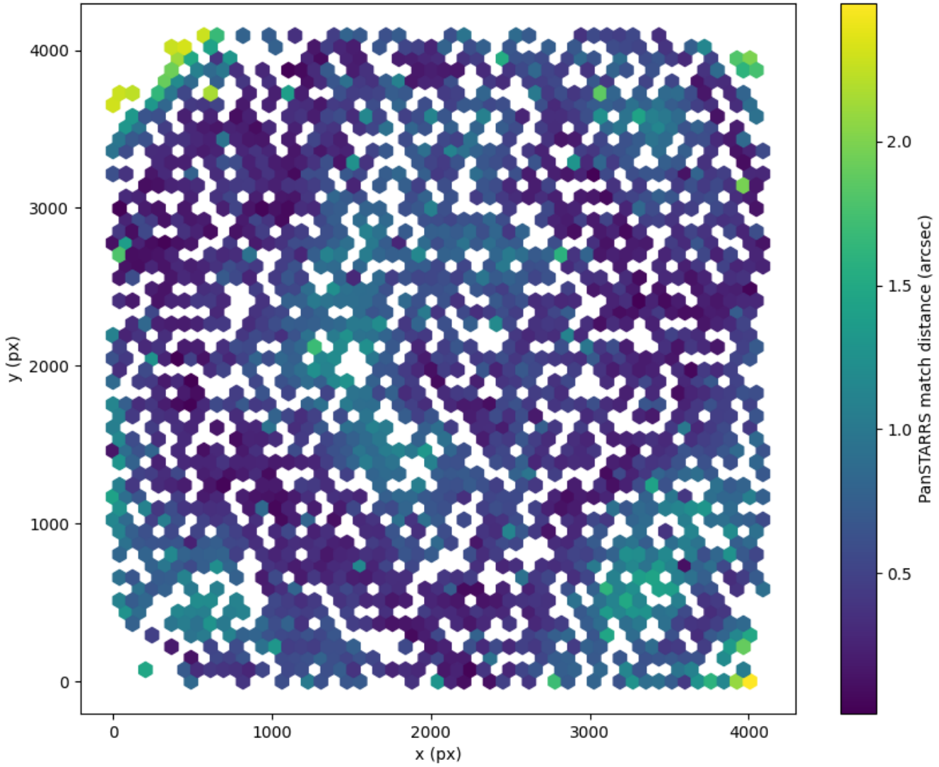
Field 2245 2D field distribution of catalog-matching distance (arcsec) to Pan-STARRS Hexagon length: 82px
