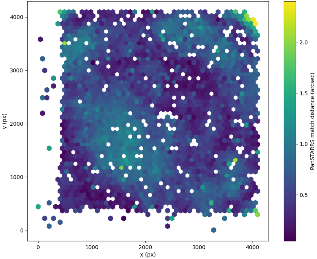
Field 0595 2D field distribution of catalog-matching distance (arcsec) to Pan-STARRS Hexagon length: 82px
