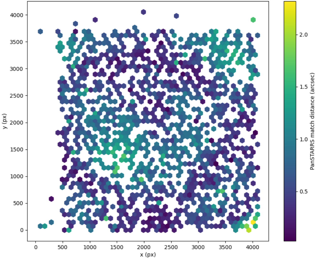
Field 2788 2D field distribution of catalog-matching distance (arcsec) to Pan-STARRS Hexagon length: 81px
