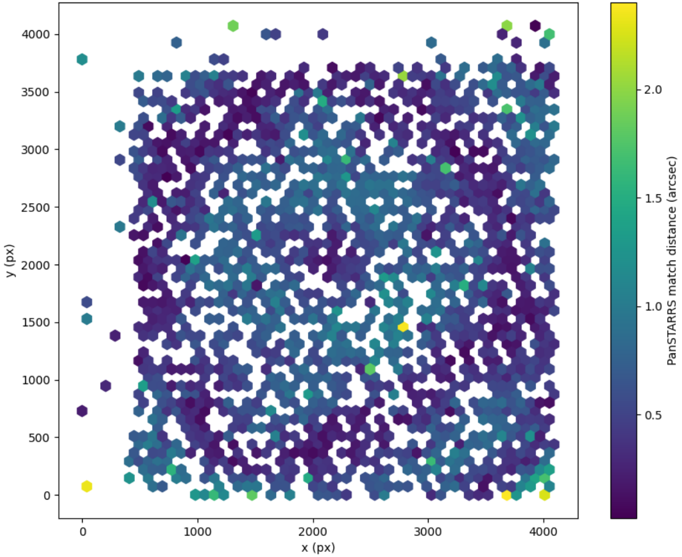
Field 2687 2D field distribution of catalog-matching distance (arcsec) to Pan-STARRS Hexagon length: 82px
