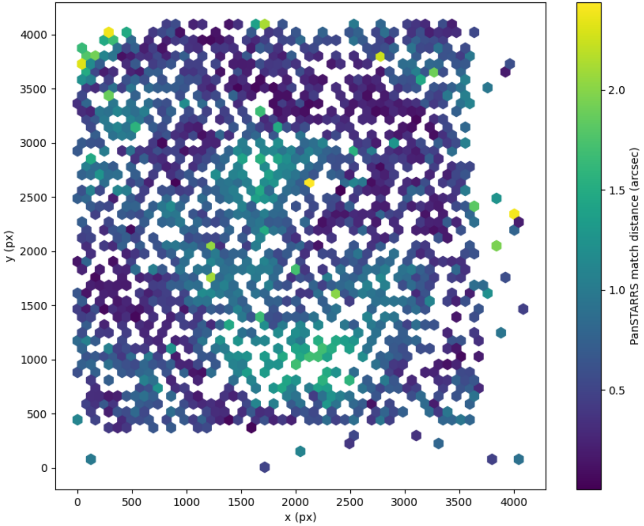
Field 2896 2D field distribution of catalog-matching distance (arcsec) to Pan-STARRS Hexagon length: 82px
