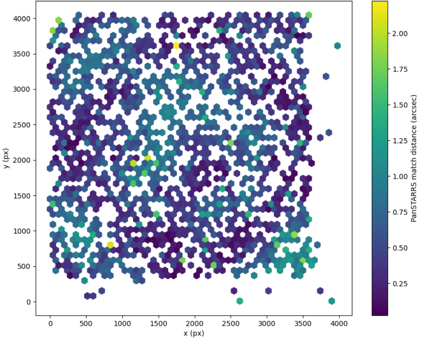
Field 2894 2D field distribution of catalog-matching distance (arcsec) to Pan-STARRS Hexagon length: 80px
