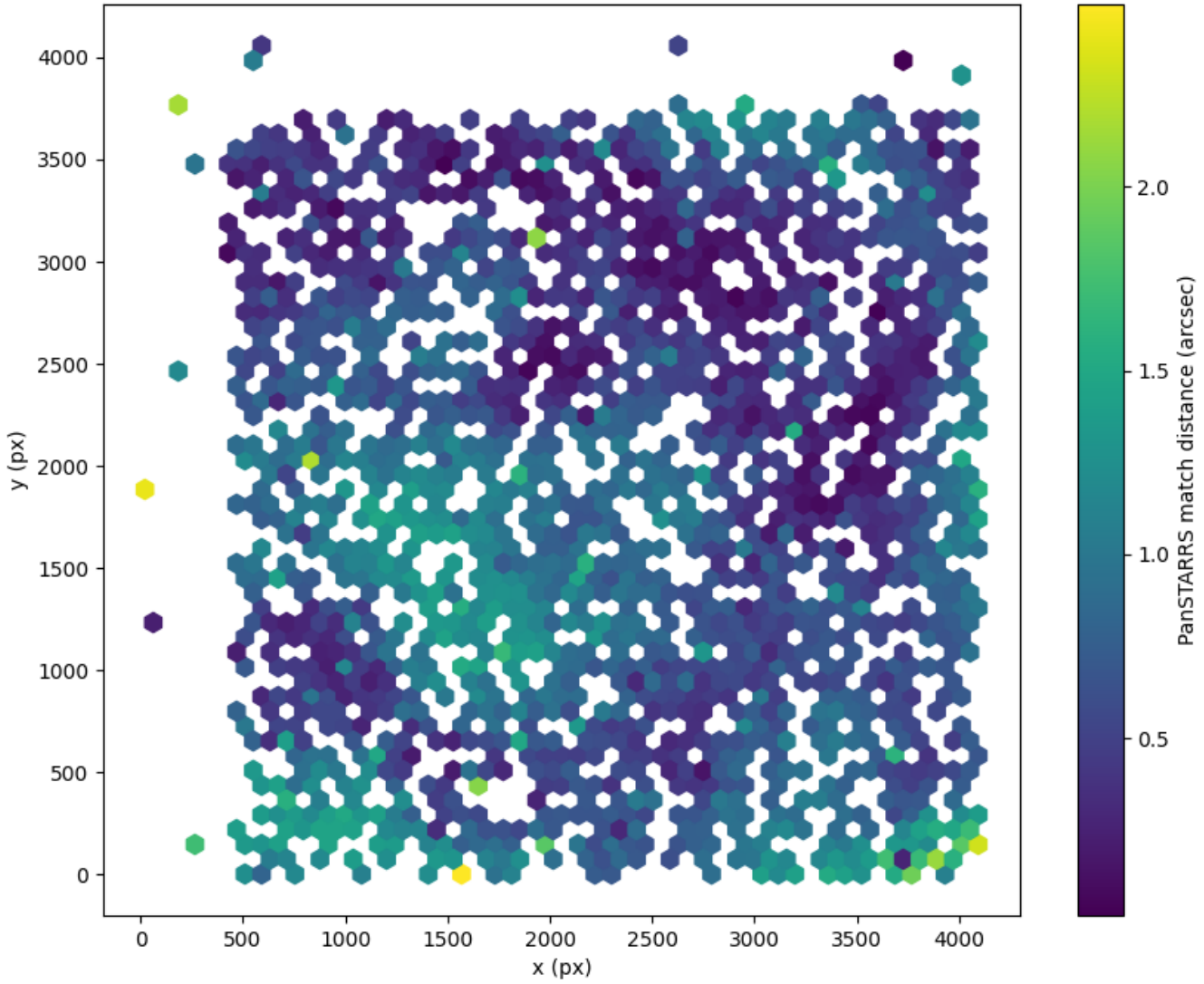
Field 2579 2D field distribution of catalog-matching distance (arcsec) to Pan-STARRS Hexagon length: 81px
