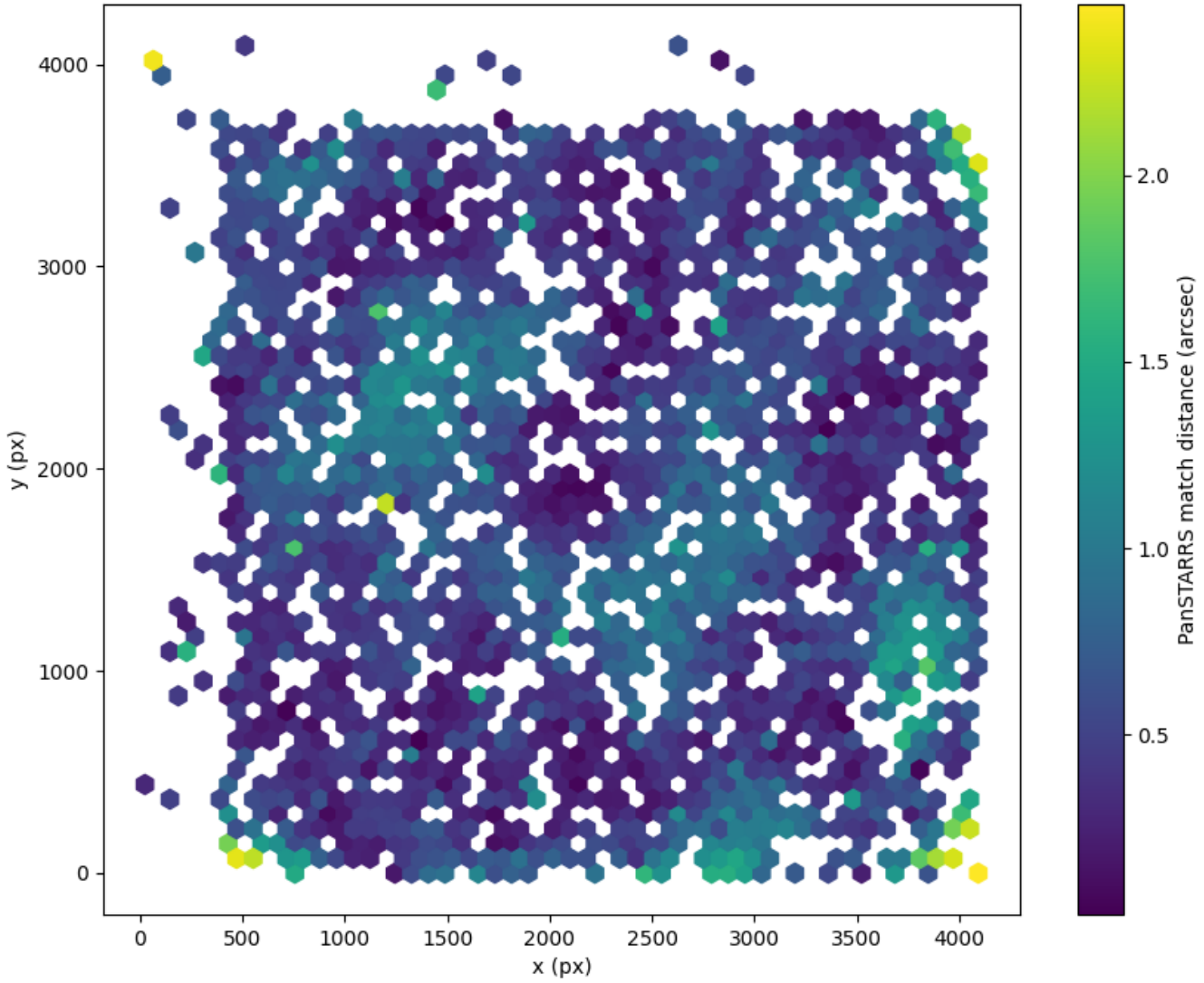
Field 2690 2D field distribution of catalog-matching distance (arcsec) to Pan-STARRS Hexagon length: 81px
