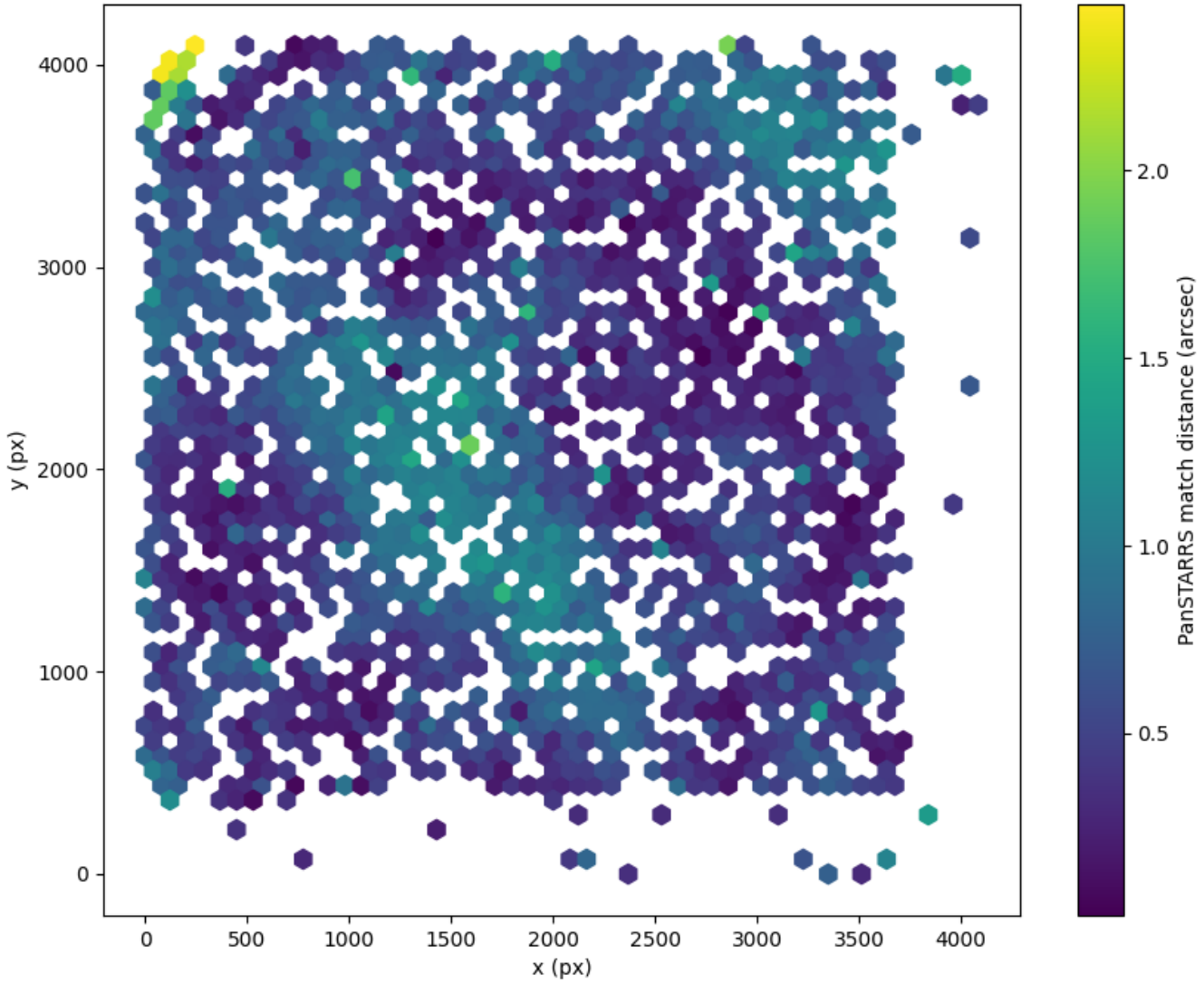
Field 2359 2D field distribution of catalog-matching distance (arcsec) to Pan-STARRS Hexagon length: 82px
