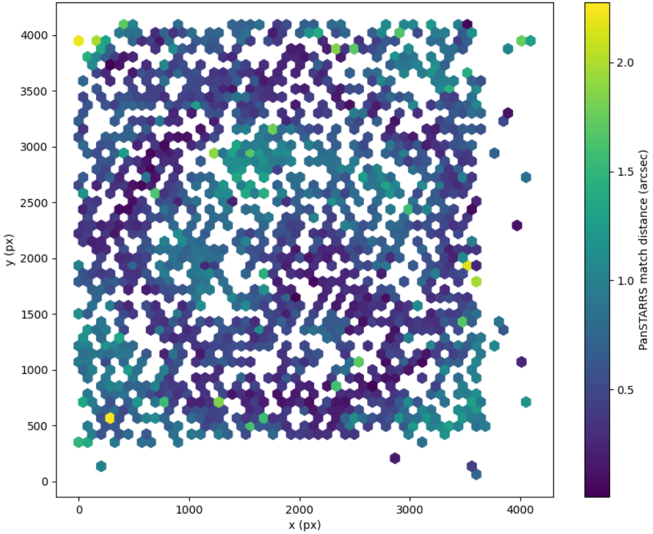
Field 2790 2D field distribution of catalog-matching distance (arcsec) to Pan-STARRS Hexagon length: 82px
