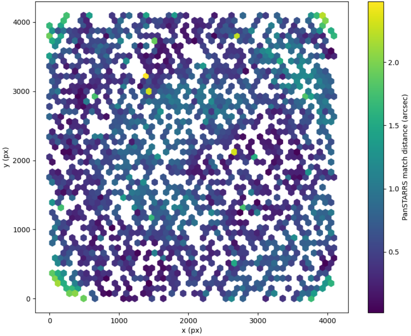
Field 2572 2D field distribution of catalog-matching distance (arcsec) to Pan-STARRS Hexagon length: 82px
