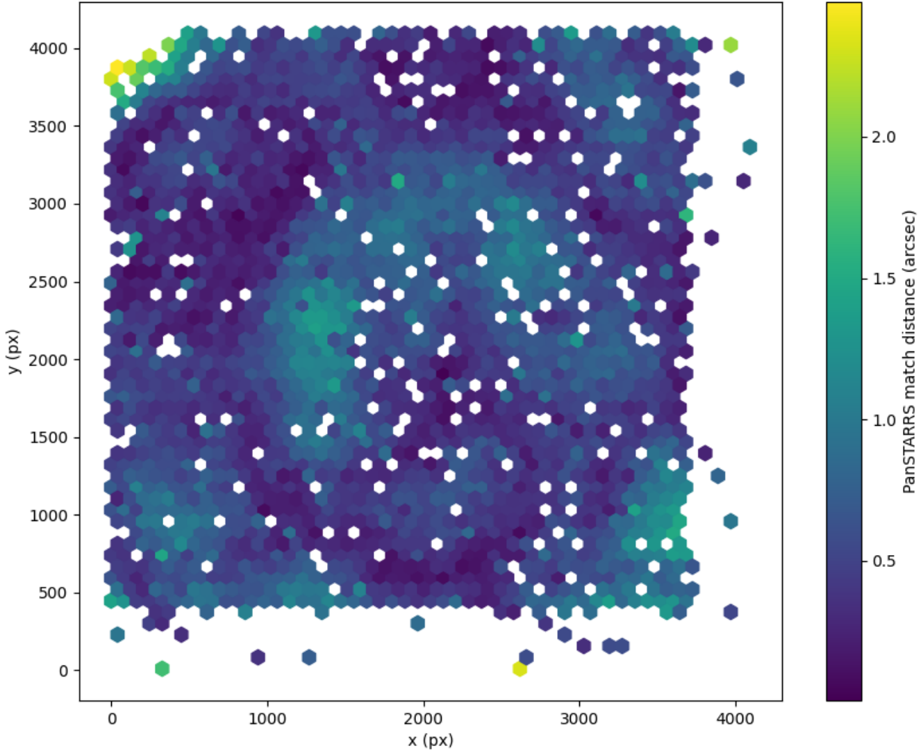
Field 2139 2D field distribution of catalog-matching distance (arcsec) to Pan-STARRS Hexagon length: 82px
