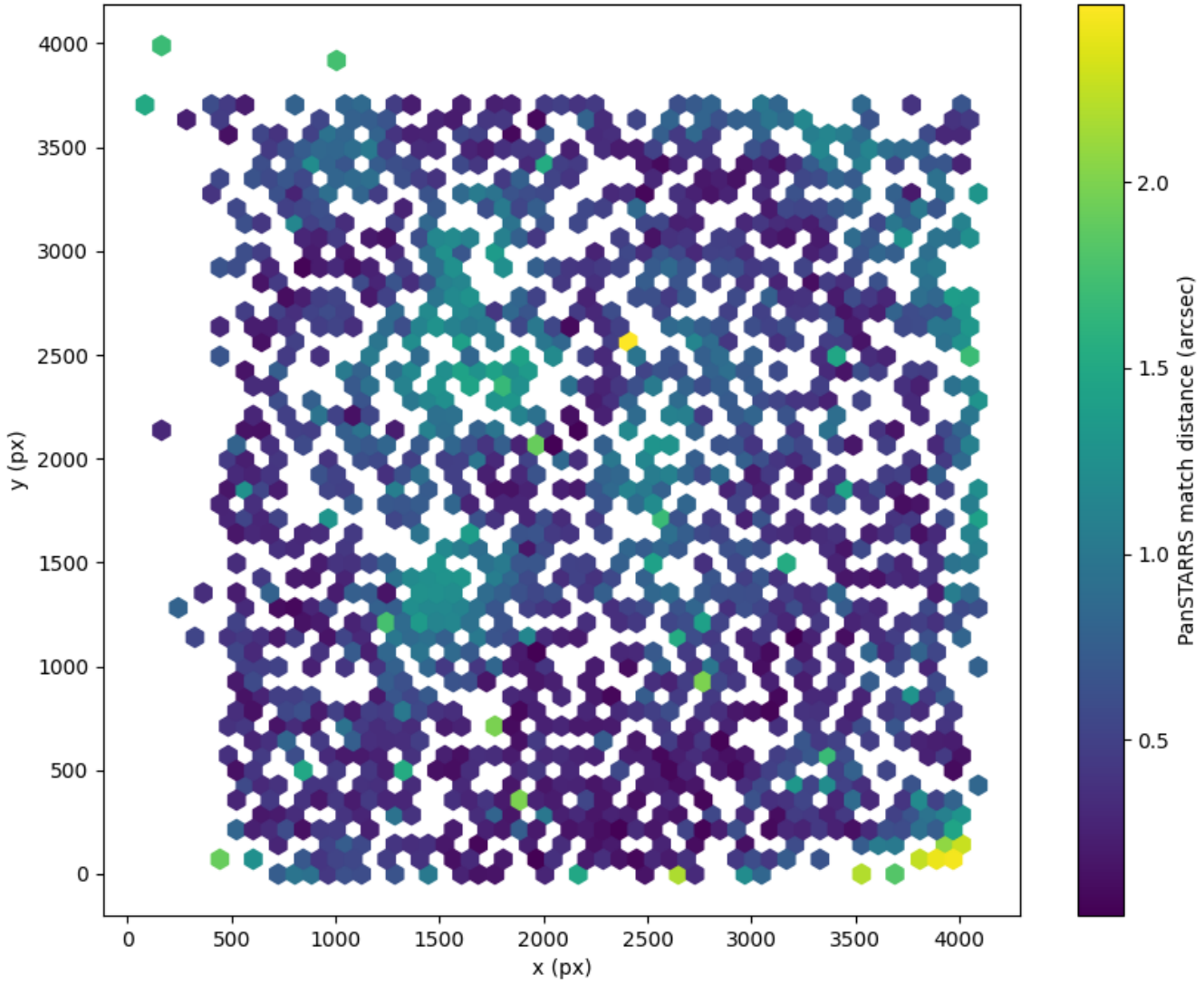
Field 2684 2D field distribution of catalog-matching distance (arcsec) to Pan-STARRS Hexagon length: 80px
