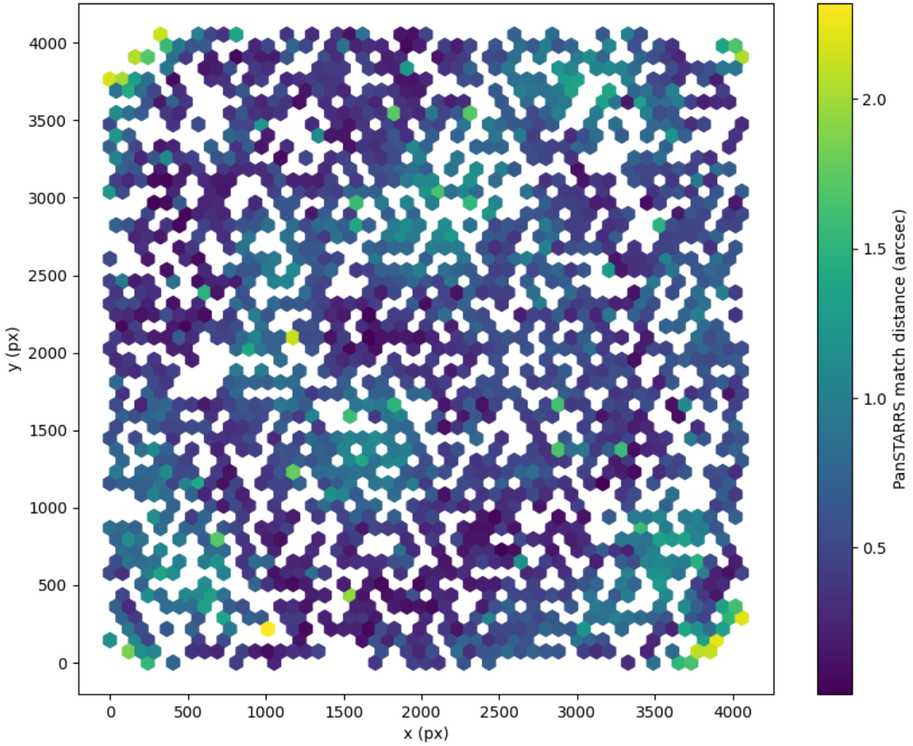
Field 2355 2D field distribution of catalog-matching distance (arcsec) to Pan-STARRS Hexagon length: 81px
