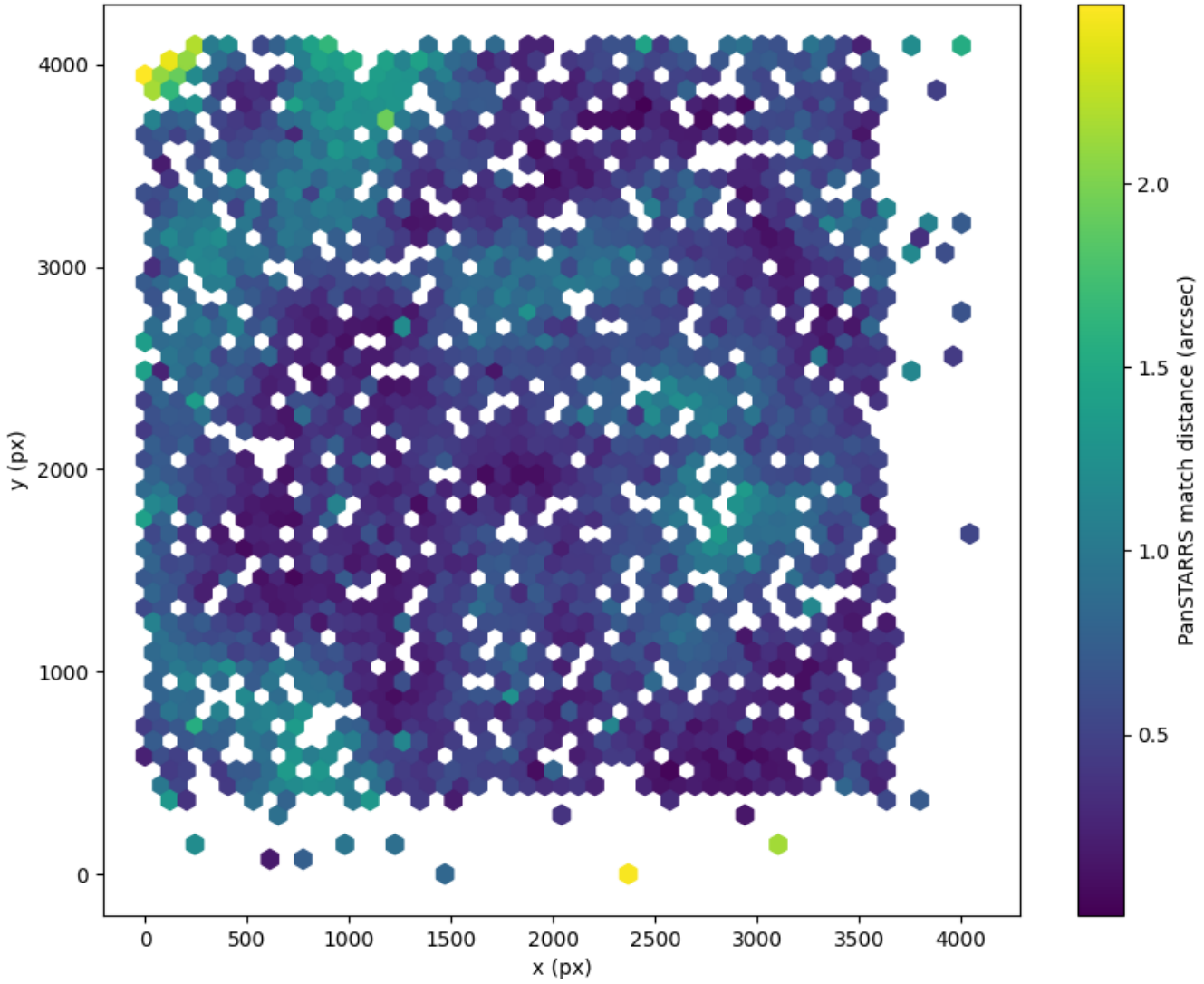
Field 2691 2D field distribution of catalog-matching distance (arcsec) to Pan-STARRS Hexagon length: 82px
