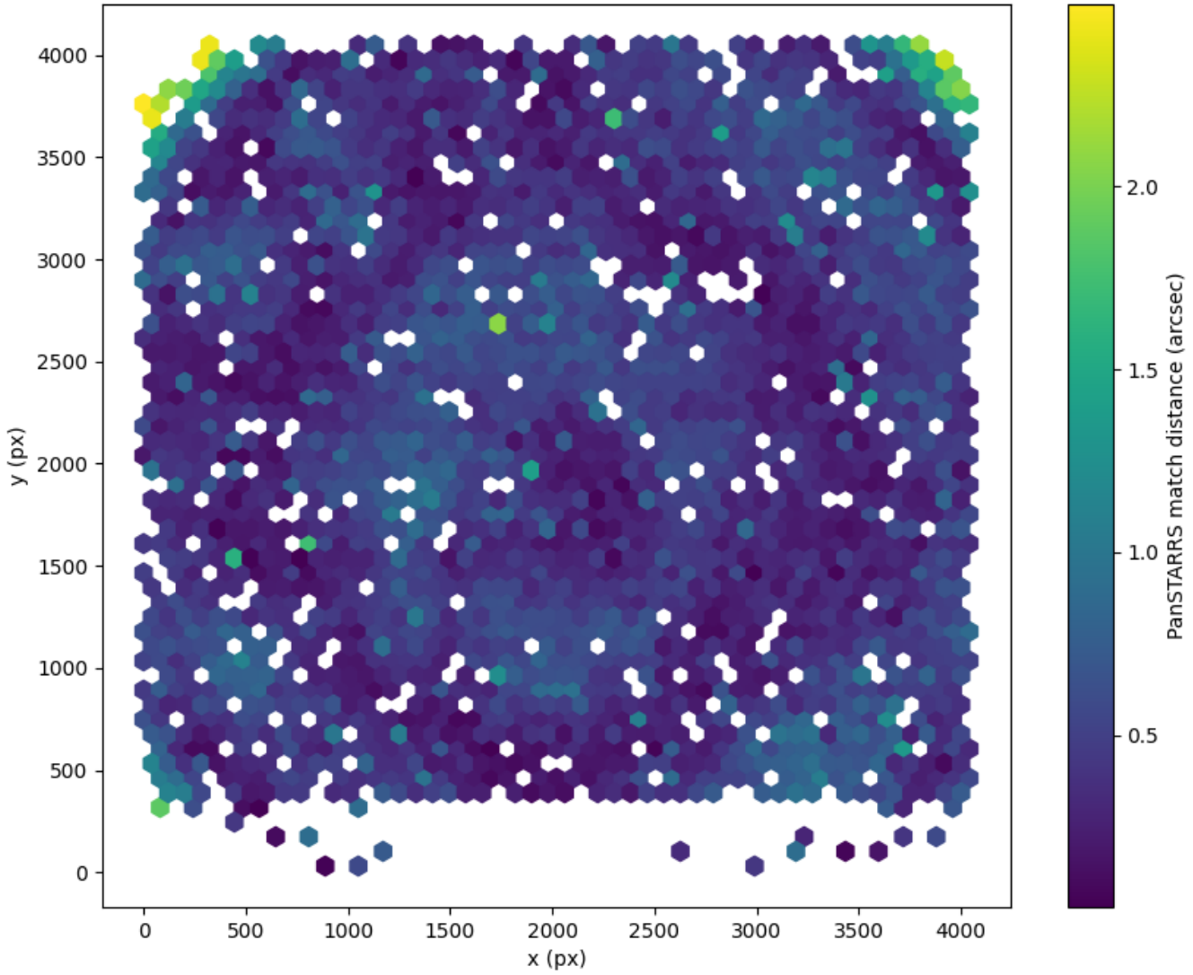
Field 0136 2D field distribution of catalog-matching distance (arcsec) to Pan-STARRS Hexagon length: 81px
