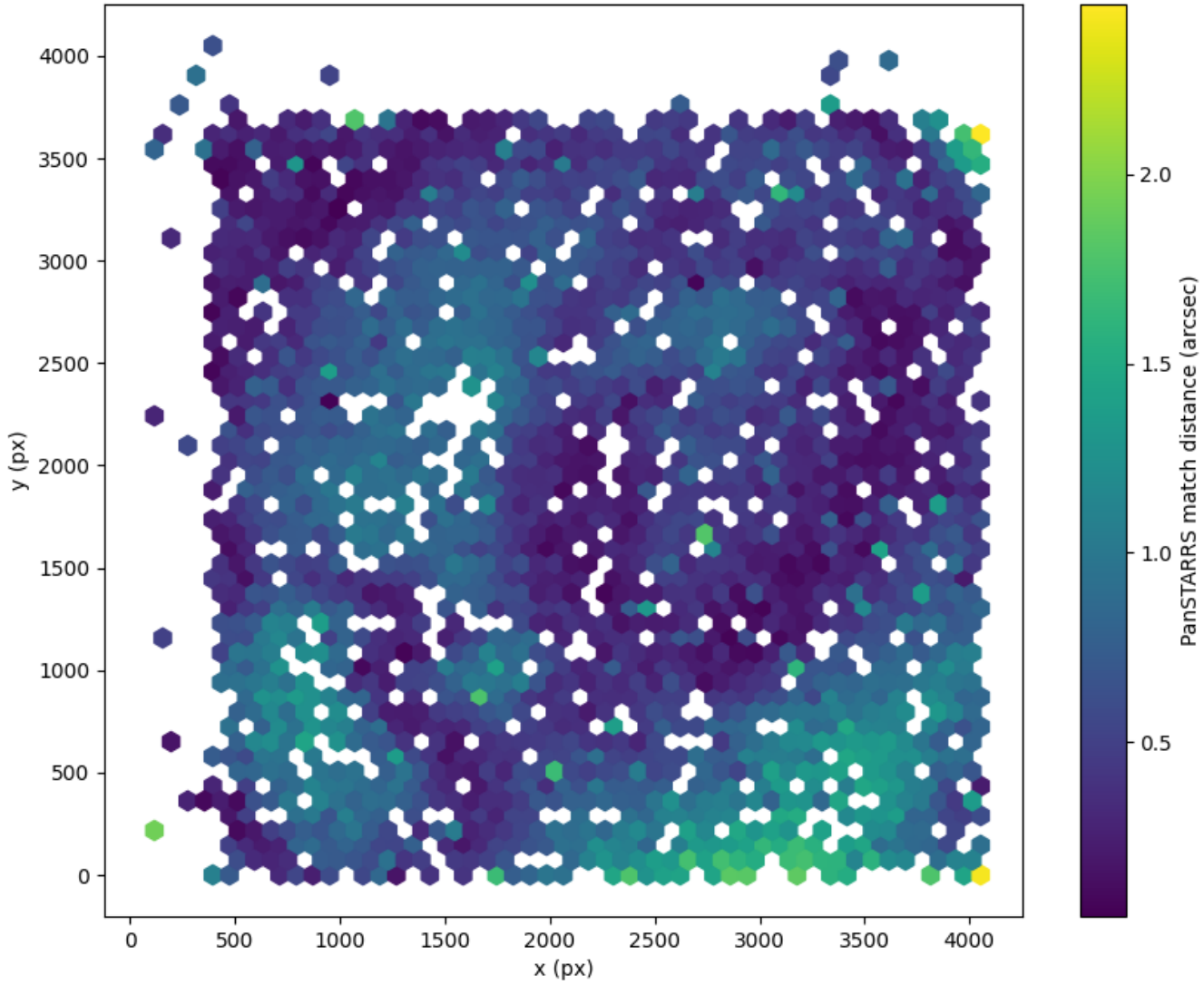
Field 2251 2D field distribution of catalog-matching distance (arcsec) to Pan-STARRS Hexagon length: 80px
