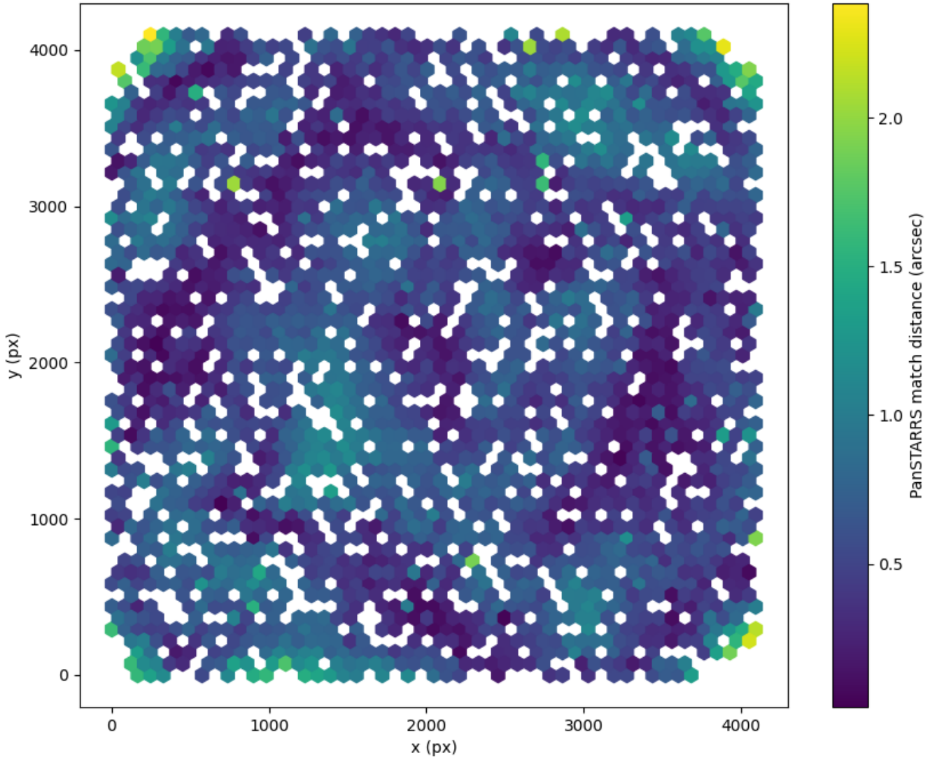
Field 0022 2D field distribution of catalog-matching distance (arcsec) to Pan-STARRS Hexagon length: 82px
