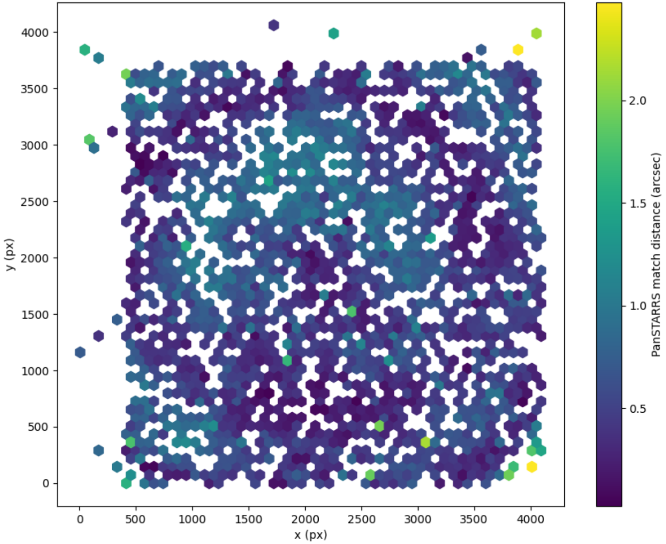
Field 2246 2D field distribution of catalog-matching distance (arcsec) to Pan-STARRS Hexagon length: 82px
