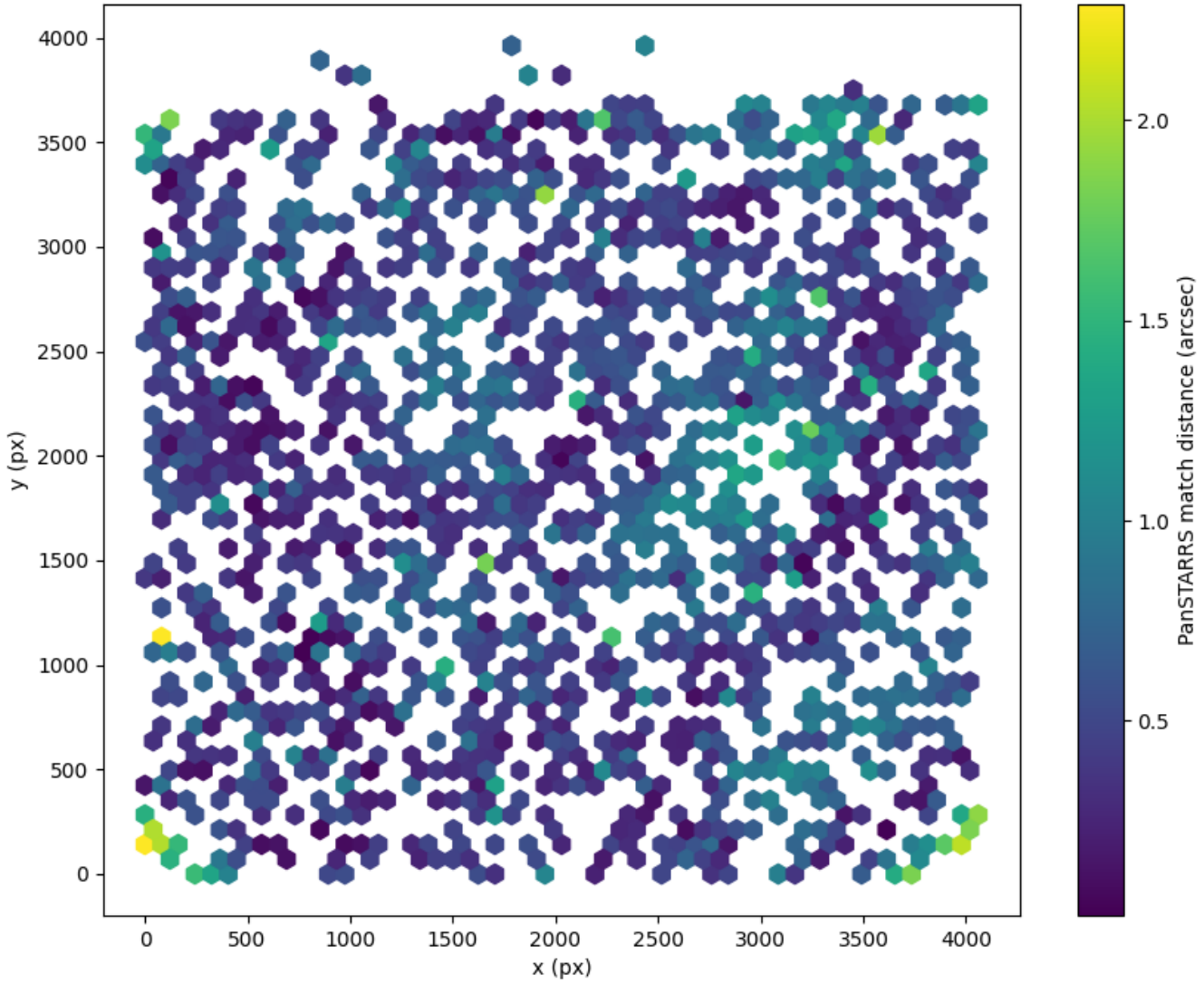
Field 2787 2D field distribution of catalog-matching distance (arcsec) to Pan-STARRS Hexagon length: 81px
