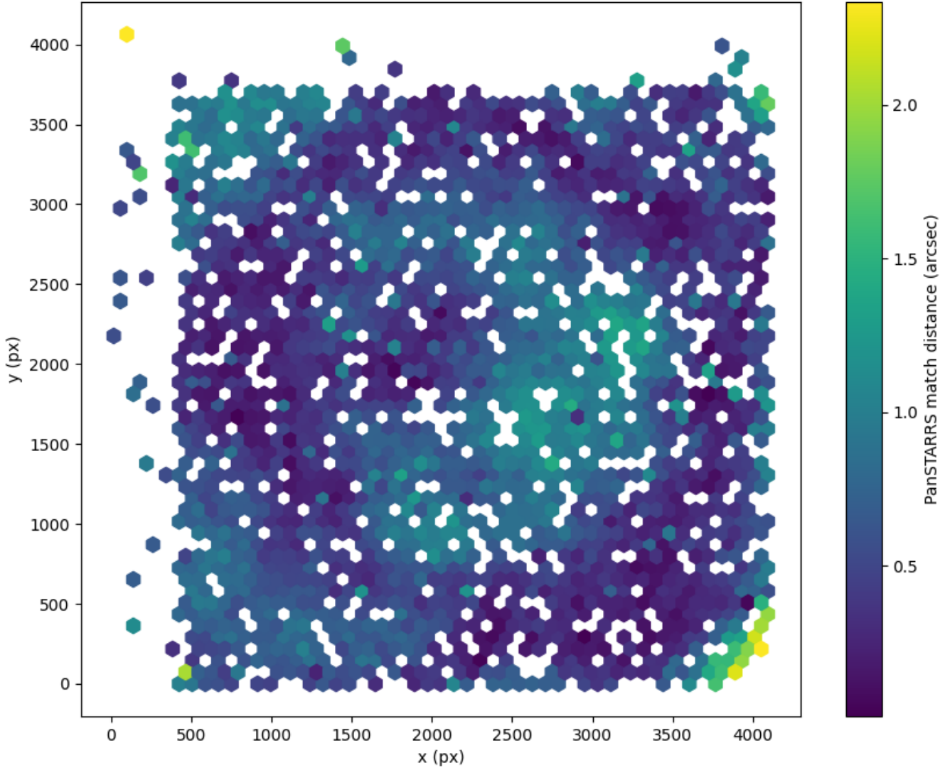
Field 2473 2D field distribution of catalog-matching distance (arcsec) to Pan-STARRS Hexagon length: 81px
