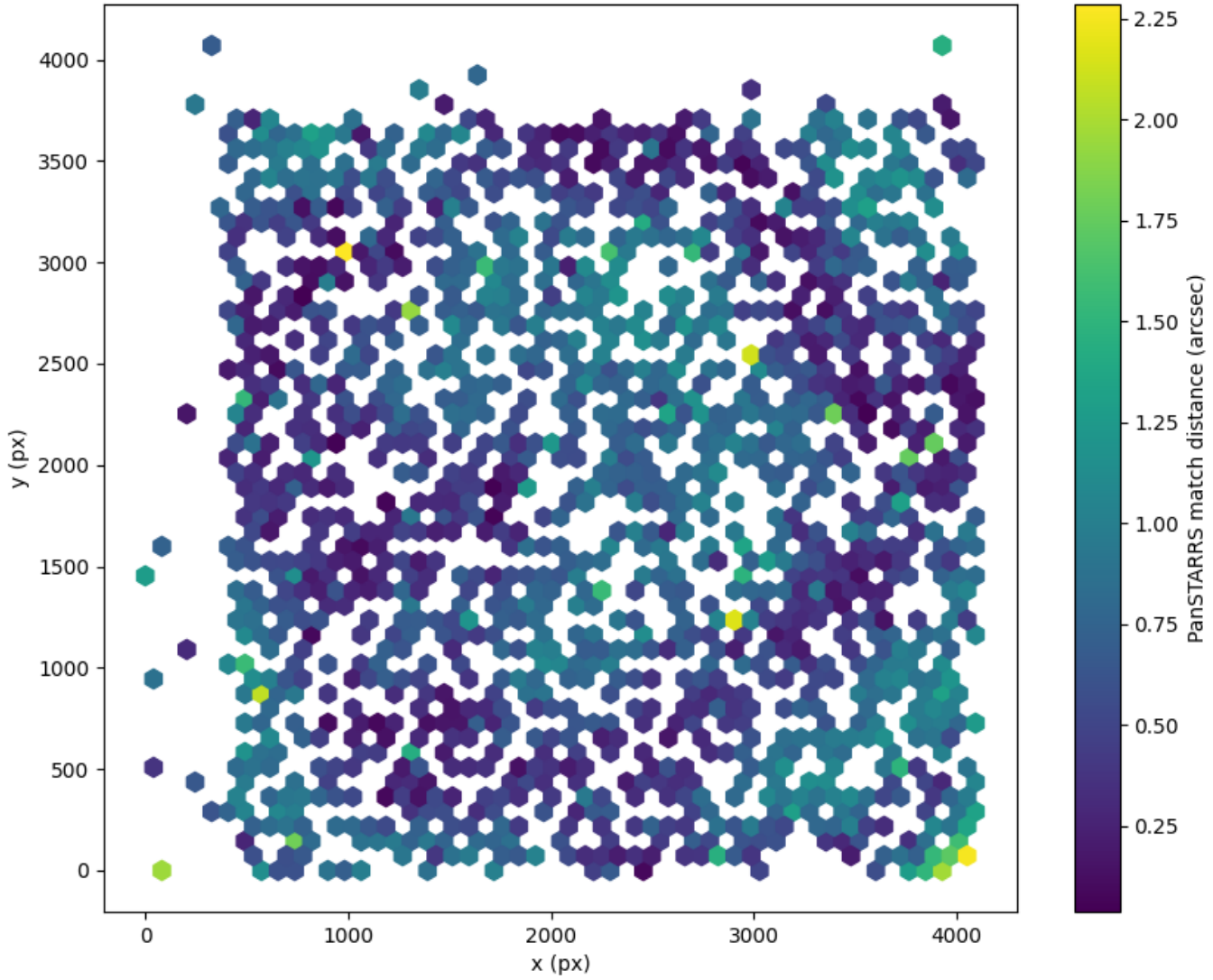
Field 2895 2D field distribution of catalog-matching distance (arcsec) to Pan-STARRS Hexagon length: 82px
