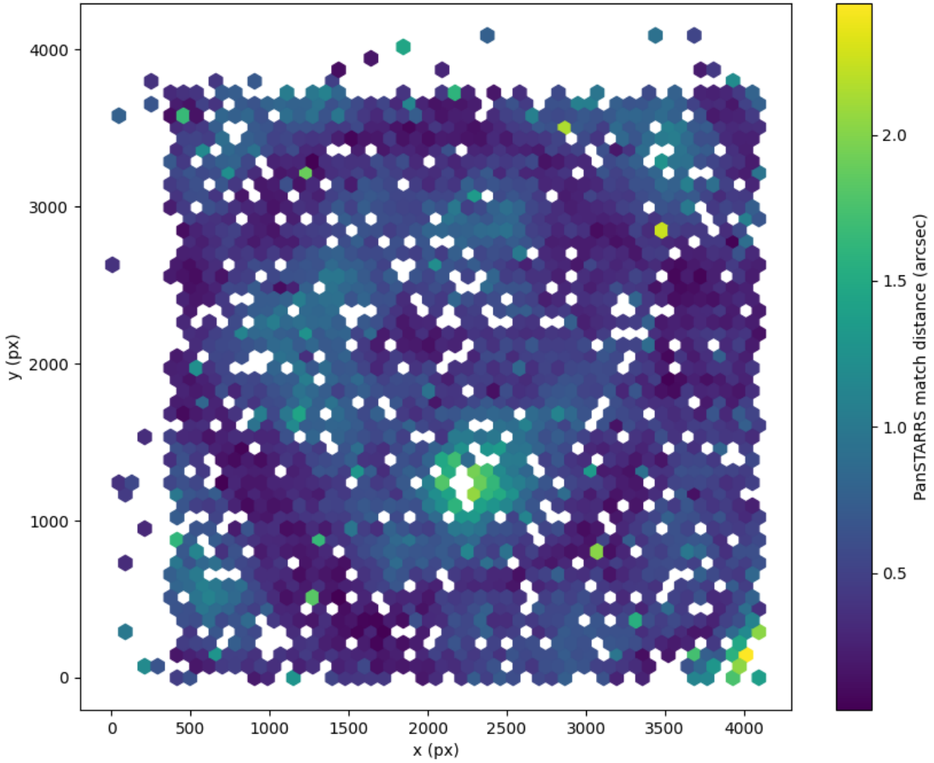
Field 2250 2D field distribution of catalog-matching distance (arcsec) to Pan-STARRS Hexagon length: 82px
