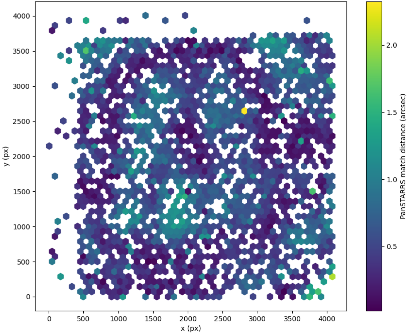
Field 2470 2D field distribution of catalog-matching distance (arcsec) to Pan-STARRS Hexagon length: 81px
