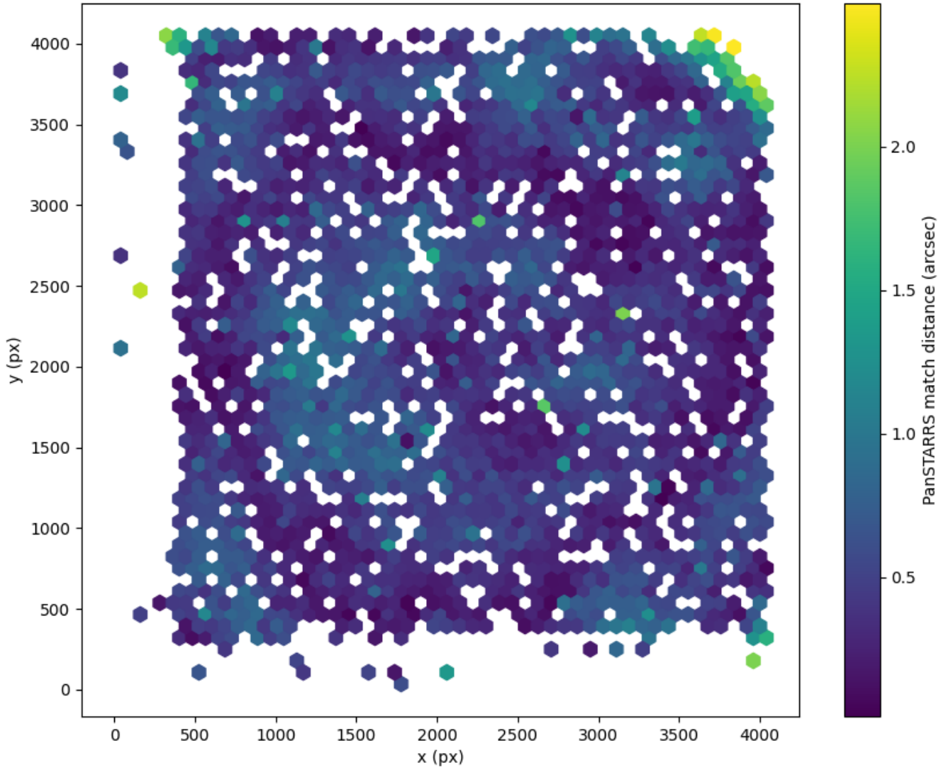
Field 0705 2D field distribution of catalog-matching distance (arcsec) to Pan-STARRS Hexagon length: 81px
