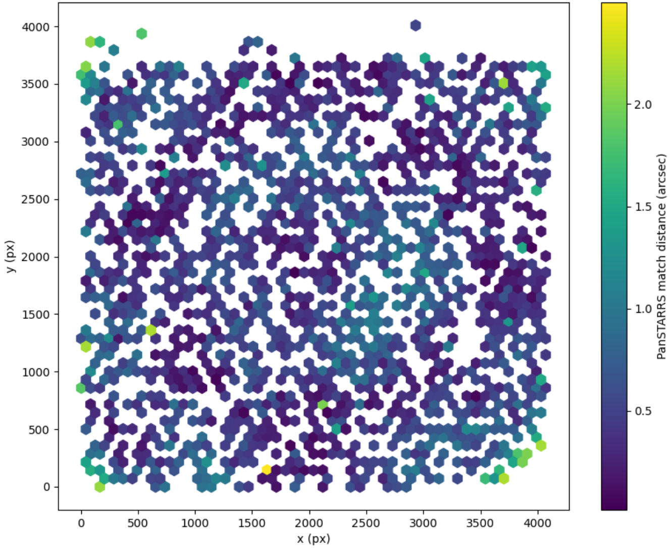
Field 2892 2D field distribution of catalog-matching distance (arcsec) to Pan-STARRS Hexagon length: 81px
