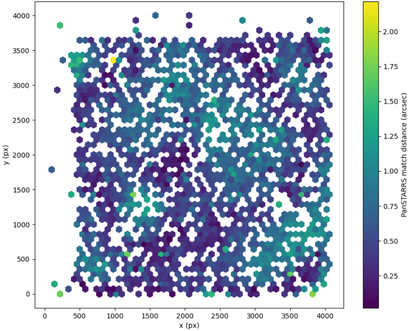
Field 2794 2D field distribution of catalog-matching distance (arcsec) to Pan-STARRS Hexagon length: 80px
