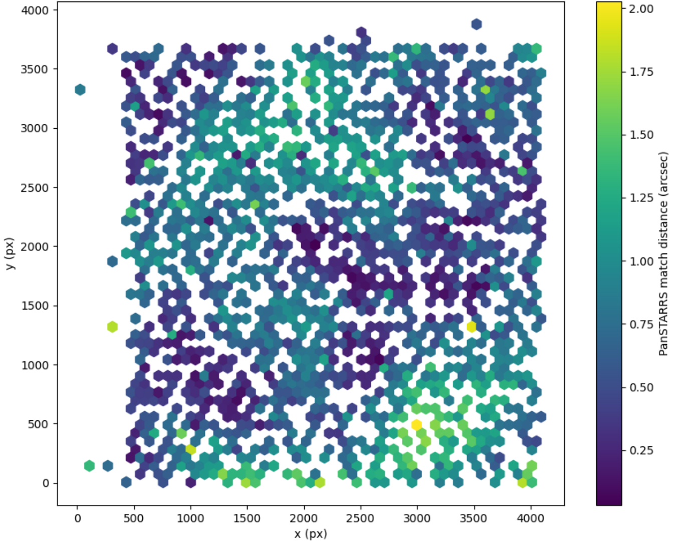
Field 2685 2D field distribution of catalog-matching distance (arcsec) to Pan-STARRS Hexagon length: 81px
