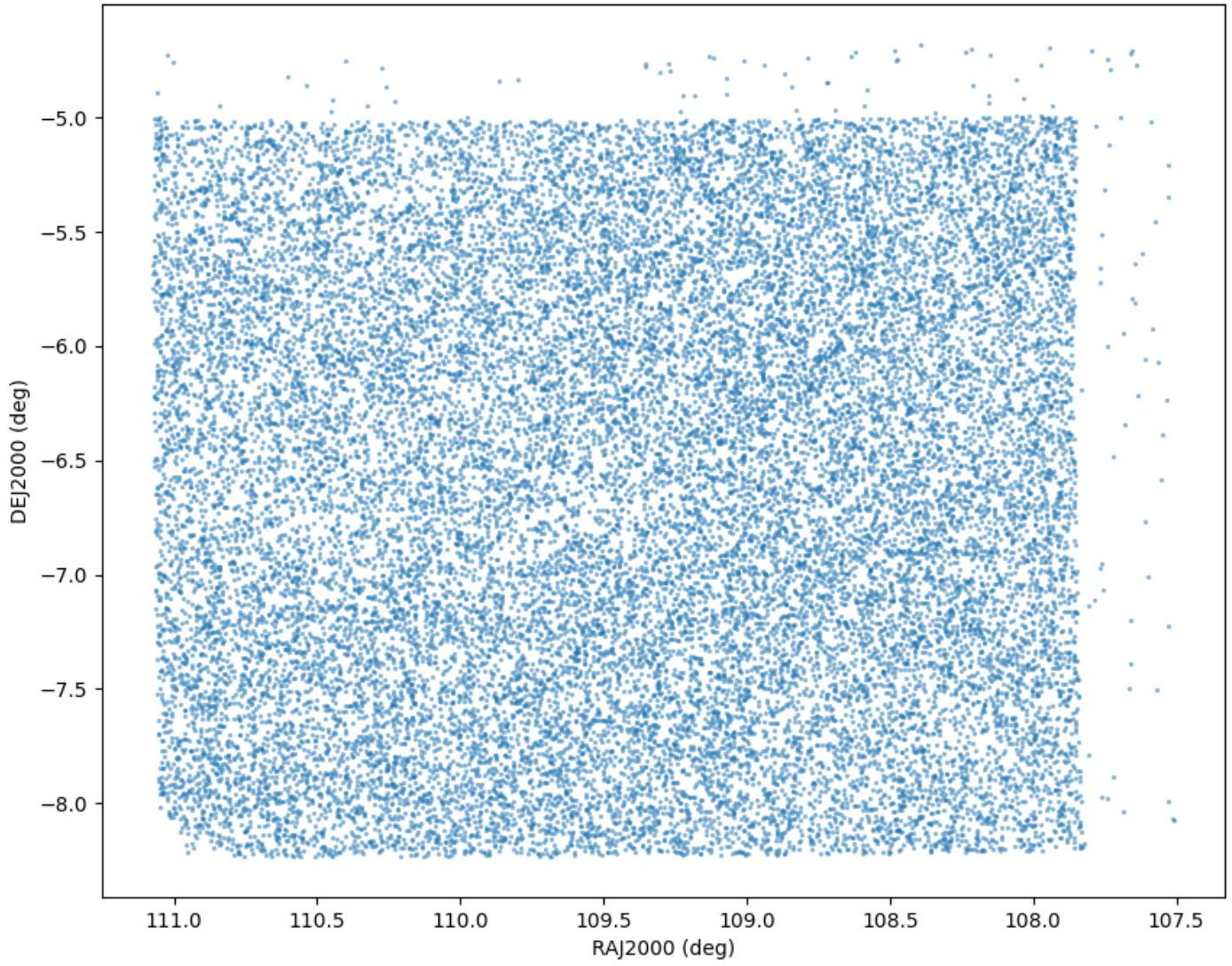
Field 2261 Catalog field coverage
