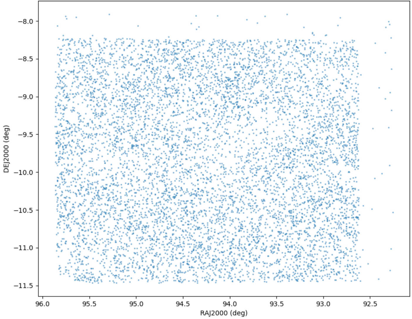
Field 2368 Catalog field coverage
