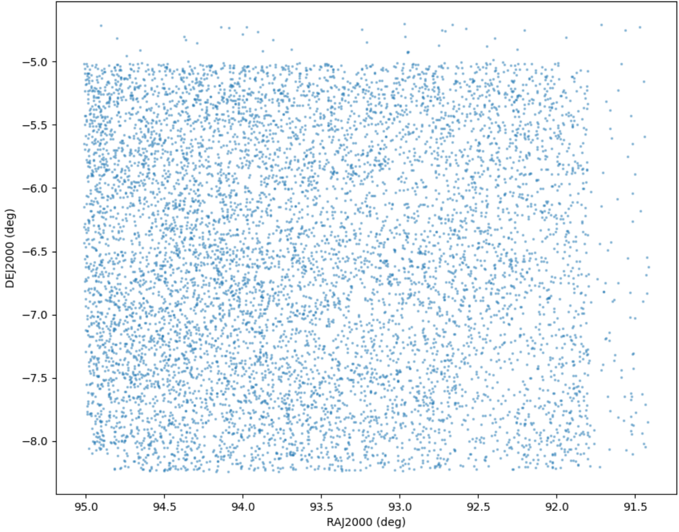
Field 2256 Catalog field coverage
