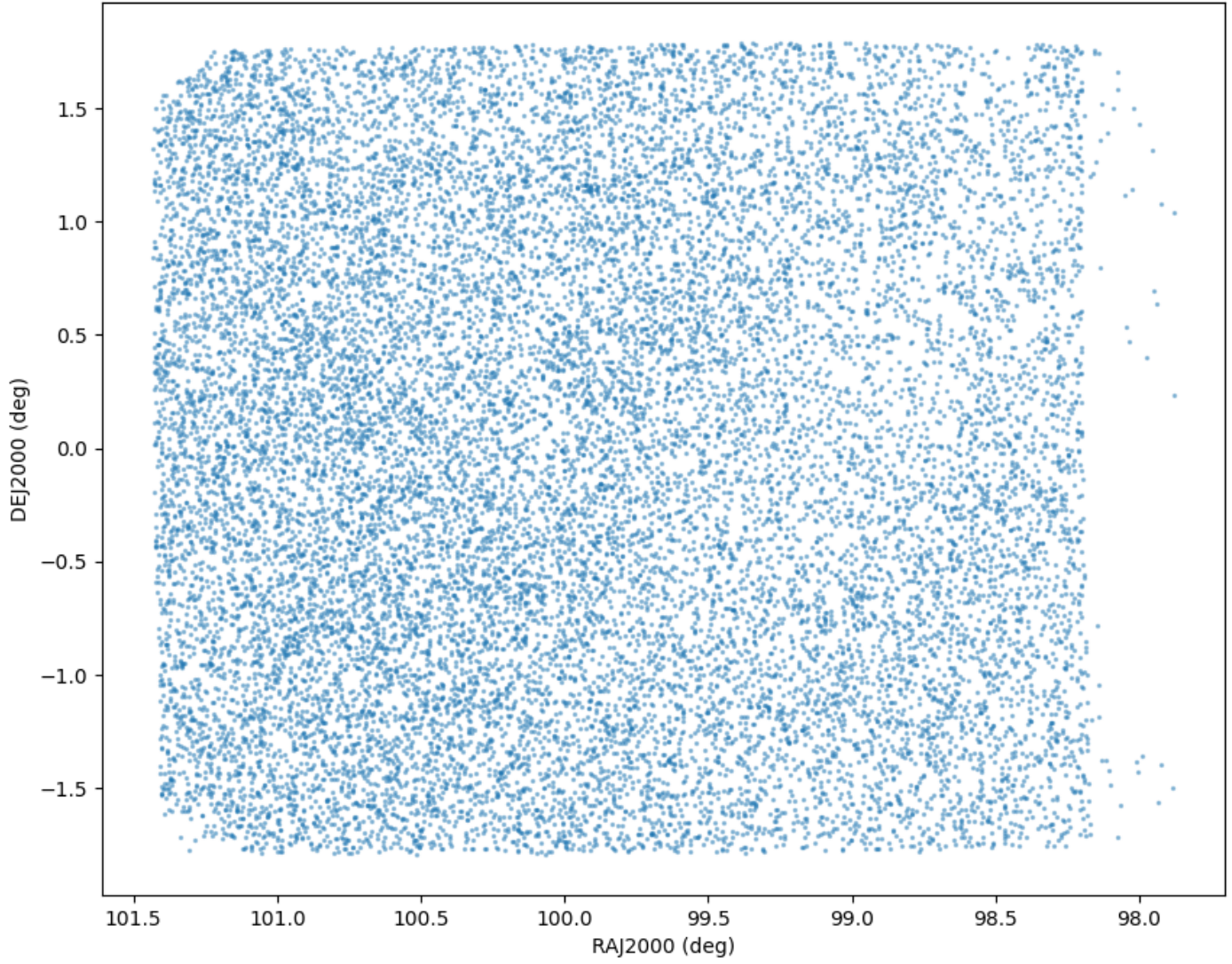
Field 0032 Catalog field coverage
