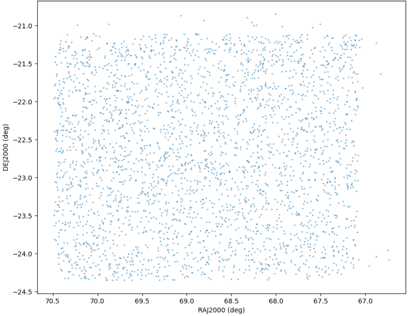
Field 2796 Catalog field coverage
