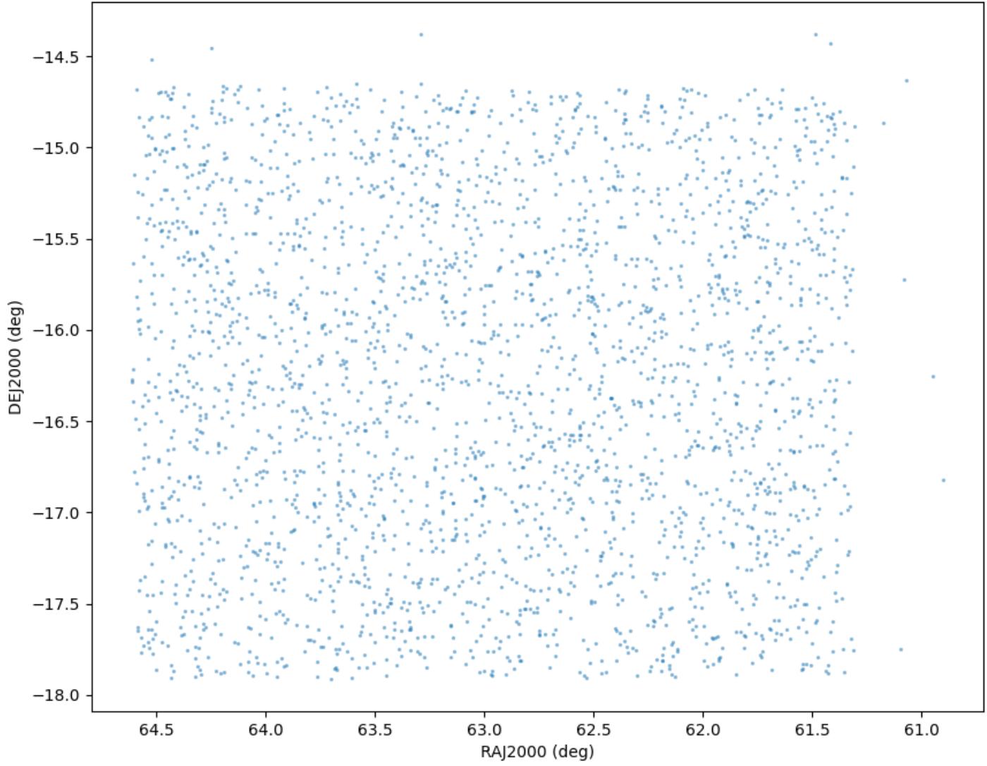
Field 2579 Catalog field coverage
