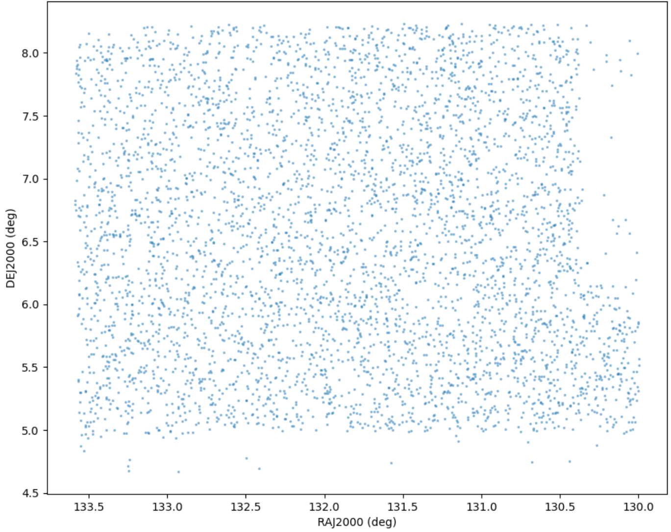
Field 0266 Catalog field coverage
