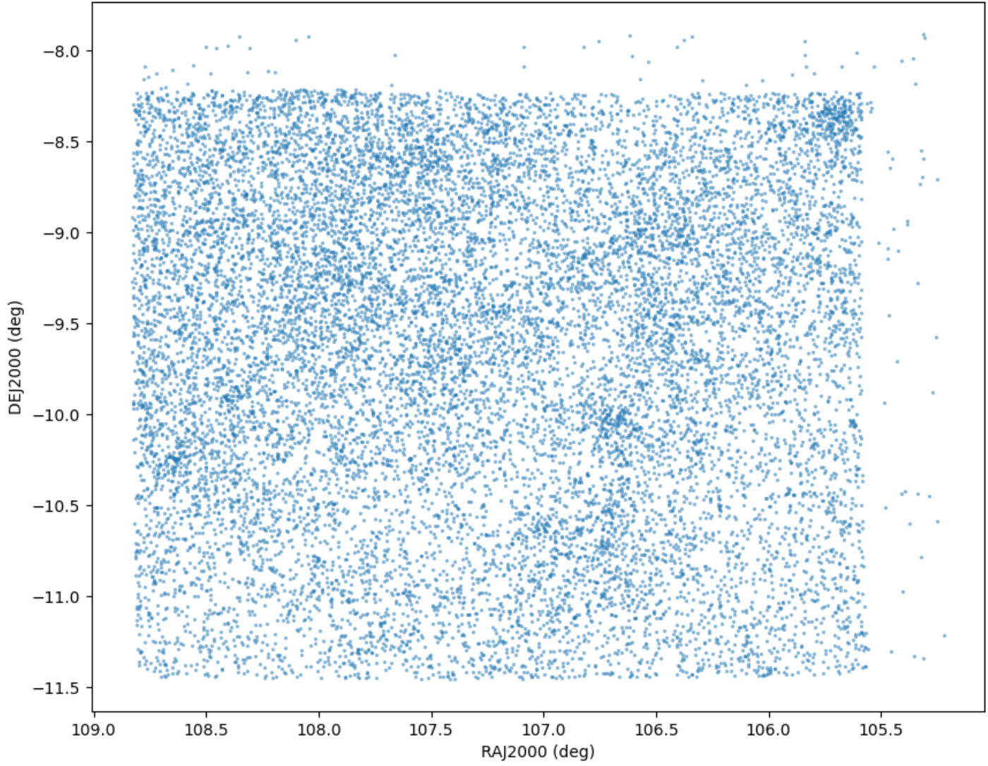
Field 2372 Catalog field coverage
