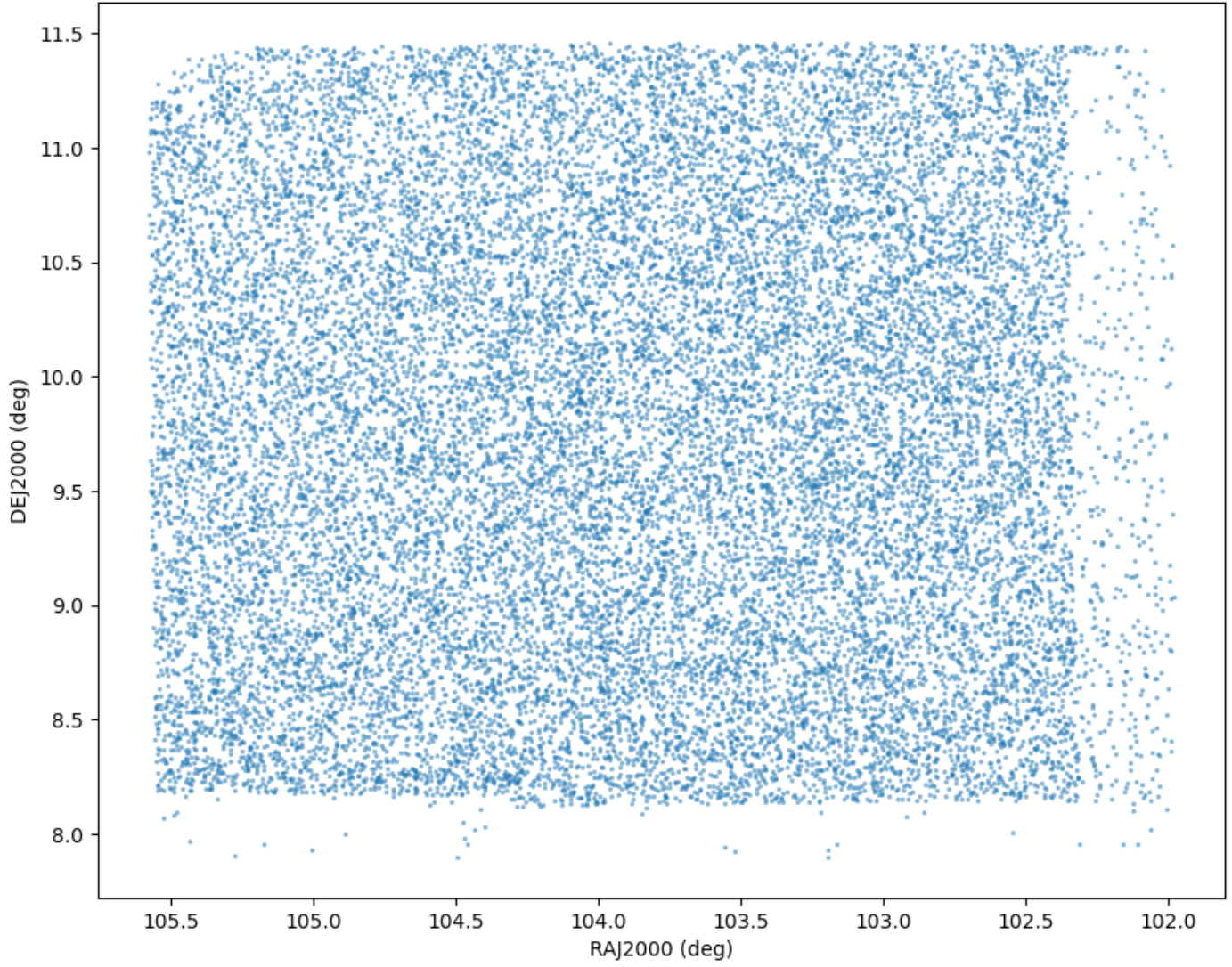
Field 0369 Catalog field coverage
