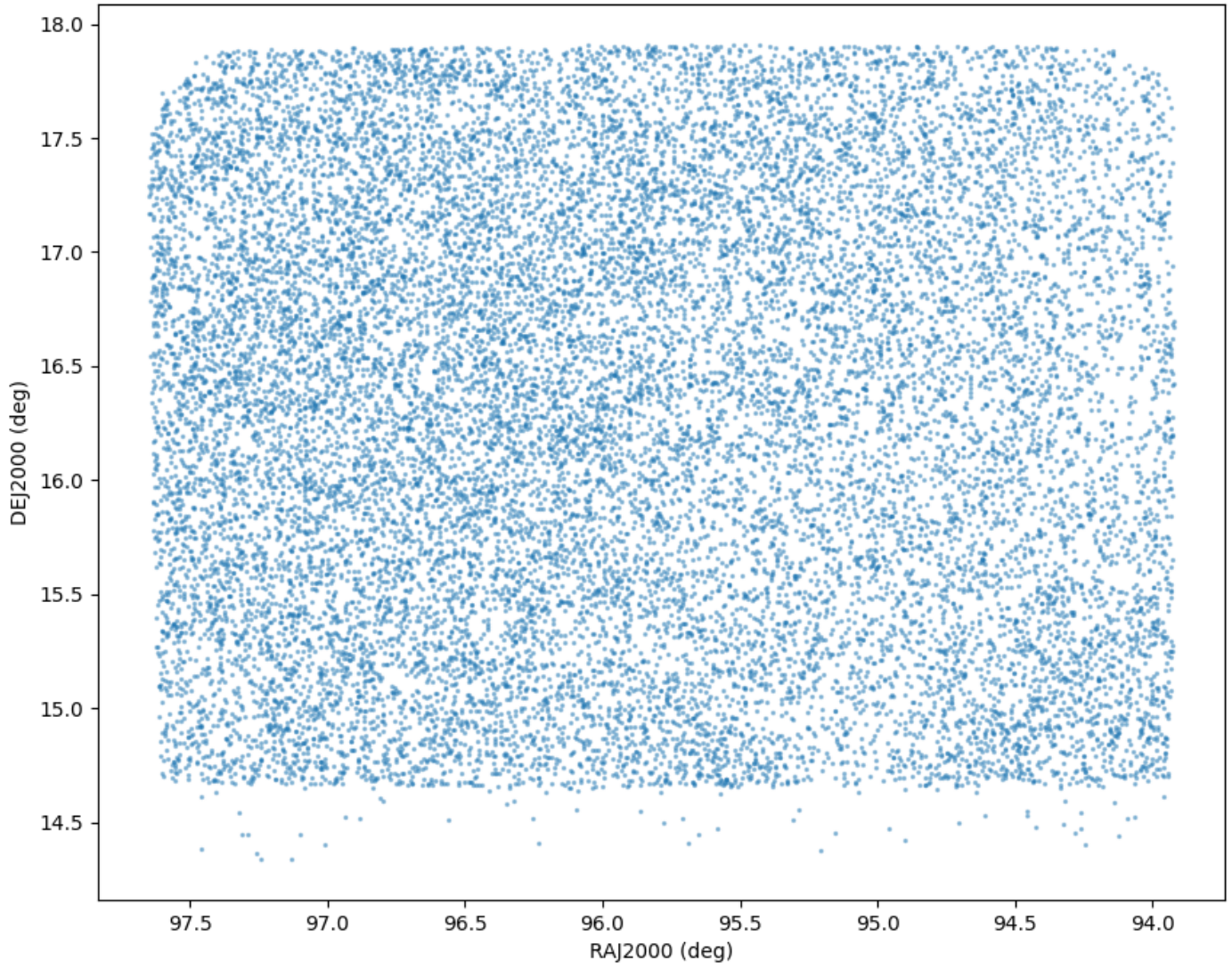
Field 0587 Catalog field coverage
