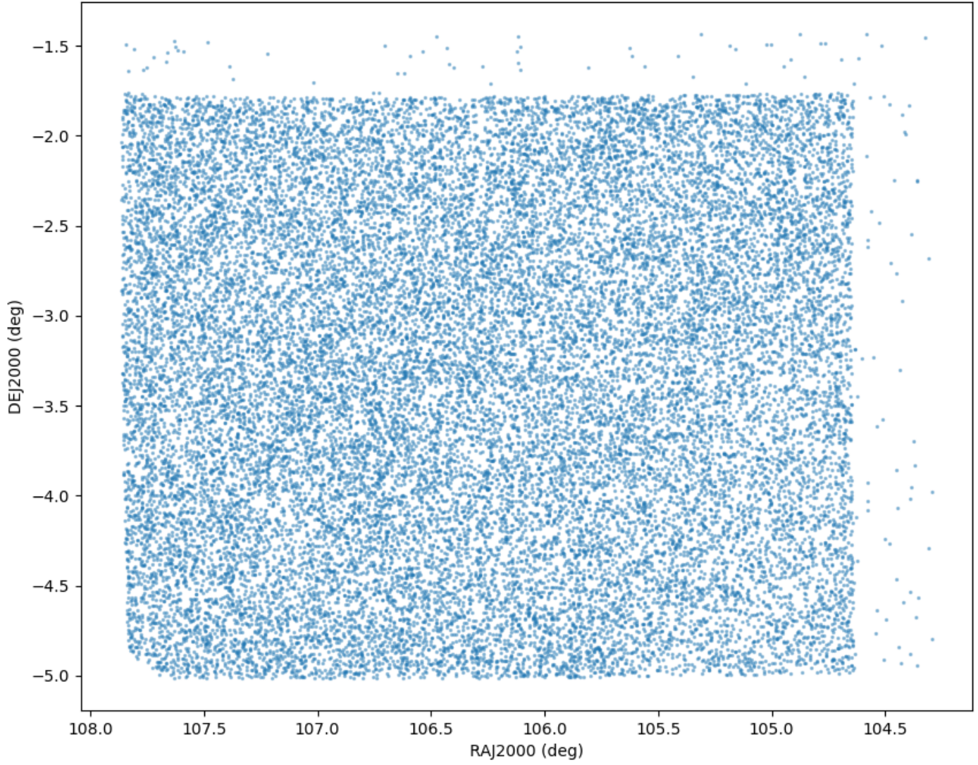
Field 2148 Catalog field coverage
