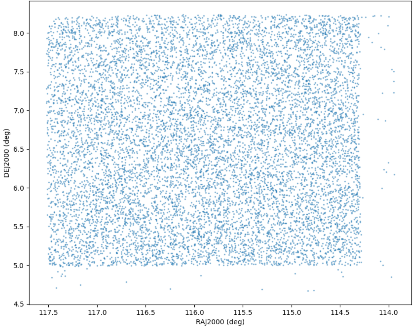
Field 0261 Catalog field coverage
