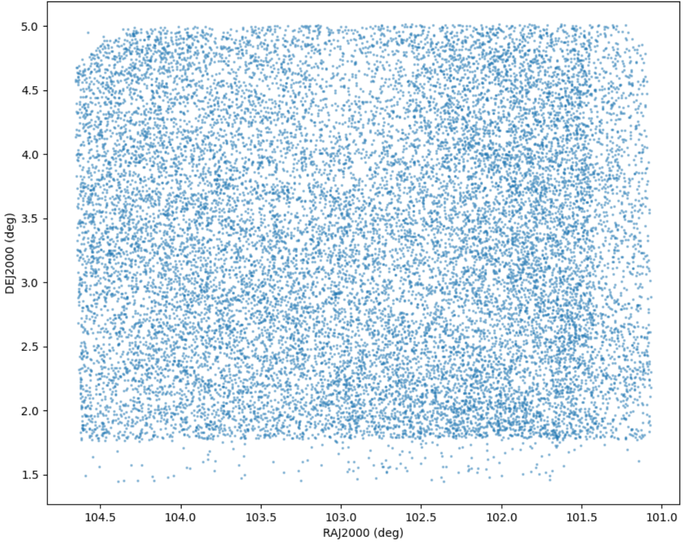
Field 0145 Catalog field coverage
