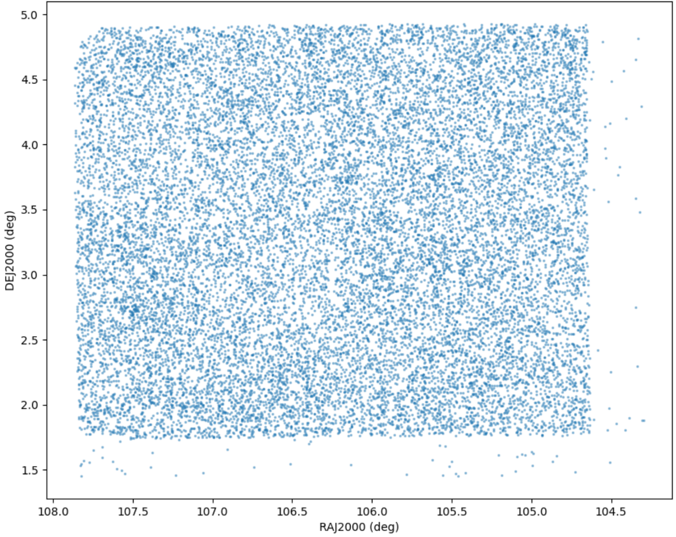
Field 0146 Catalog field coverage
