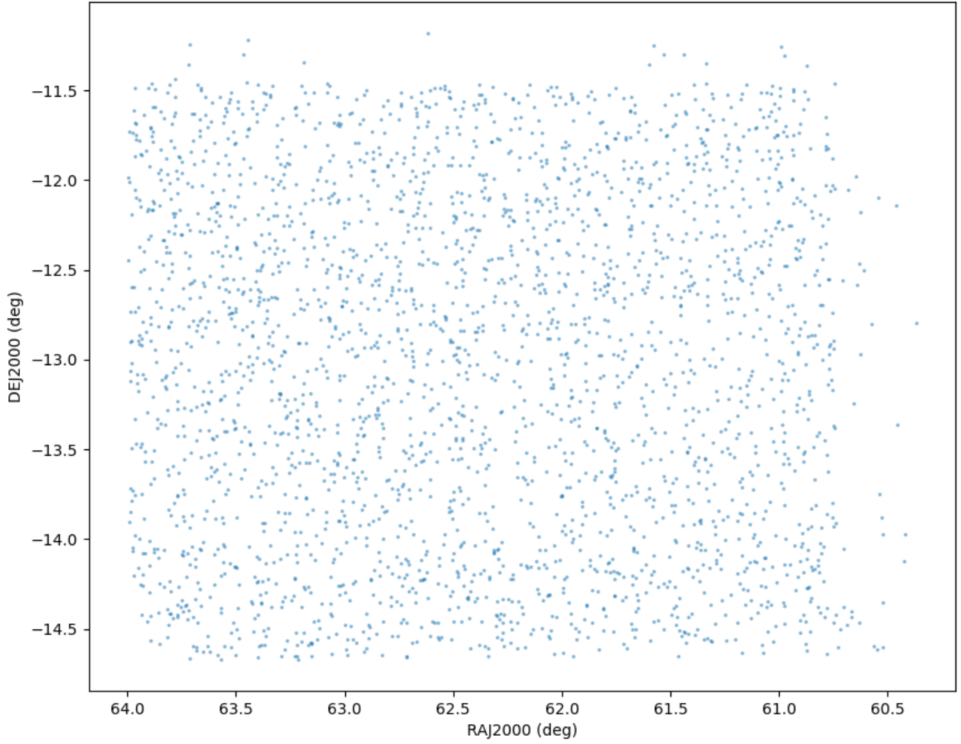
Field 2469 Catalog field coverage
